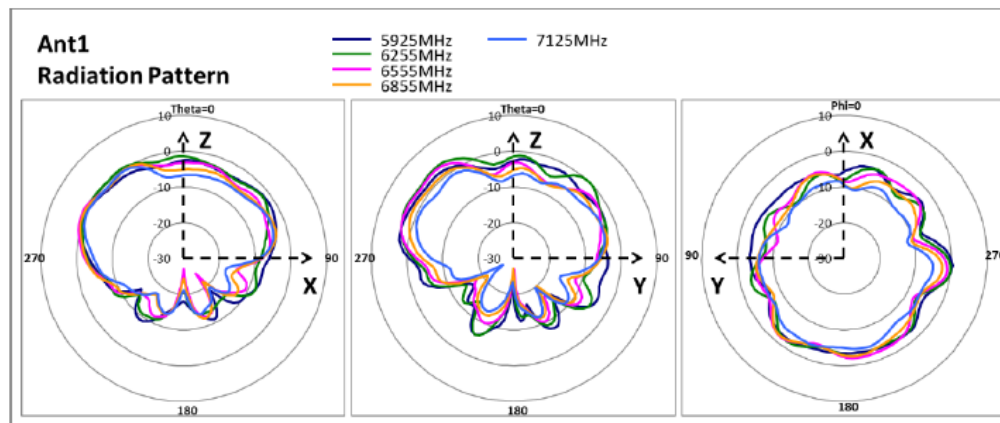
ANTENNA 1 (6GHz)
