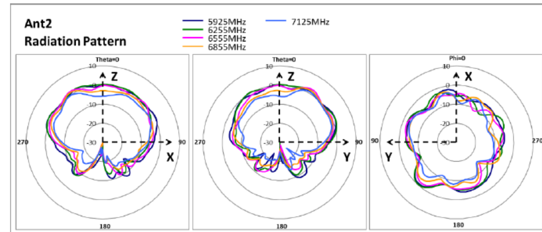
ANTENNA 2 (6GHz)
