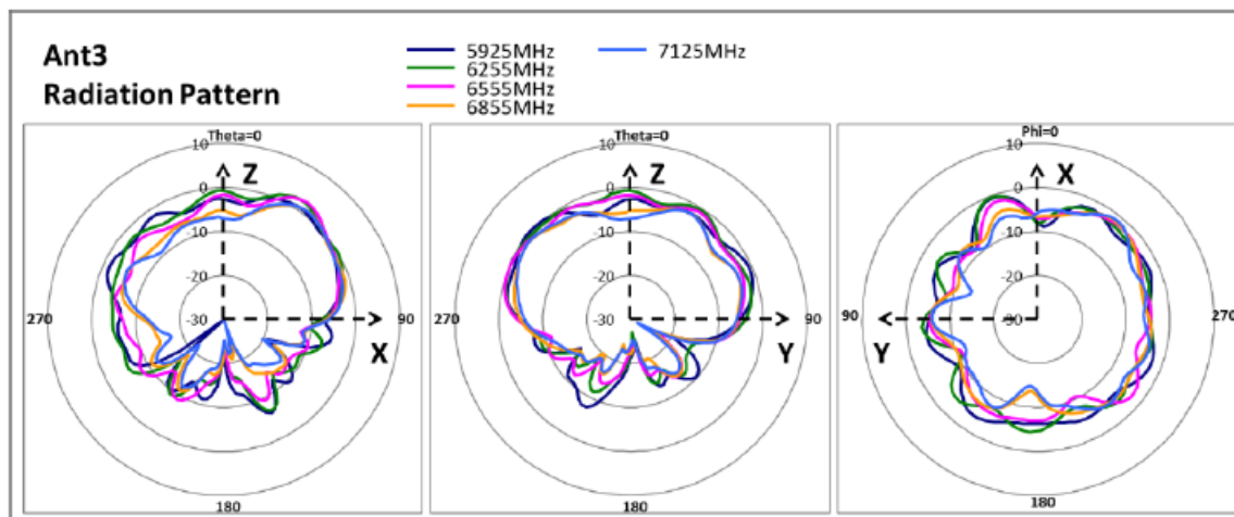
ANTENNA 3 (6GHz)
