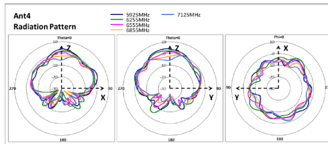
ANTENNA 4 (6GHz)
