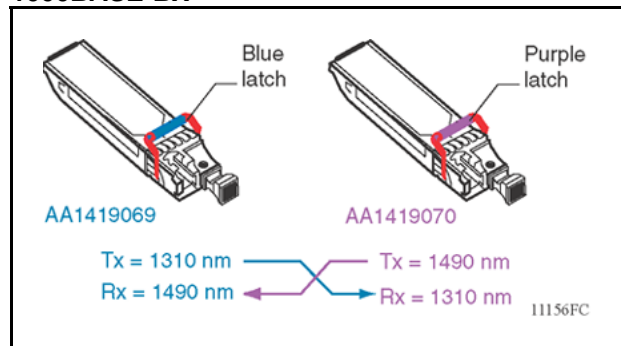
Figure 2 1000BASE-BX
