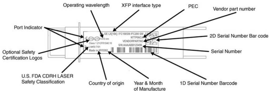
Figure 5: XFP label
