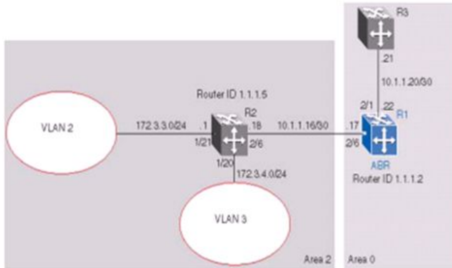
Figure 27: ABR configuration example
