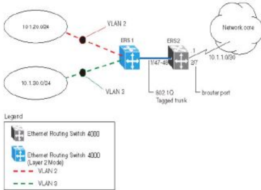
Figure 33: RIP configuration example
