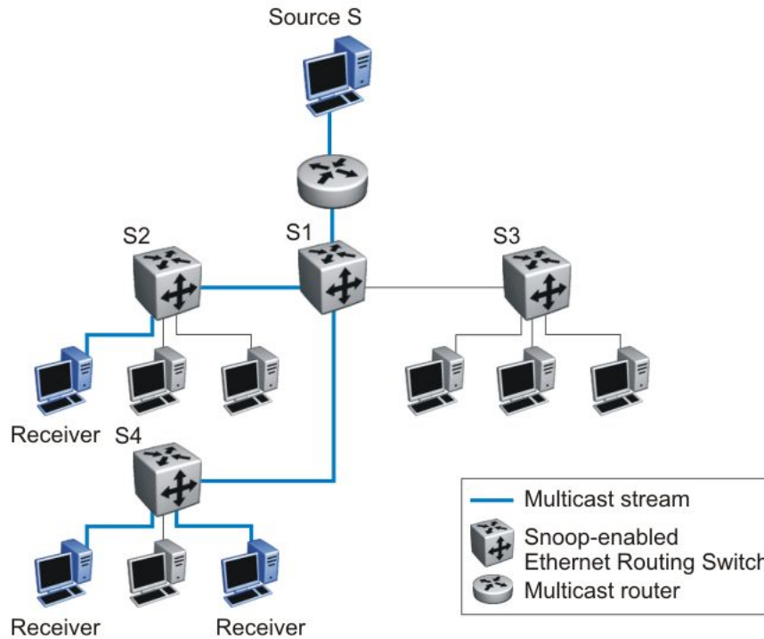
Figure 20: Ethernet Routing Switch running IGMP snooping
