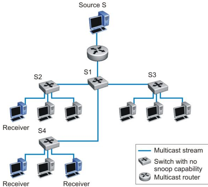
Figure 19: IP multicast propagation on a LAN without IGMP snooping
