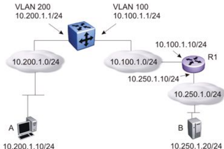
Figure 3: Static routes
