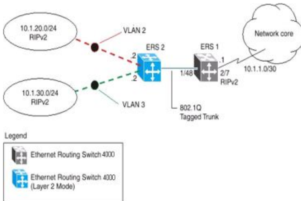
Figure 34: RIPv2 configuration example
