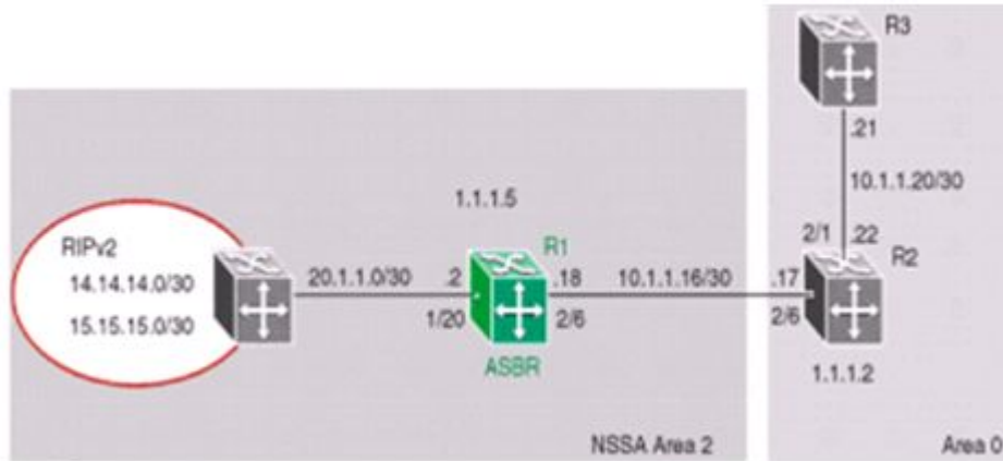
Figure 30: NSSA configuration example
