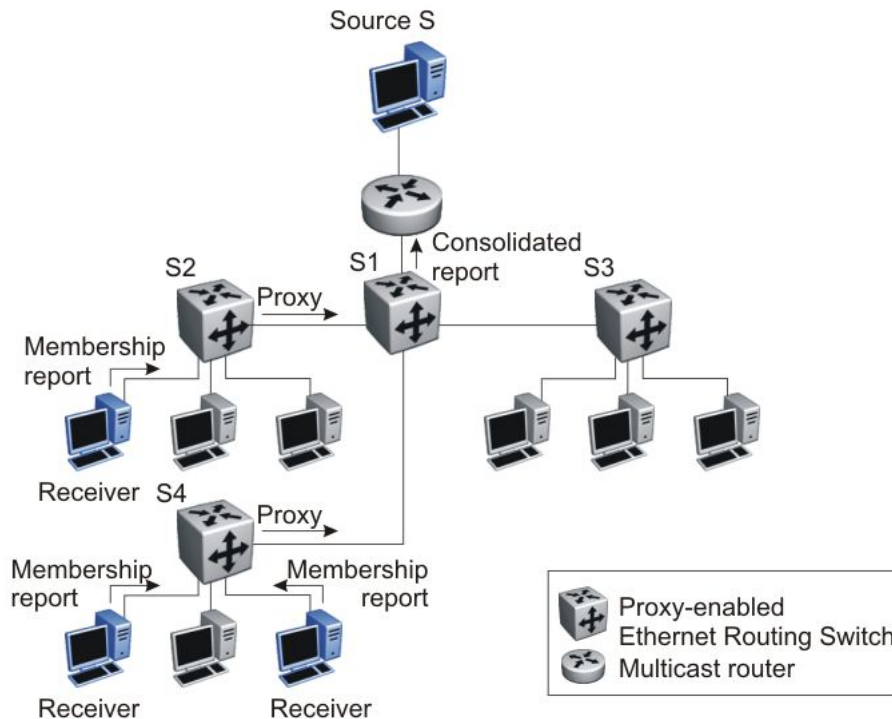
Figure 21: Ethernet Routing Switch running IGMP proxy
