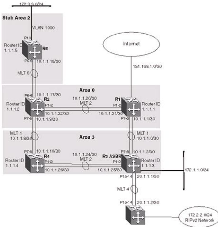
Figure 32: Multi-area complex example
