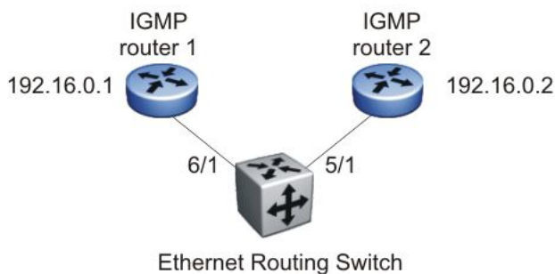
Figure 22: Static mrouter port and nonquerier
