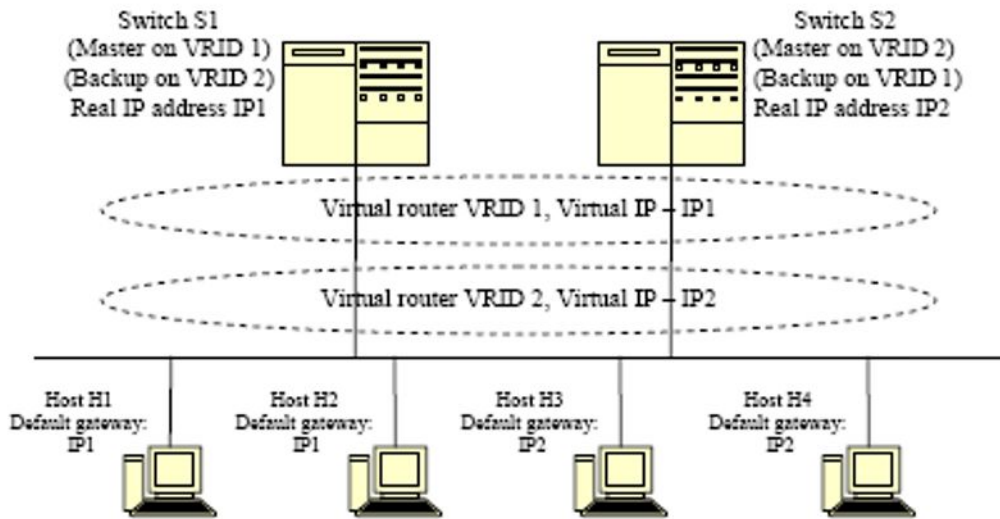
Figure 37: Example VRRP topology 2
