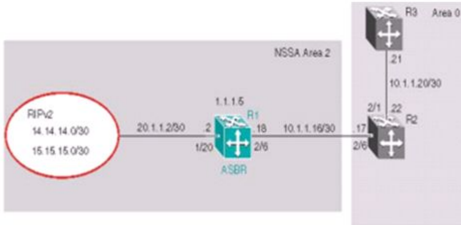
Figure 31: External route advertisement example
