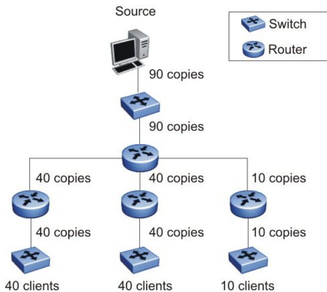
Figure 16: Wasteful propagation of multiple copies of the same unicast stream
