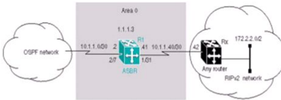
Figure 28: ASBR distribution example
