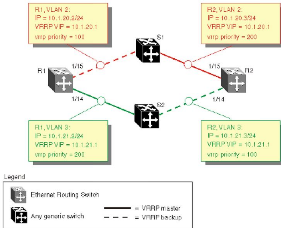
Figure 36: Example VRRP topology 1
