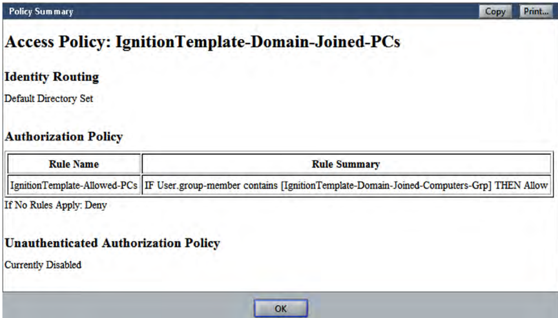
Figure 3: Access Policy Summary page- Ignition Template-Domain-Joined-PCs example
