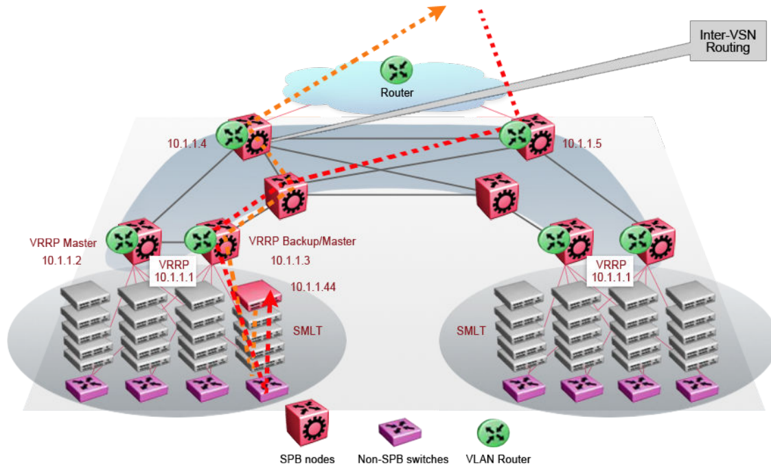
Figure 70: Optimized routing before moving VMs
