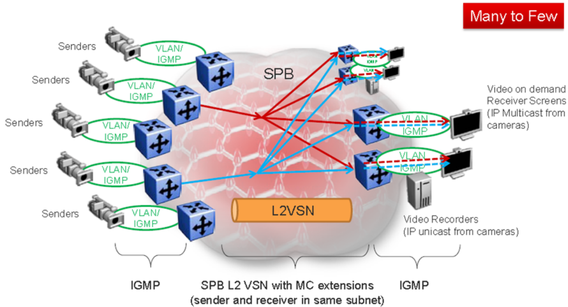
Figure 74: Deployment scenario — bridged video surveillance and IP camera deployment for transportation, airports, and government
