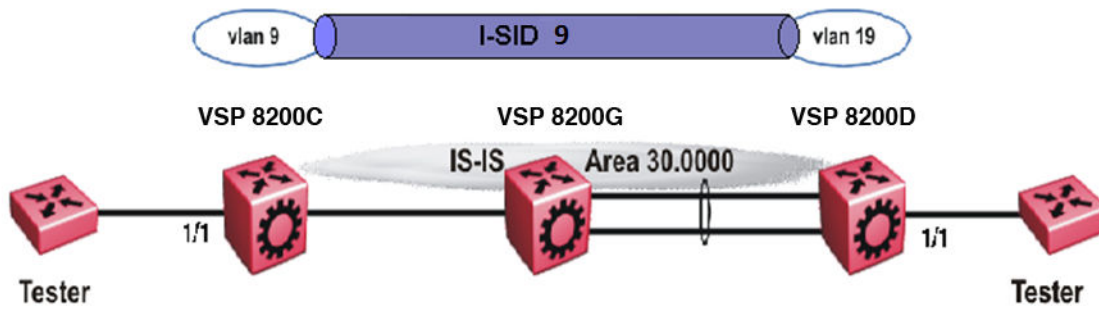
Figure 47: Layer 2 VSN with different VLAN IDs
