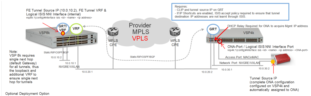
Figure 31: FE over VPLS traffic flow
