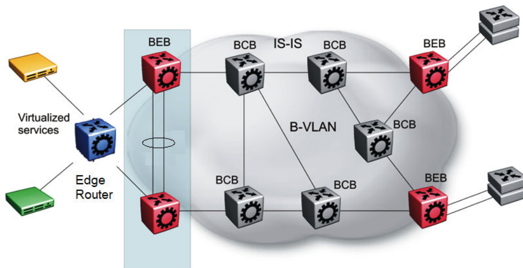
Figure 62: SPBM basic architecture
