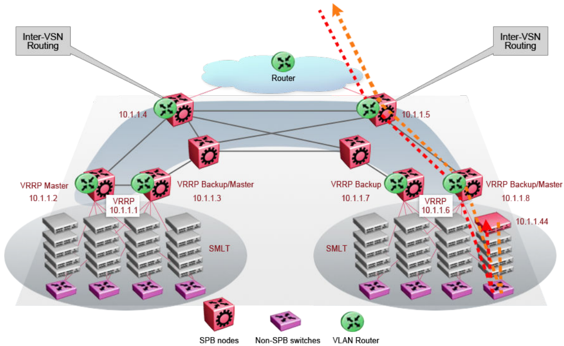
Figure 71: Optimized routing after moving VMs
