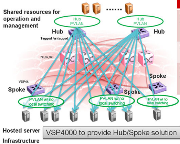
Figure 73: Data center hosting private VLAN
