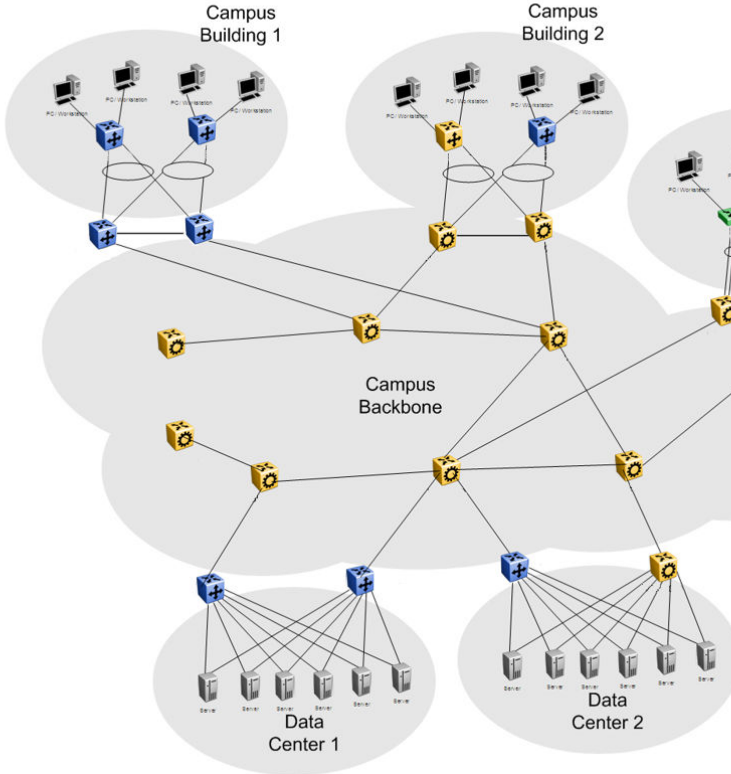
Figure 49: SPBM IP shortcuts in a campus
