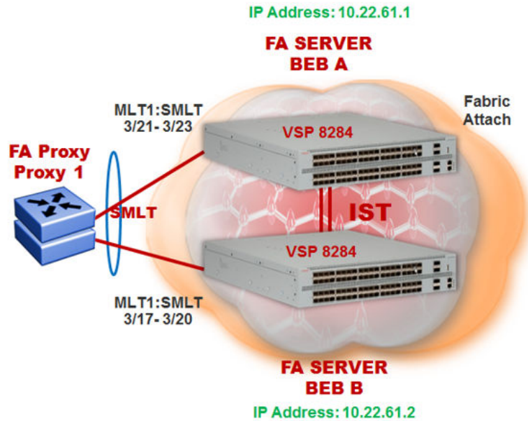
Figure 37: FA configuration in dual-homed SMLT
