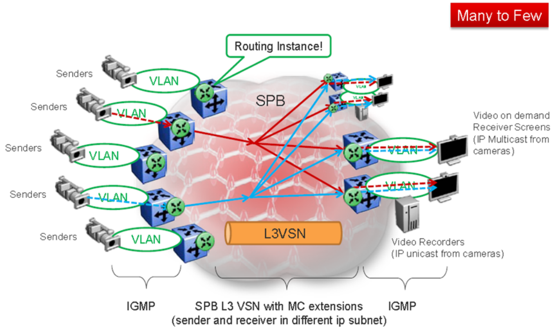
Figure 75: Deployment scenario — Routed video surveillance and IP camera deployment for transportation, airports, and government
