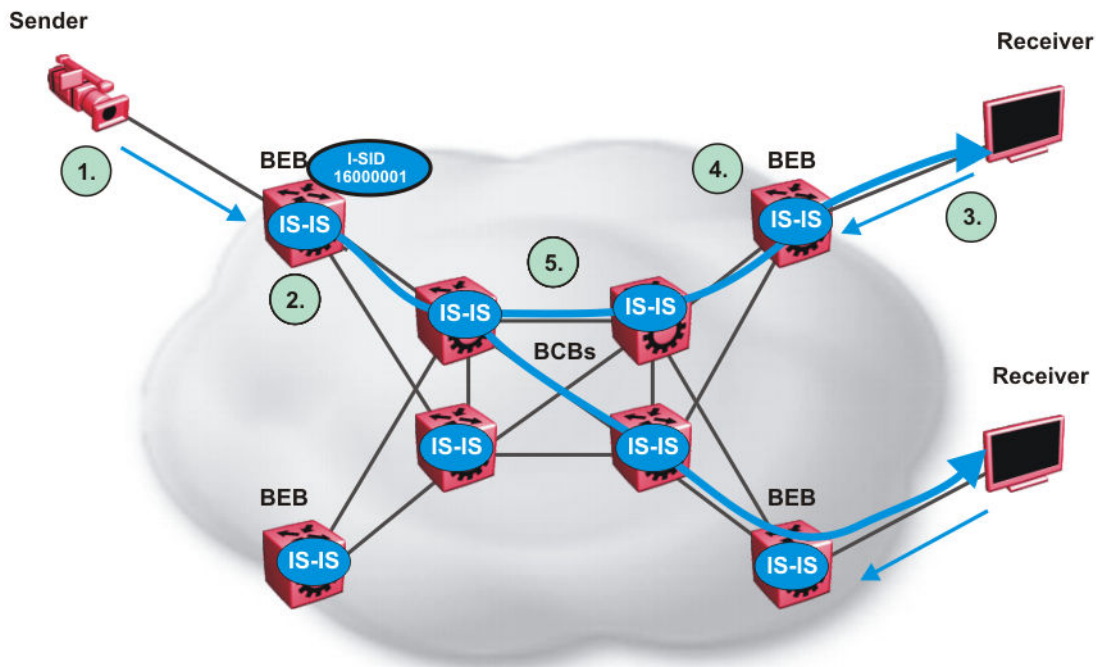
Figure 5: IP Multicast over Fabric Connect streams
