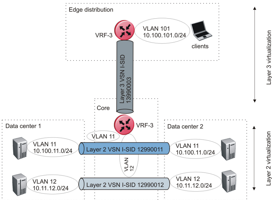
Figure 66: VRF scenario to move traffic between data centers
