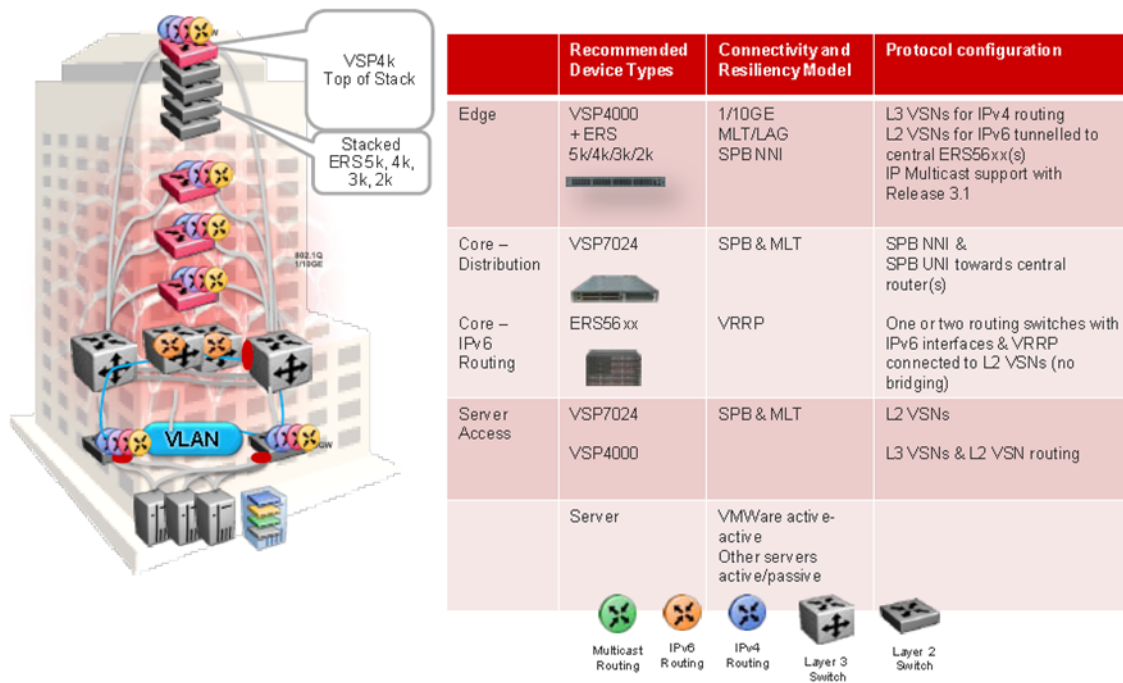
Figure 72: Small core — multi-tenant
