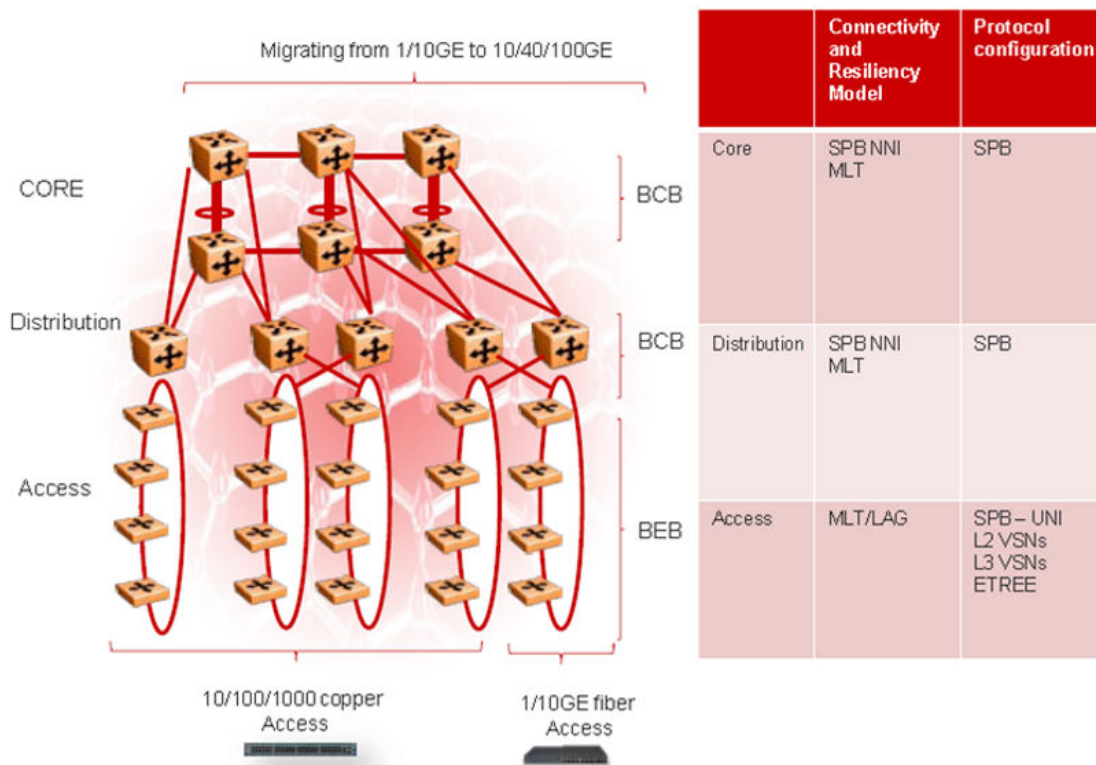
Figure 76: Metro ring access solution
