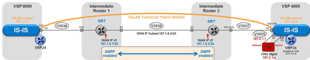
Figure 32: FE over VPLS traffic flow component view
