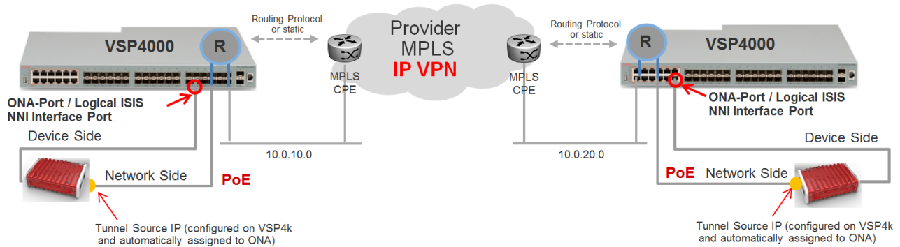
Figure 35: Fabric Extend traffic flow
