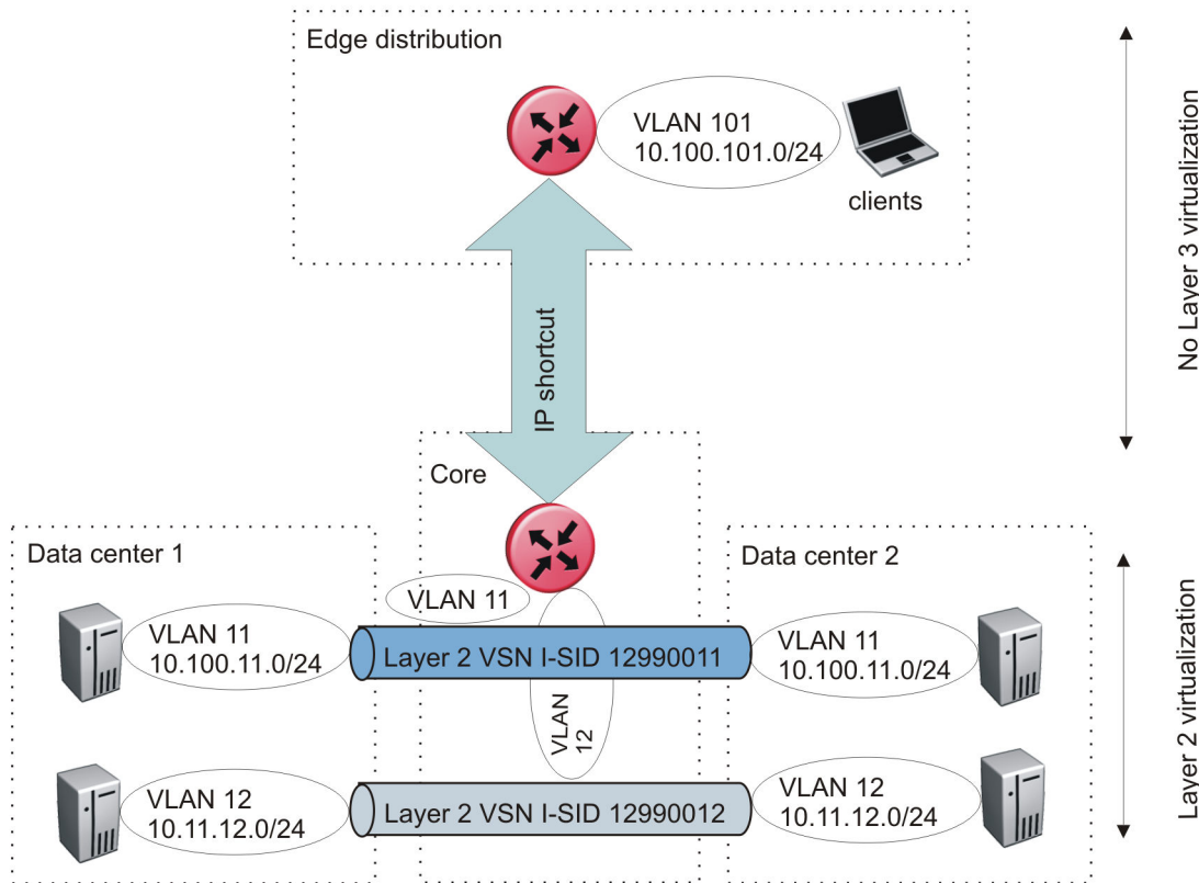
Figure 65: IP shortcut scenario to move traffic between data centers
