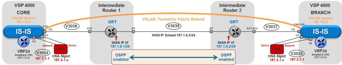
Figure 36: Fabric Extend traffic flow component view
