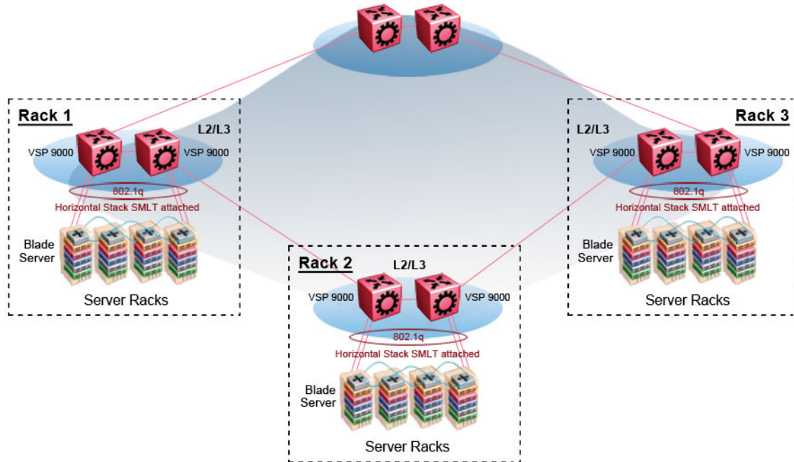
Figure 2: SPBM ring topology with shared data centers
