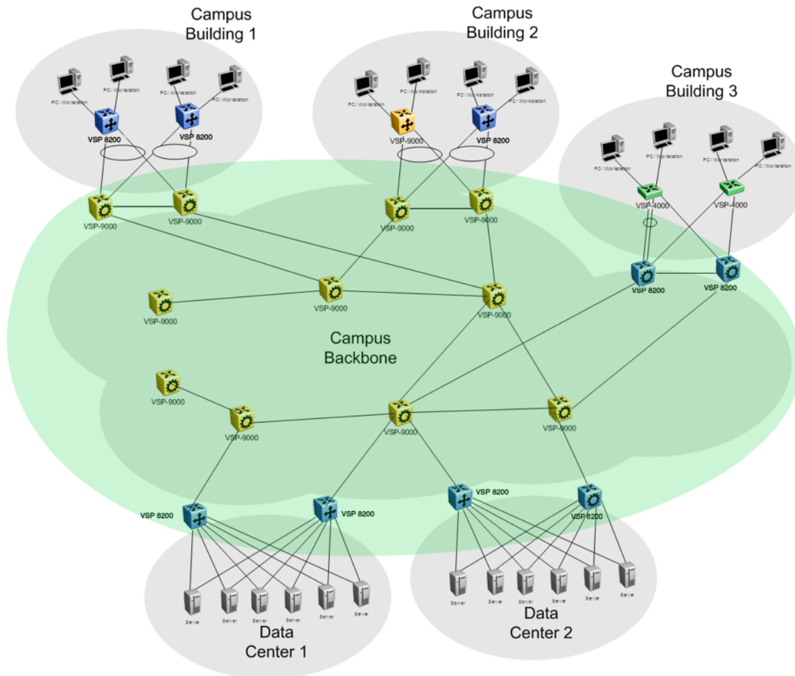
Figure 39: SPBM L2 VSN in a campus
