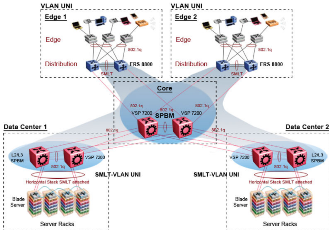
Figure 64: SPBM campus without SMLT
