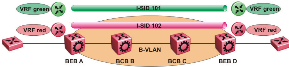
Figure 51: SPBM Layer 3 VSN
