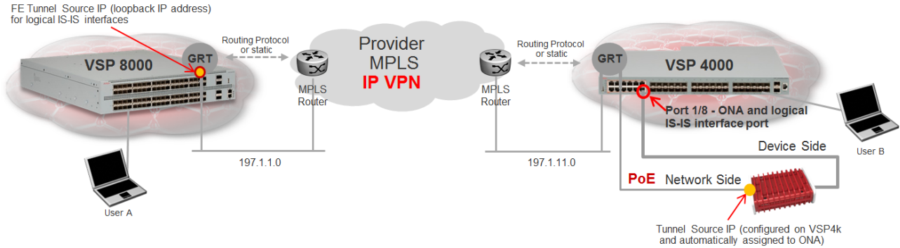
Figure 27: IP using GRT traffic flow
