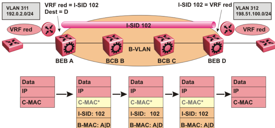
Figure 52: Packet forwarding in SPBM Layer 3 VSN
