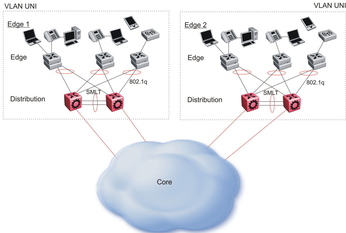
Figure 63: Access to the SPBM Core
