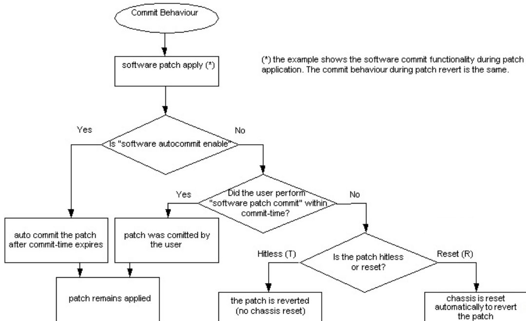
Figure 3: Committing a software patch
