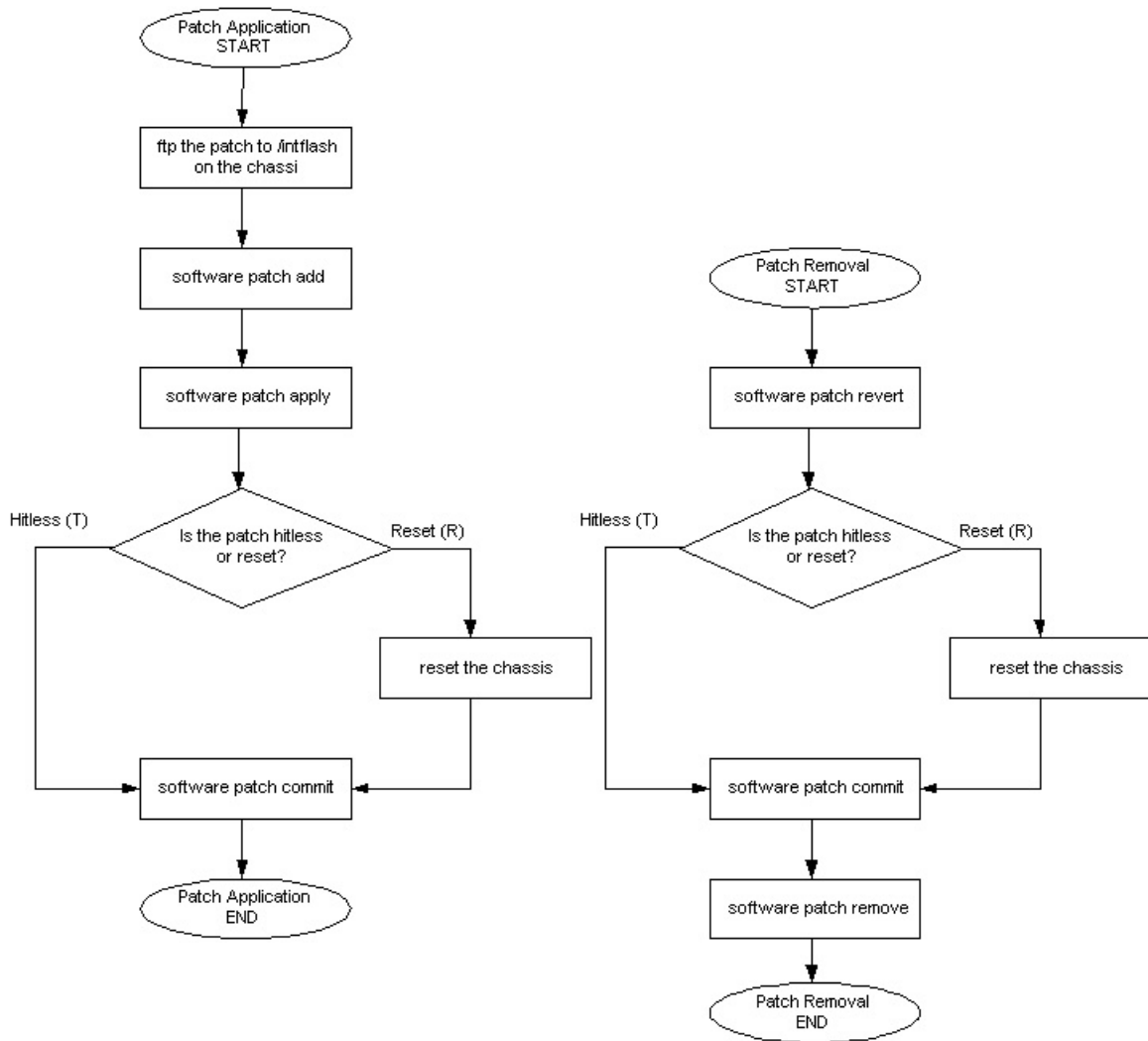
Figure 2: Patch application and removal
