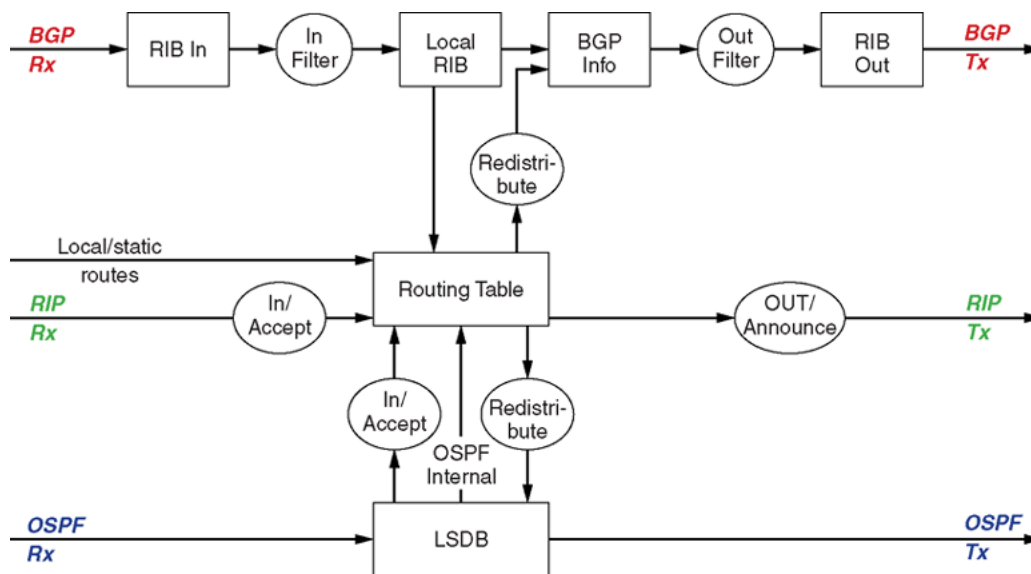
Figure 5: Route filtering for unicast routing protocols
