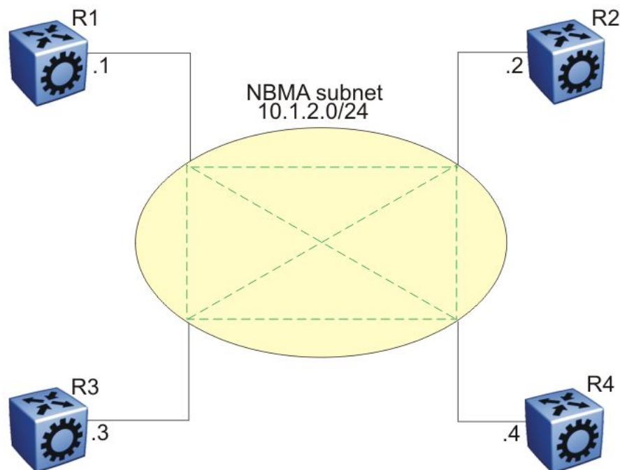
Figure 10: NBMA subnet
