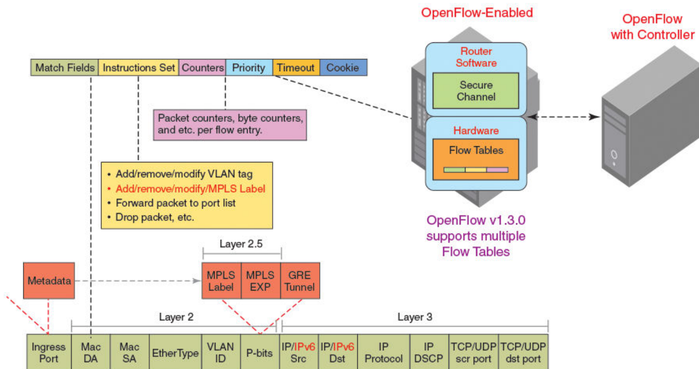
FIGURE 6 OpenFlow 1.3 flow table entries
