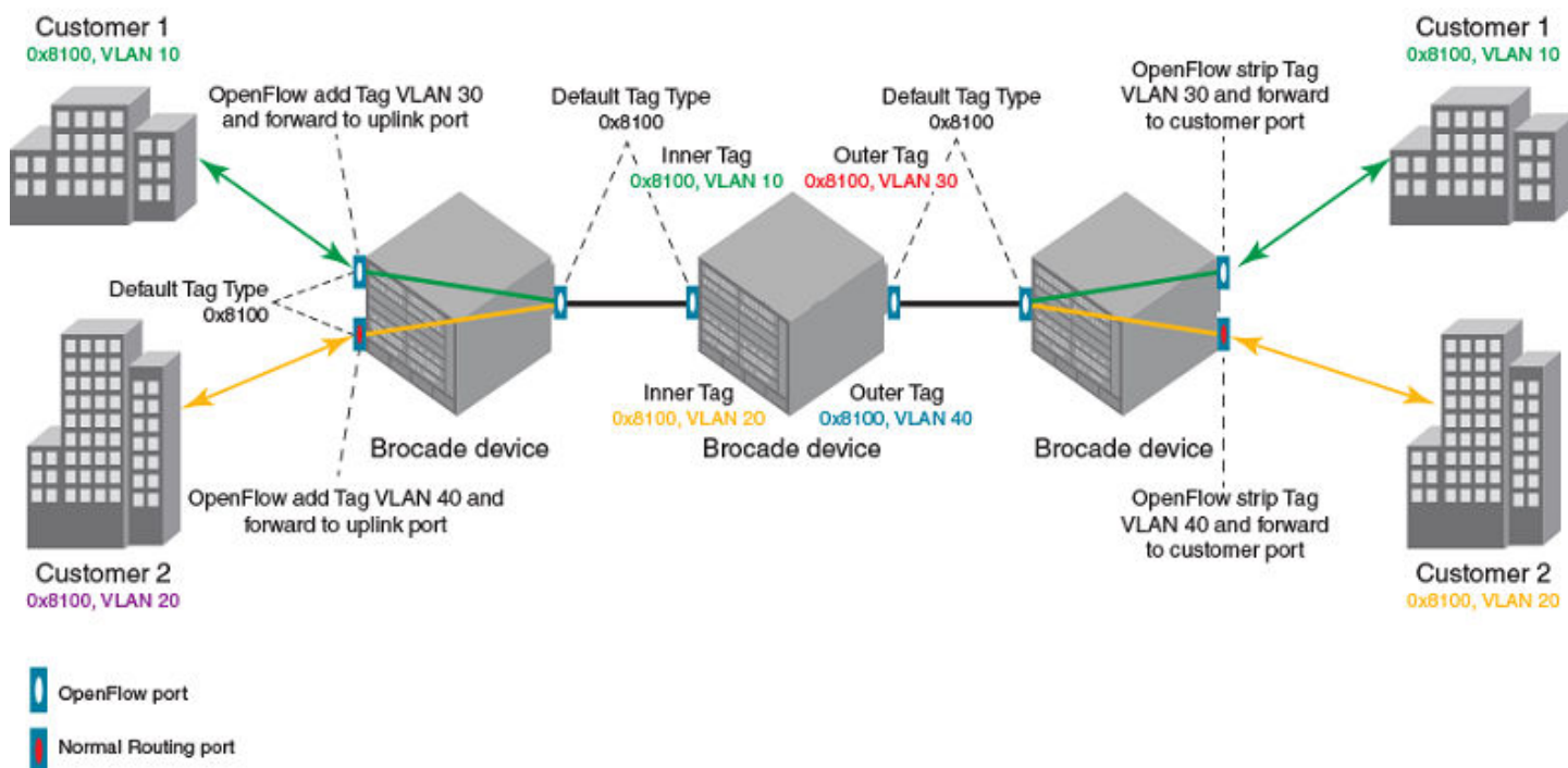
FIGURE 8 Transportation of VLAN or segment using QinQ
