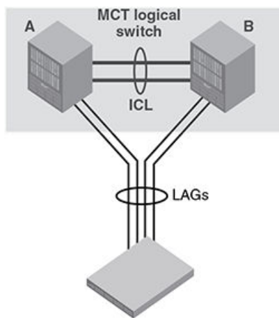
FIGURE 155 MCT peers
