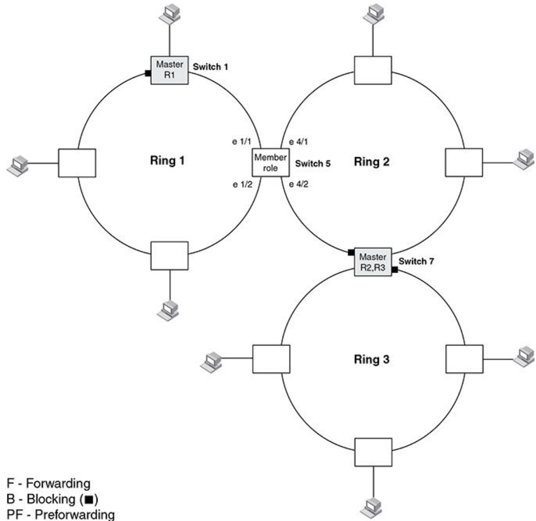
FIGURE 109 Multiple MRP rings - phase 1
