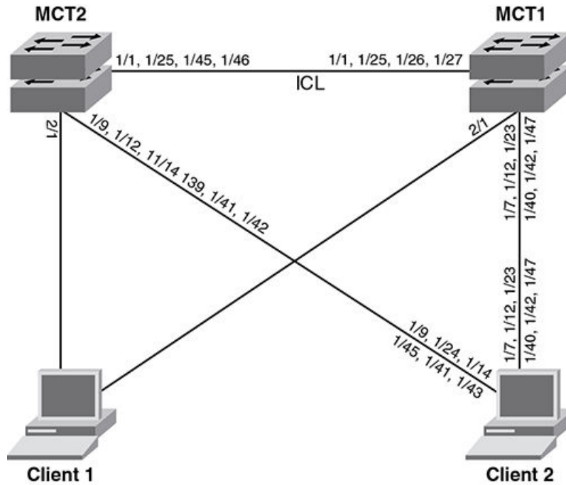
FIGURE 167 MCT snooping topology example
