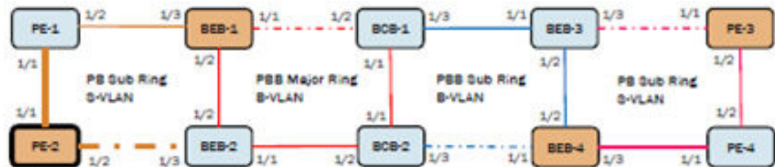
FIGURE 137 PB ring node sample configuration
