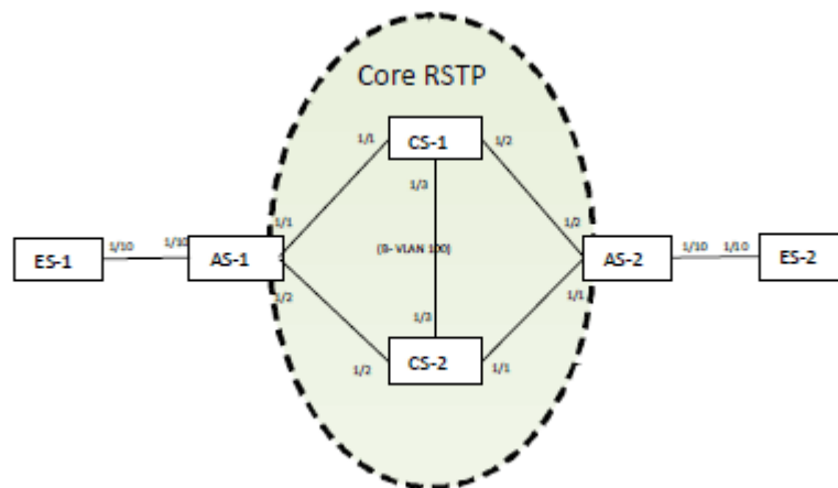
FIGURE 98 Core RSTP in PBB network
