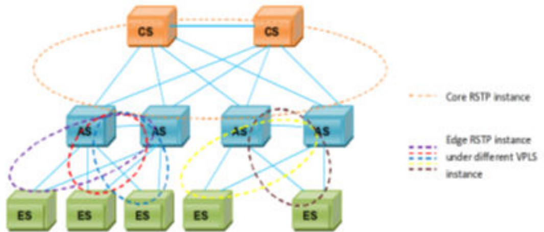
FIGURE 90 RSTP isolation in dual homing of AS and ES
