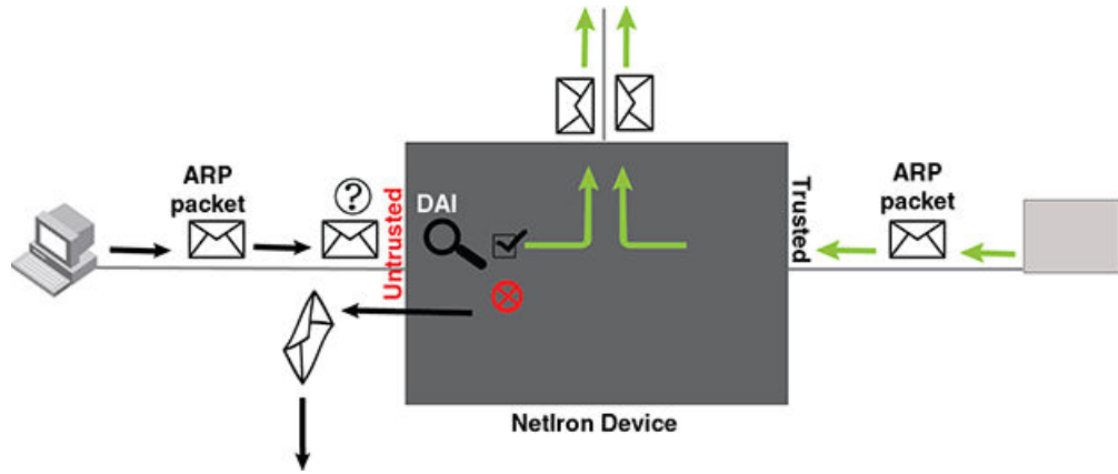
FIGURE 175 Dynamic ARP inspection at work
