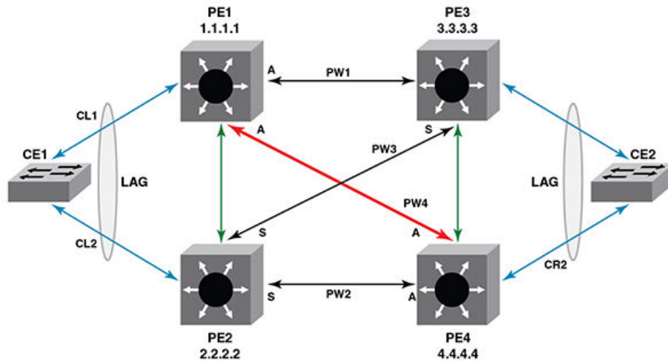
FIGURE 166 Sample topology with MCT end-points for VLL
