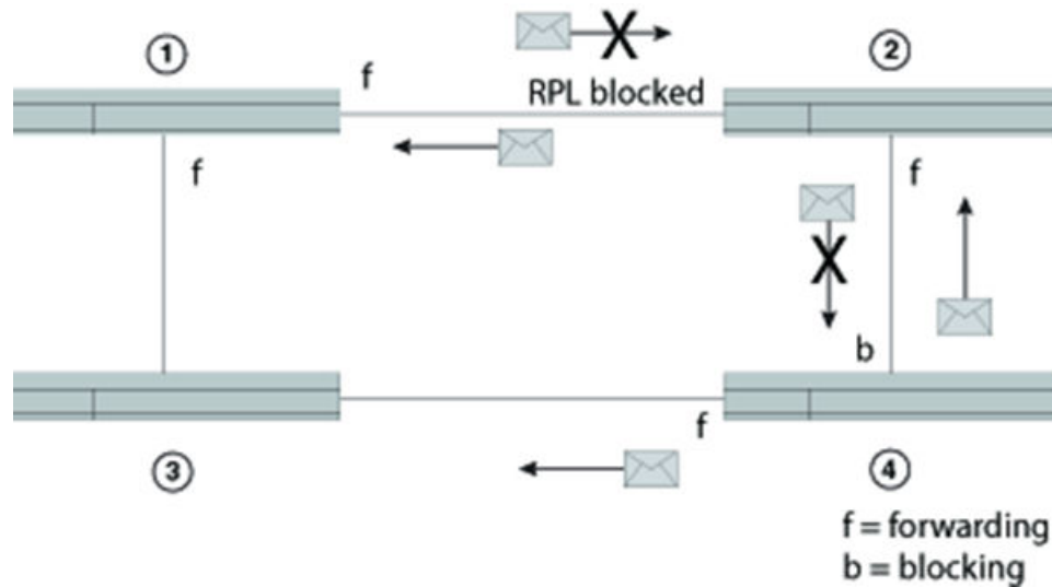
FIGURE 126 Initializing an ERP topology - VI
