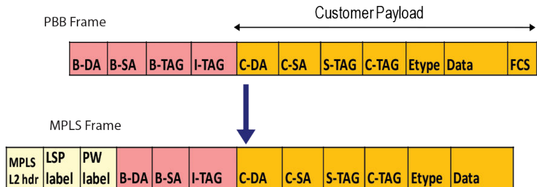
FIGURE 34 ISID mapping
