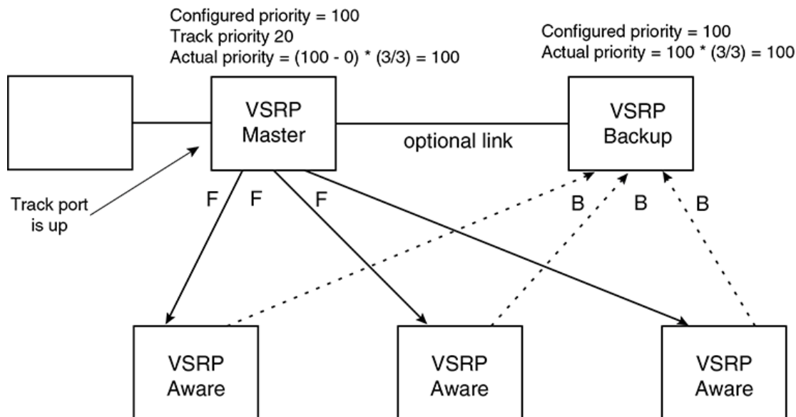
FIGURE 143 Track port priority
