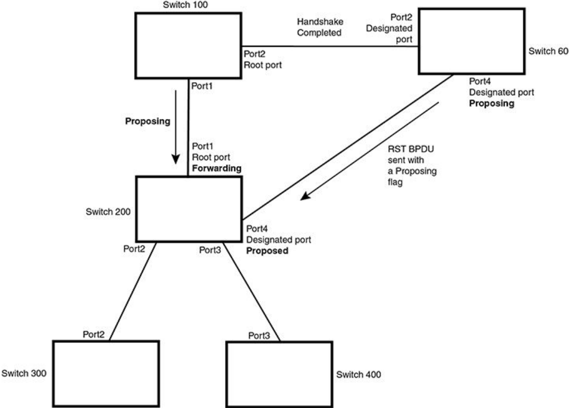
FIGURE 75 New root bridge sending a proposal flag
