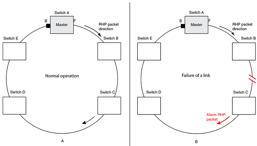
FIGURE 105 An MRP ring under normal operation (A) and after detection of a failure in the ring (B)
