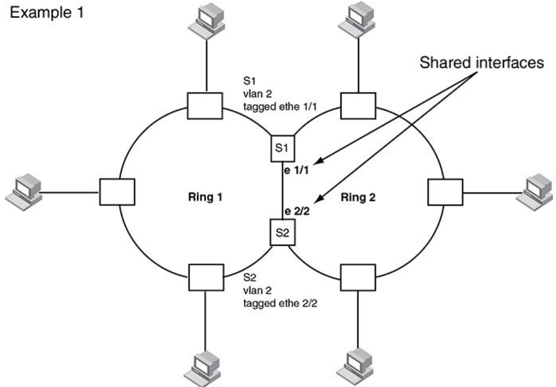
FIGURE 110 Example 1 multiple rings sharing interfaces - phase 2
