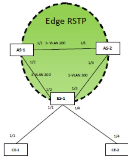
FIGURE 97 Edge RSTP topology 5
