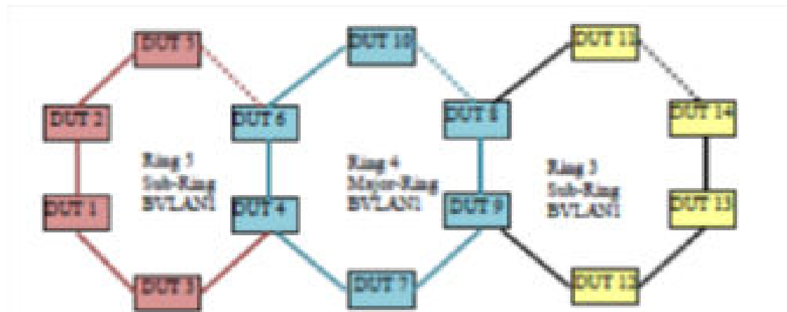
FIGURE 136 ERP configuration with same VLAN
