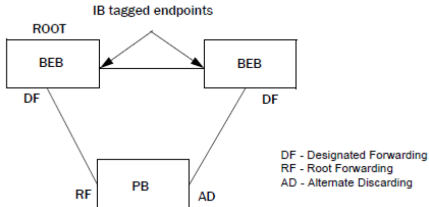
FIGURE 92 RSTP convergence when two AS connected via IB tagged endpoint
