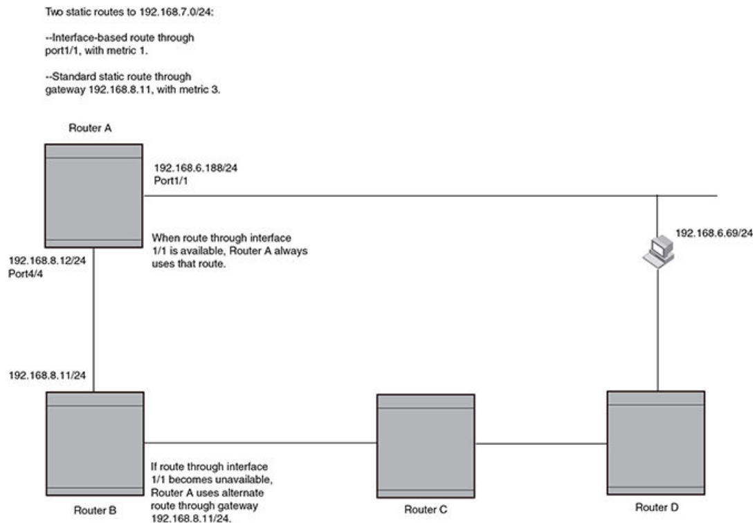
FIGURE 183 Standard and interface routes to the same destination network
