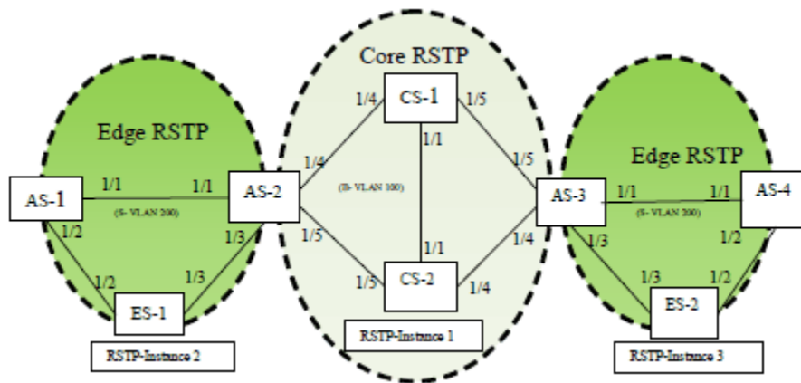
FIGURE 99 RSTP deployment in PB and PBB network
