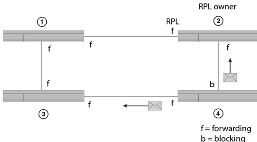
FIGURE 121 Initializing an ERN topology - I
