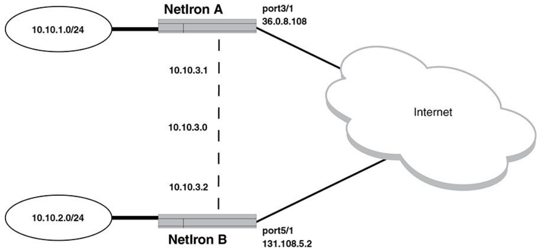
FIGURE 171 GRE IP tunnel configuration example
