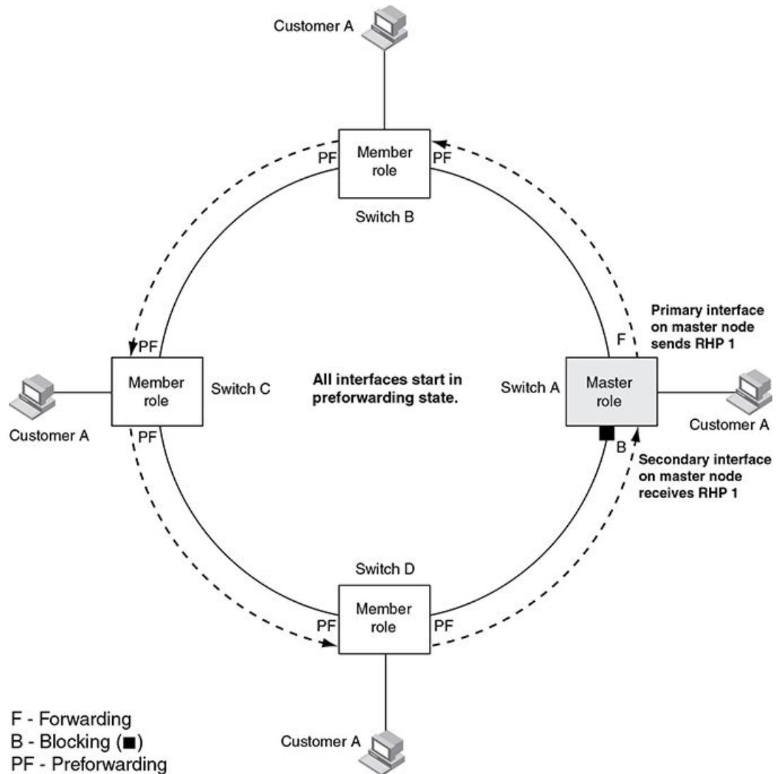
FIGURE 102 MRP ring - initial state
