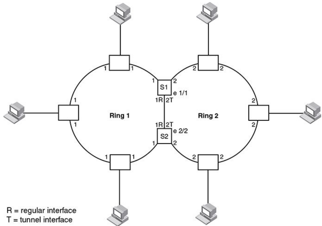
FIGURE 113 Interface IDs and types
