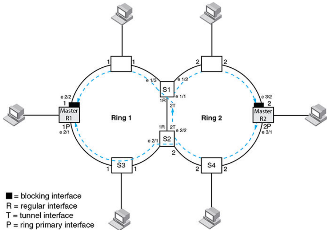
FIGURE 117 RHP flow on rings with shared interfaces showing ring 2 RHP flow
