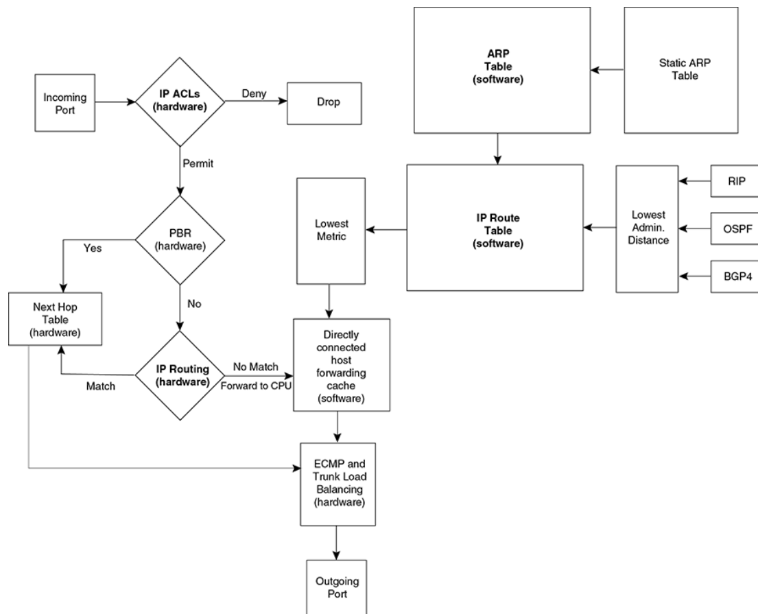
FIGURE 169 IP Packet flow through a Brocade device
