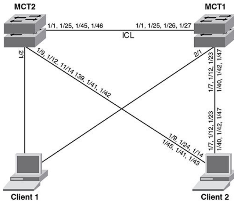
FIGURE 167 MCT snooping topology example
