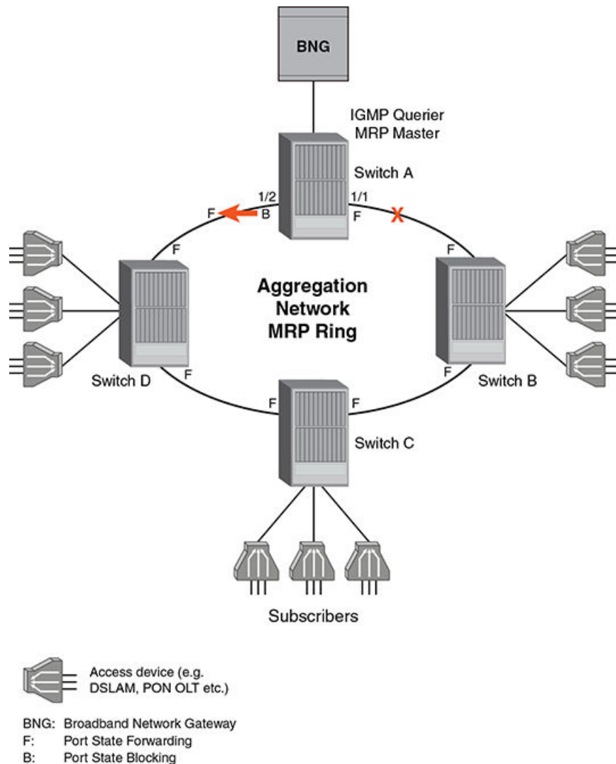
FIGURE 106 MRP ring with switch A as the querier
