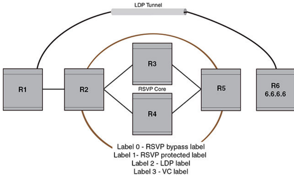
FIGURE 184 L2VPN packets over a LDP tunnel
