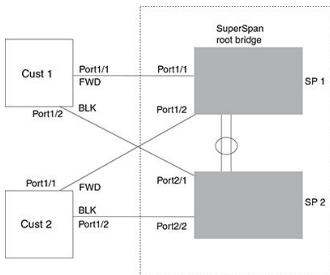
FIGURE 56 SuperSpan example
