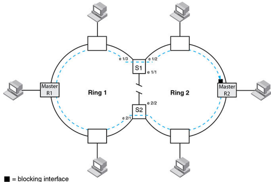
FIGURE 118 Flow of RHP packets when a link for shared interfaces breaks
