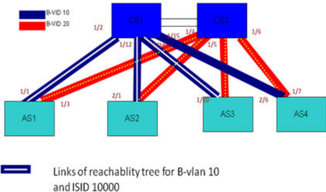
FIGURE 189 Reachability tree for B-VLAN 10 and ISID 10000
