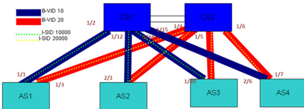
FIGURE 188 MMRP with PBB enabled
