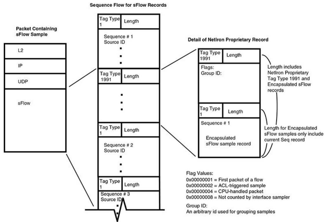
FIGURE 191 sFlow packet format
