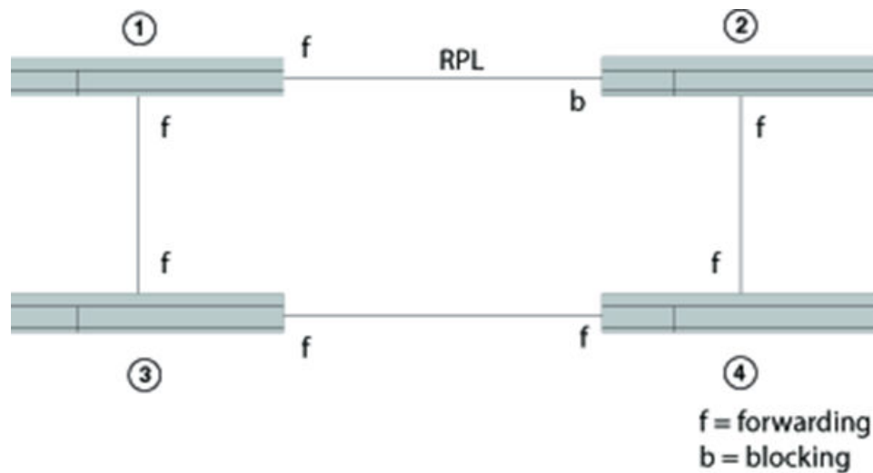
FIGURE 127 Initializing an ERP topology - VII
