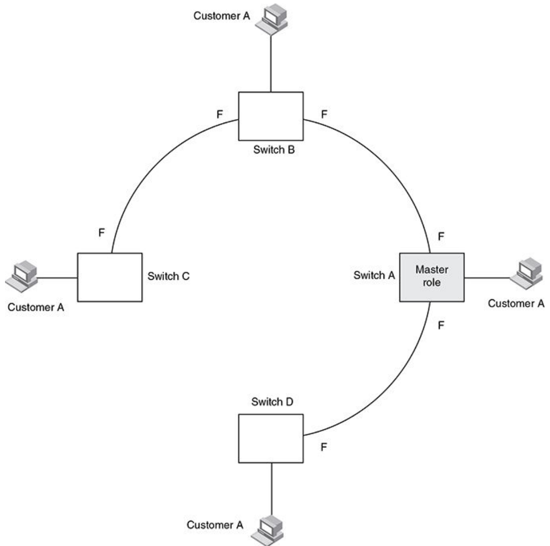
FIGURE 104 MRP ring - ring break
