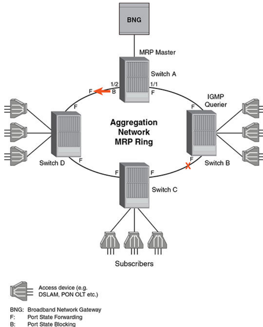
FIGURE 107 MRP ring with switch B as the querier
