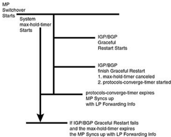
FIGURE 172 MP to LP re-syncing process
