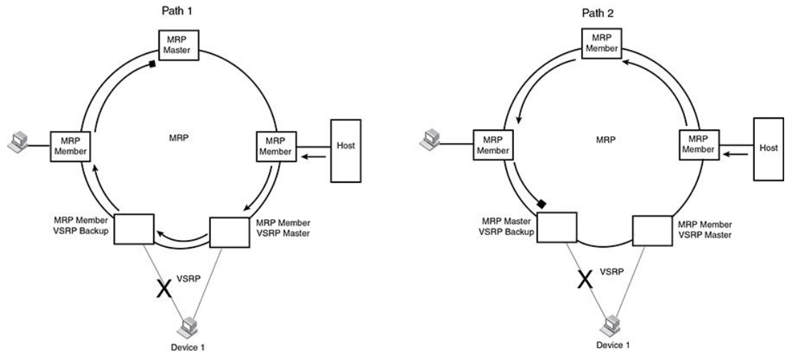
FIGURE 150 VSRP on Foundry MRP rings that failed over
