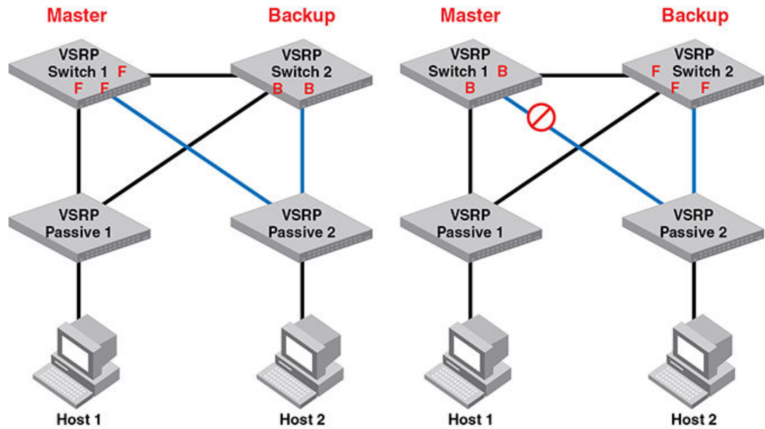
FIGURE 146 Black hole scenario 2
