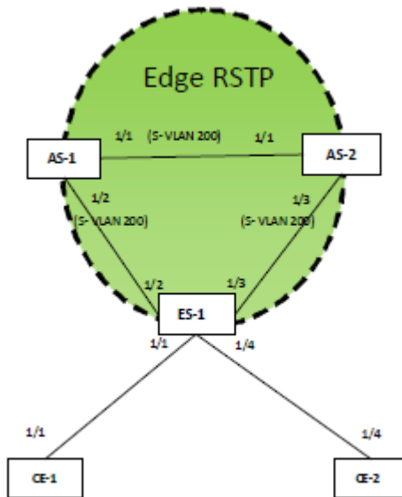
FIGURE 93 Edge RSTP topology 1
