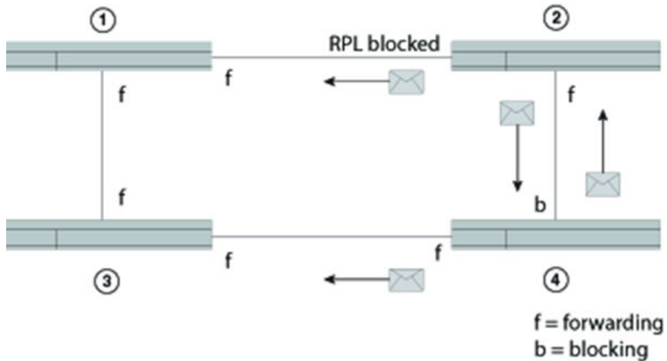
FIGURE 125 Initializing an ERP topology - V
