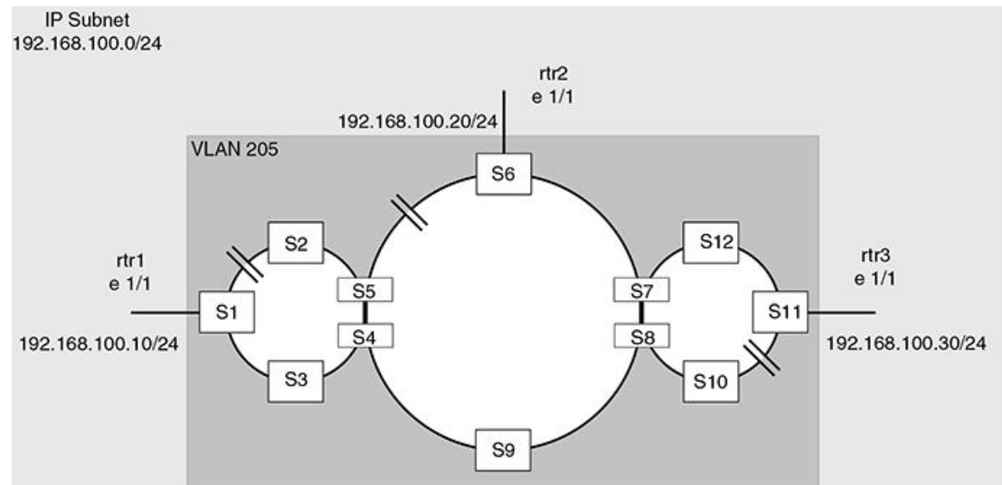
FIGURE 111 Multiple rings with one vlan spanning them
