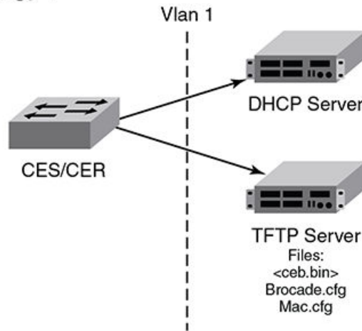
FIGURE 180 Zero Touch Provisioning
