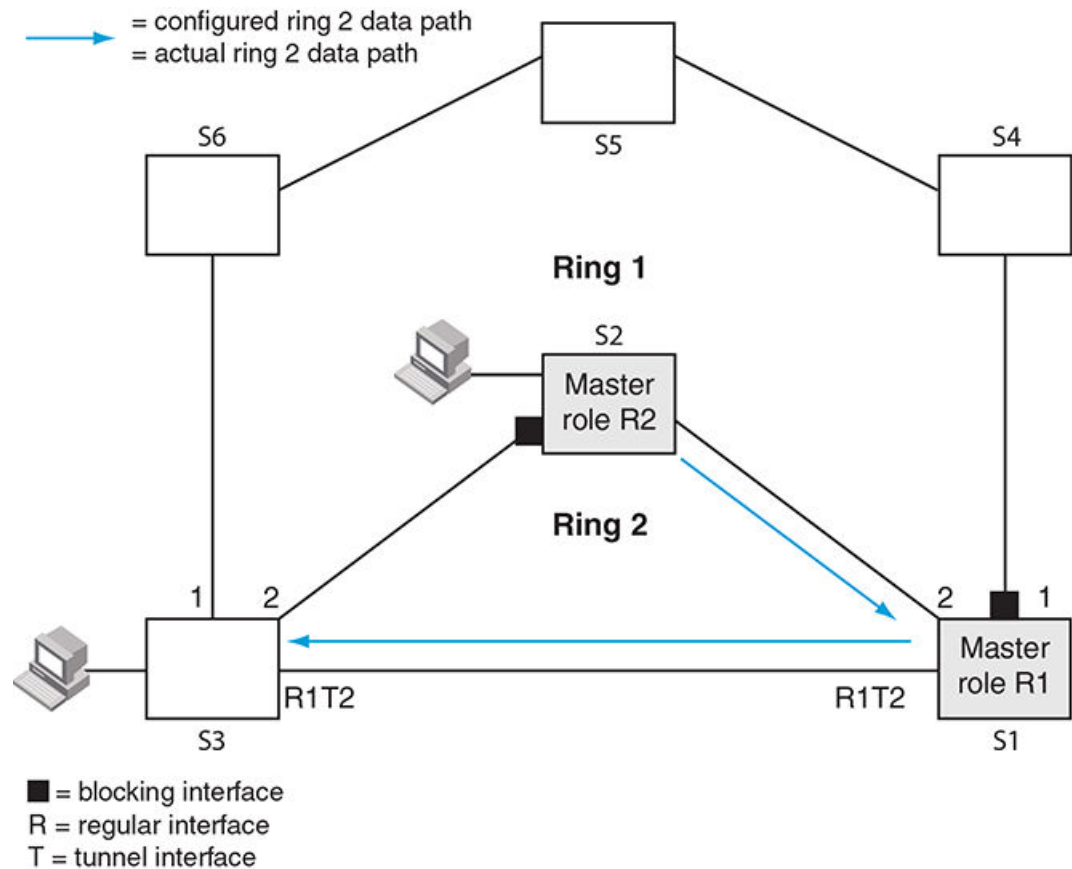
FIGURE 115 Expected switching path with shared interface
