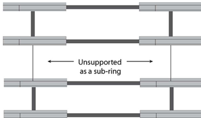
FIGURE 133 Unsupported sub-ring in segments
