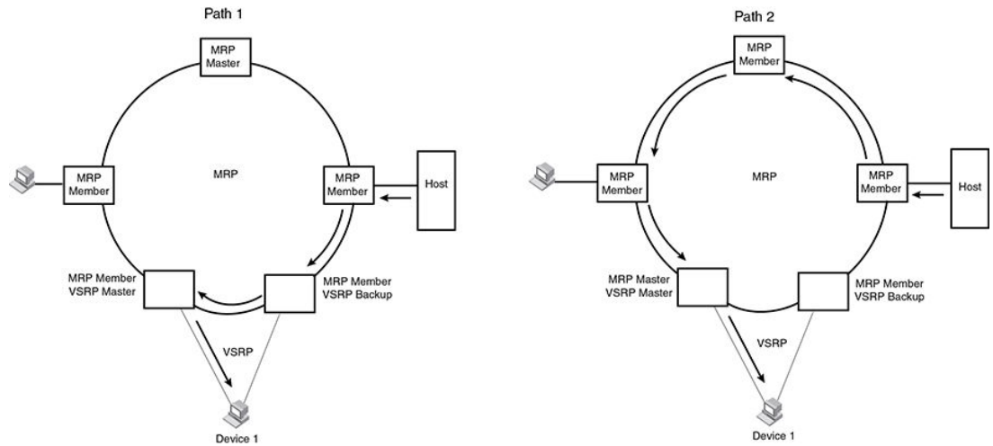
FIGURE 149 Two data paths from host on a Foundry MRP ring to a VSRP-linked device
