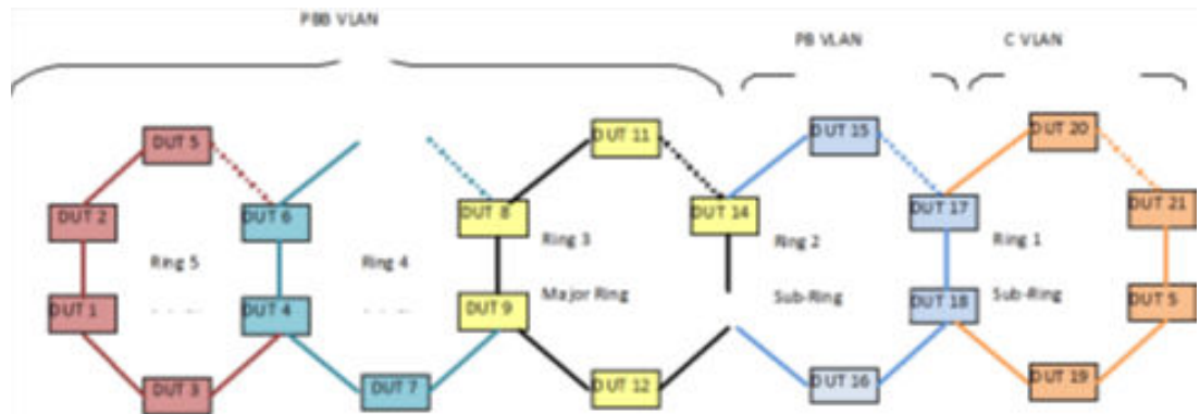
FIGURE 135 ERP configuration over ESI network
