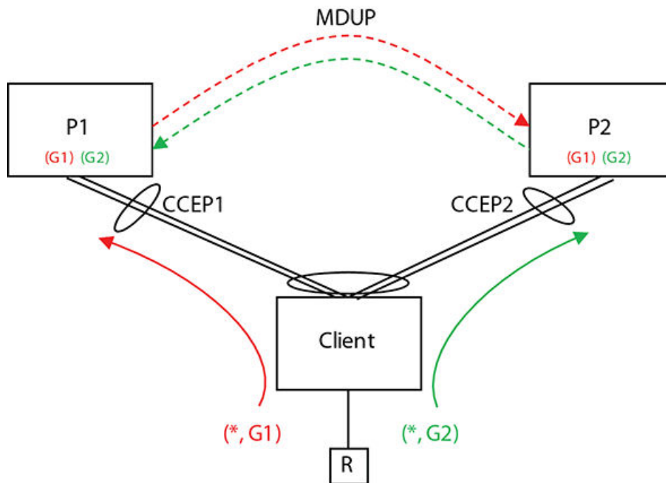
FIGURE 168 Synchronizing IGMP State on the CCEPs
