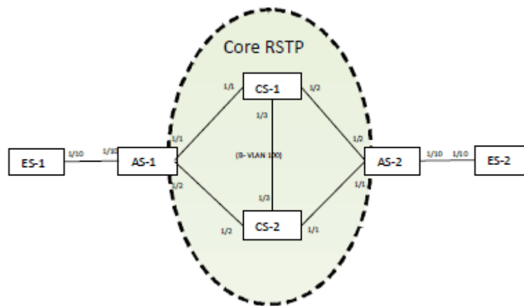
FIGURE 98 Core RSTP in PBB network
