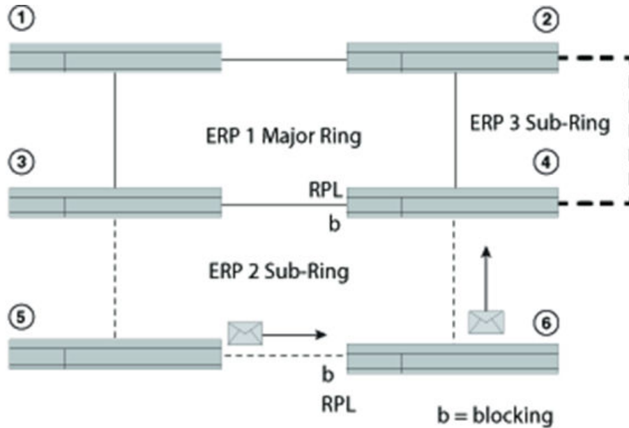
FIGURE 132 Interconnected rings with major and sub rings shown
