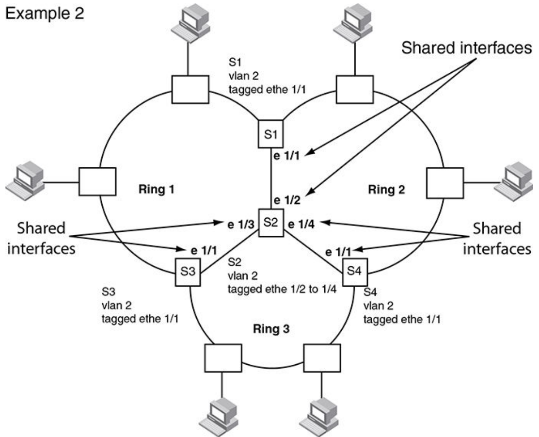
FIGURE 112 Example 2 multiple rings sharing interfaces - phase 2
