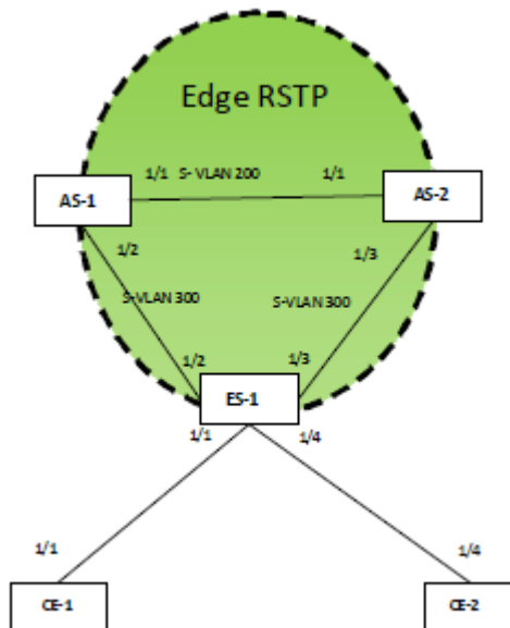
FIGURE 94 Edge RSTP topology 2
