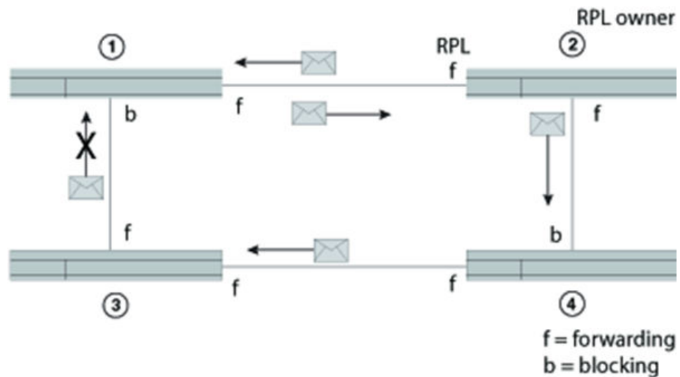
FIGURE 123 Initializing an ERP topology - III
