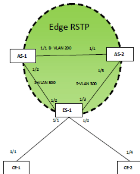
FIGURE 95 Edge RSTP topology 3
