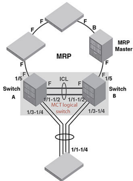
FIGURE 162 MRP integration with MCT
