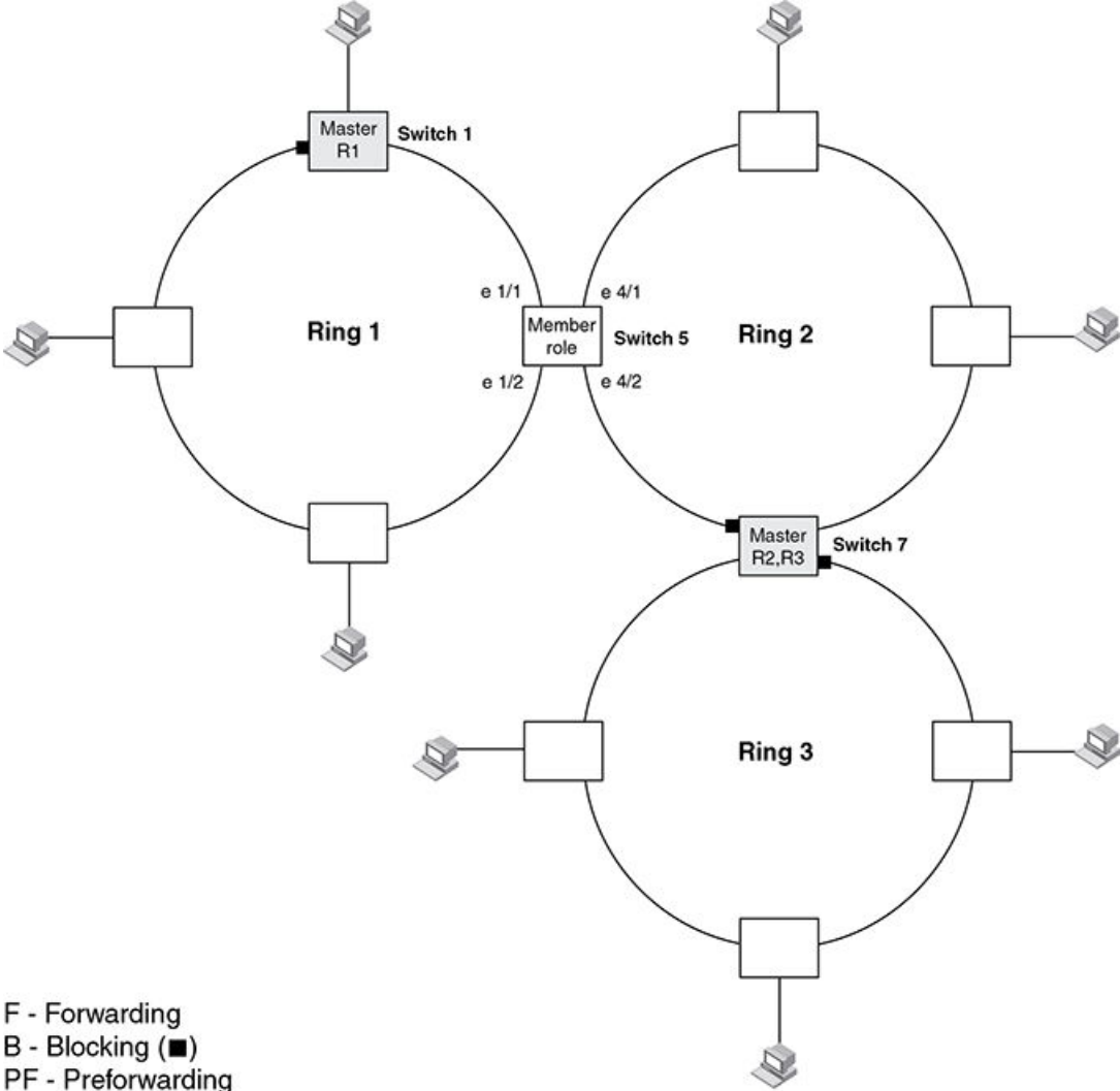
FIGURE 109 Multiple MRP rings - phase 1
