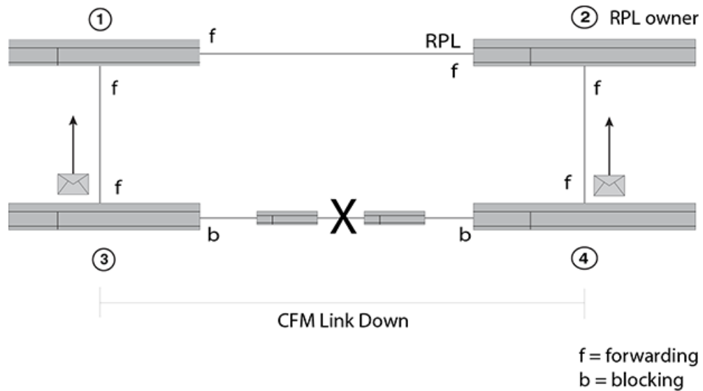
FIGURE 120 ERP with IEEE 802.1ag support
