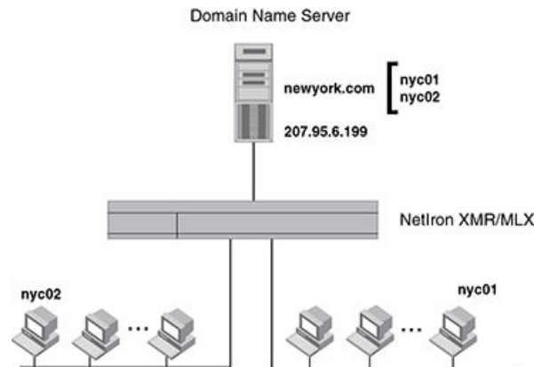
FIGURE 174 Querying a host on the newyork.com domain
