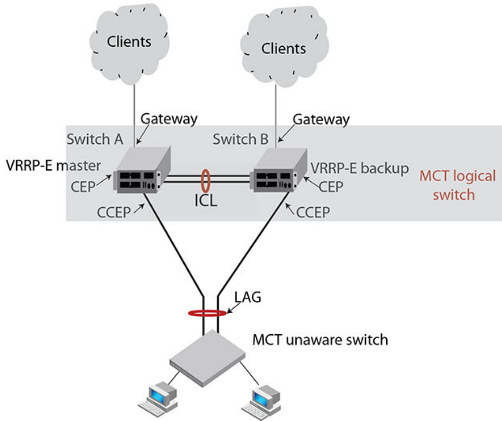
FIGURE 163 Example of MCTS that are Layer 2 switched
