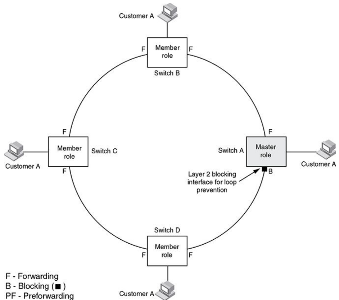
FIGURE 100 MRP - normal state
