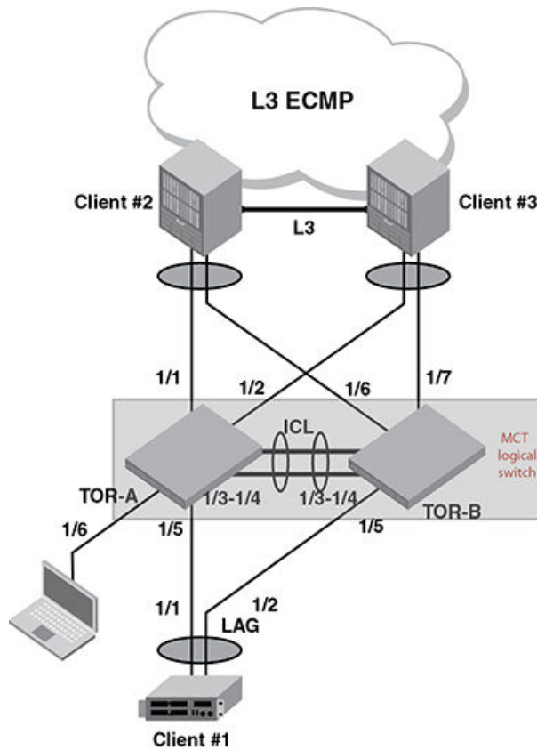
FIGURE 160 Single level MCT- extension
