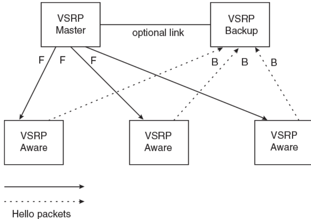
FIGURE 140 VSRP mesh - redundant paths for Layer 2 traffic
