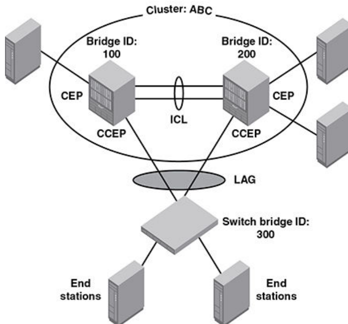
FIGURE 154 MCT Components
