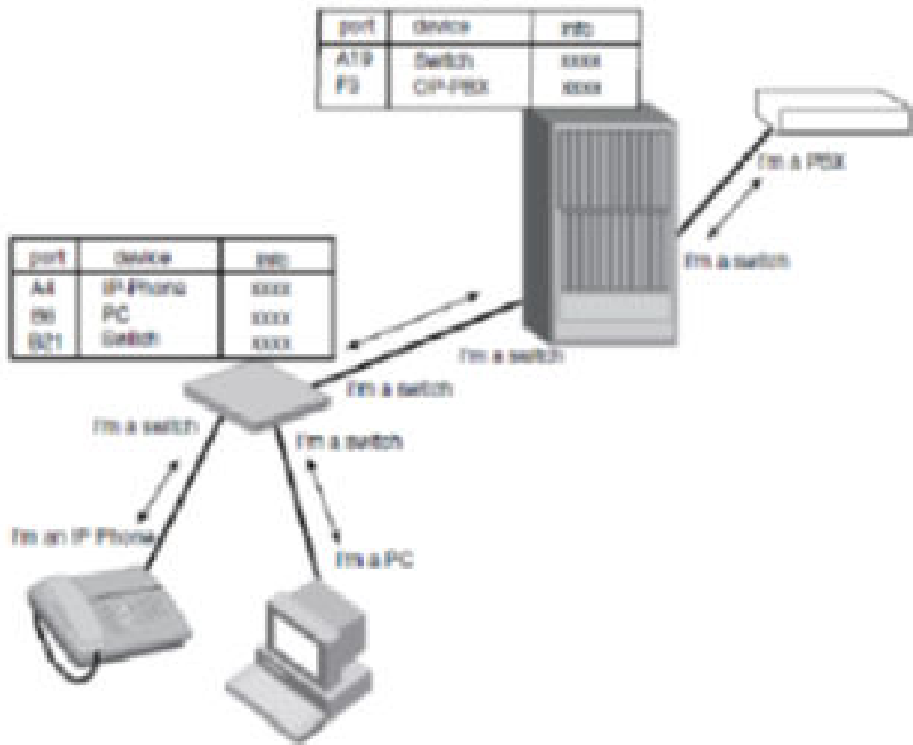
FIGURE 2 LLDP connectivity
