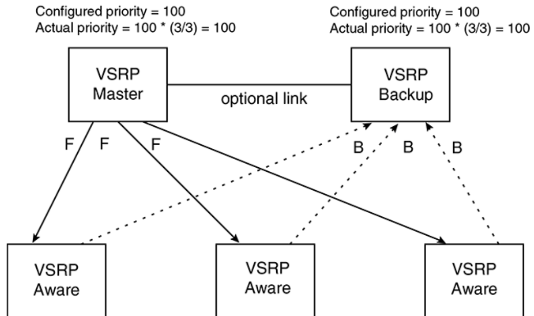
FIGURE 141 VSRP priority
