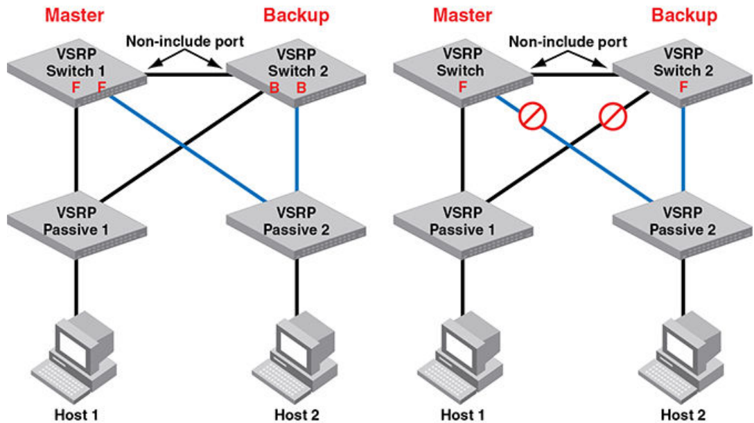
FIGURE 148 Correct VSRP behavior
