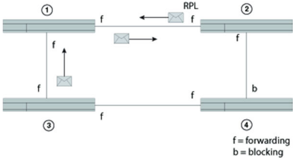
FIGURE 124 Initializing an ERP topology - IV
