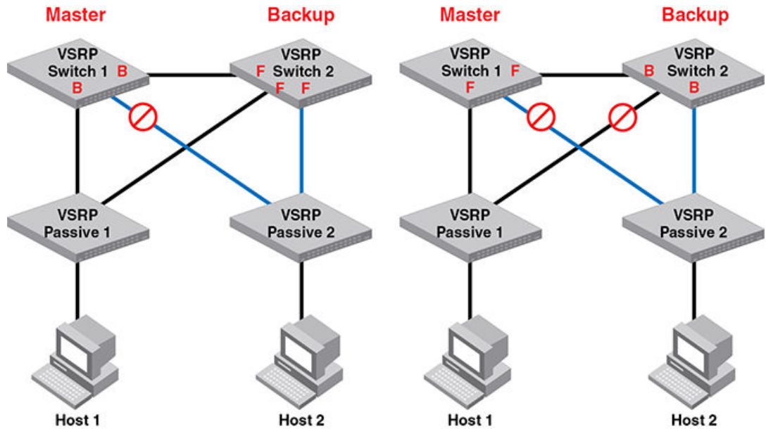
FIGURE 147 Black hole scenario 3
