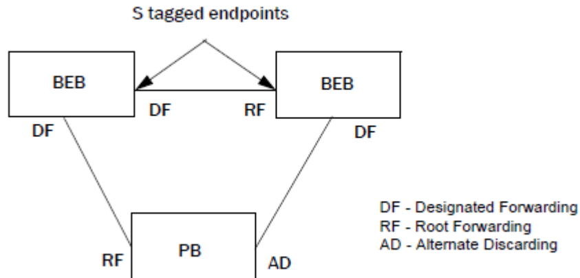
FIGURE 91 RSTP convergence when two AS connected via S tagged endpoint
