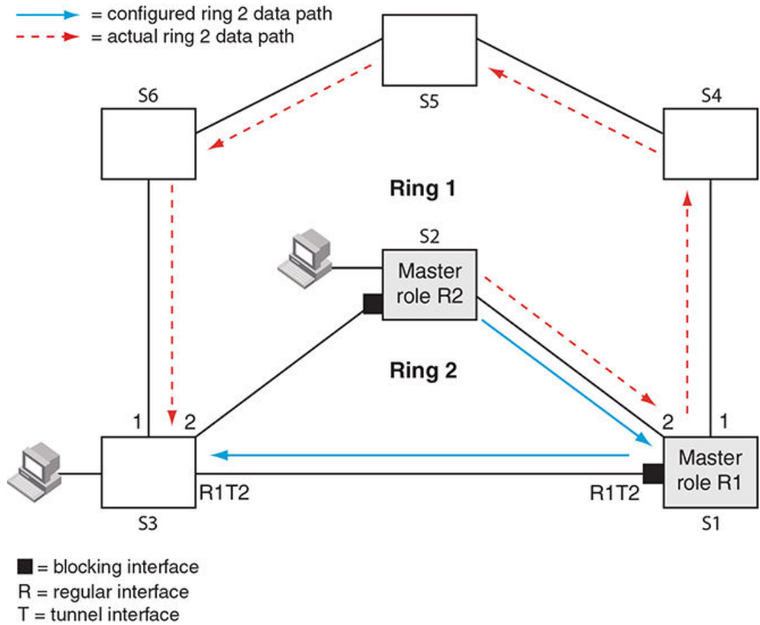
FIGURE 114 Unexpected switching path with shared interface
