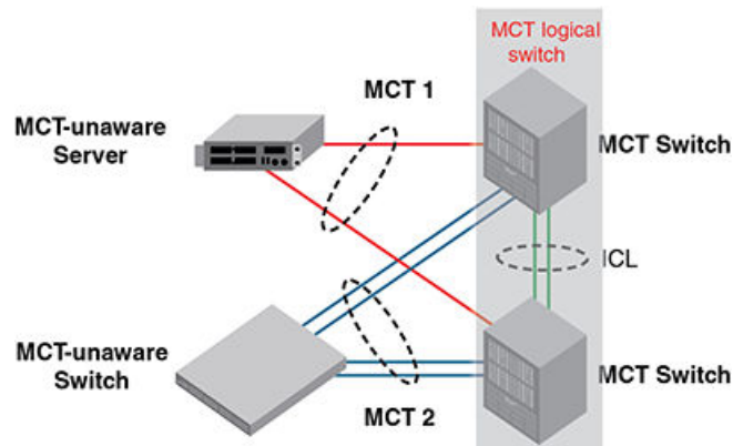
FIGURE 152 Chassis trunk example
