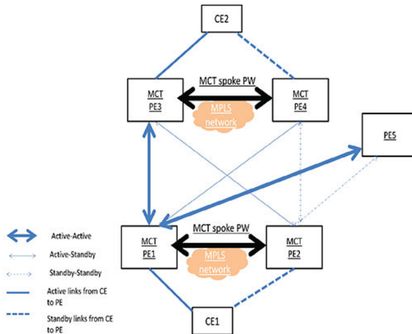
FIGURE 156 MCT Active-Passive topology
