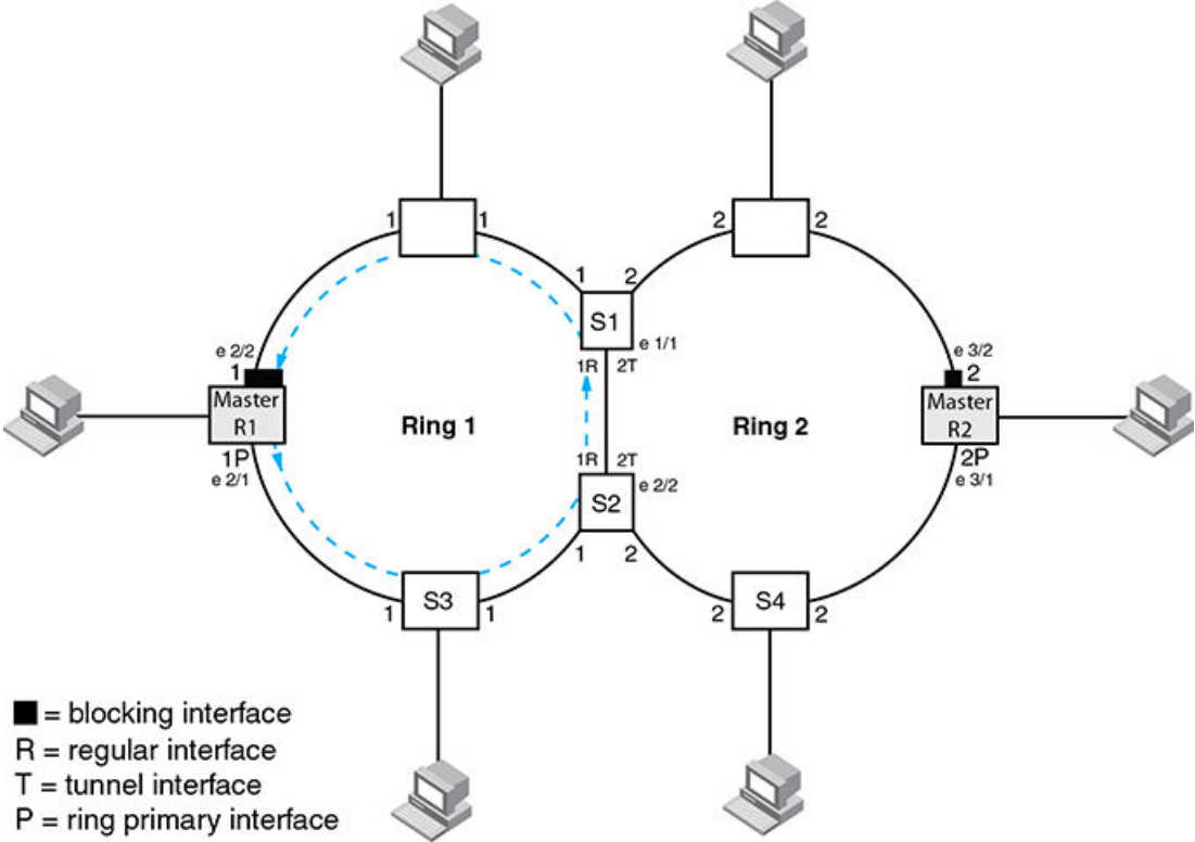
FIGURE 116 RHP flow on rings with shared interfaces showing ring 1 RHP flow
