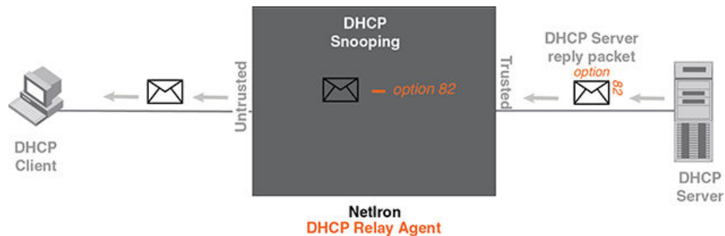
FIGURE 179 DHCP option 82 is removed from the packet
