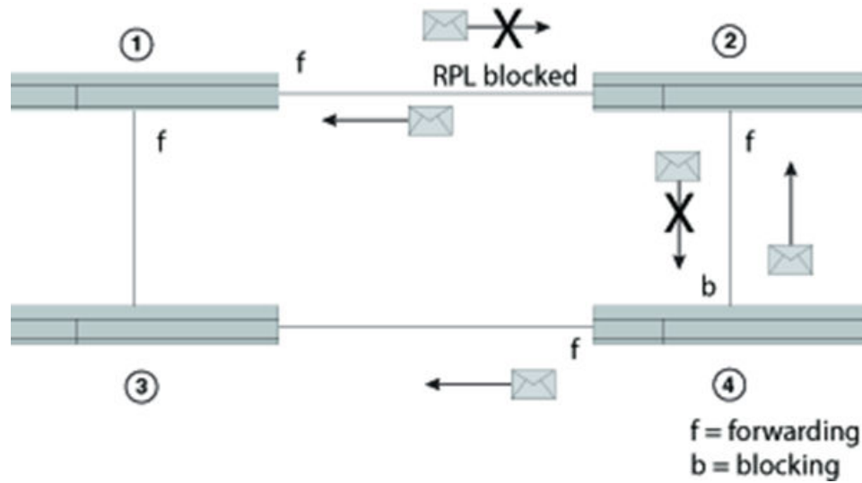
FIGURE 126 Initializing an ERP topology - VI
