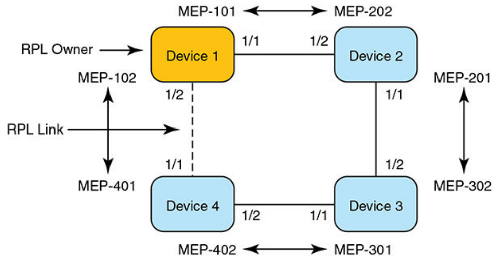
FIGURE 134 Network diagram for ERP
