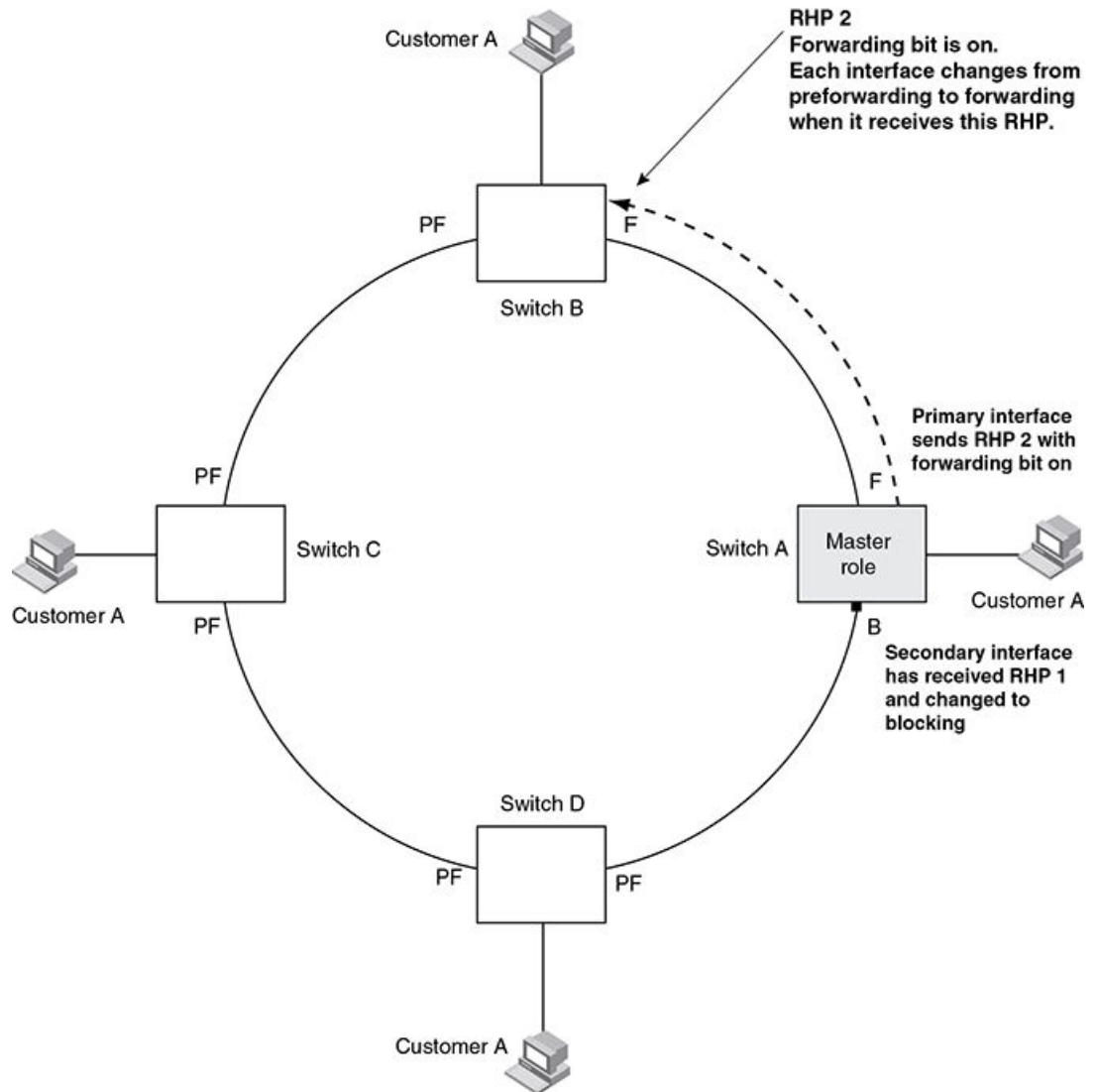
FIGURE 103 MRP ring - from preforwarding to forwarding
