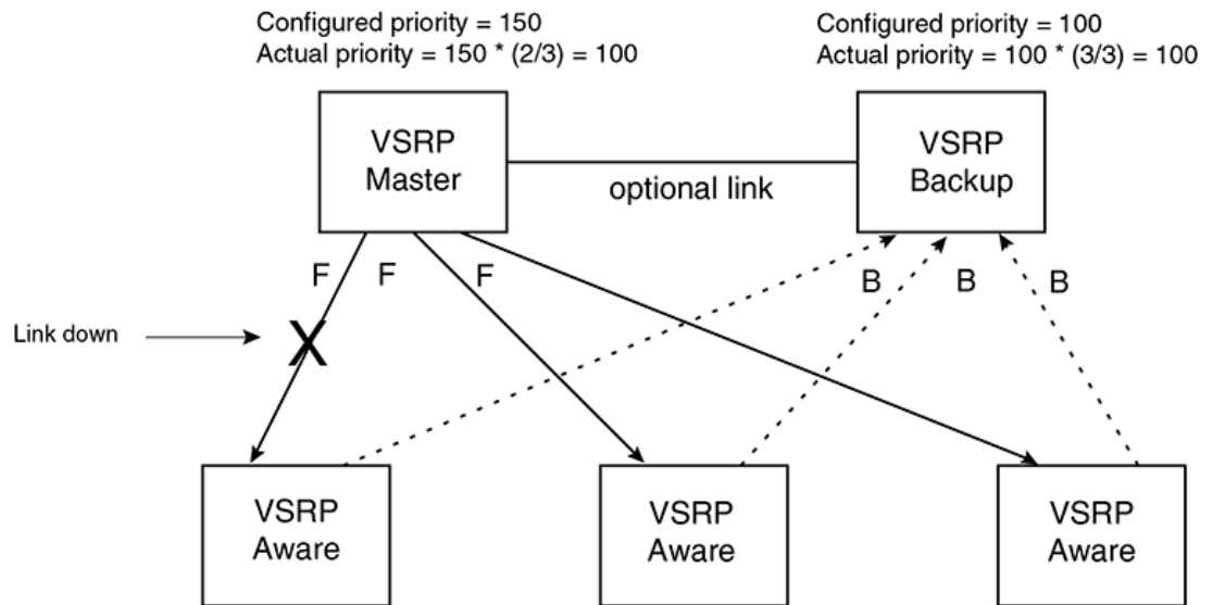
FIGURE 142 VSRP priority bias
