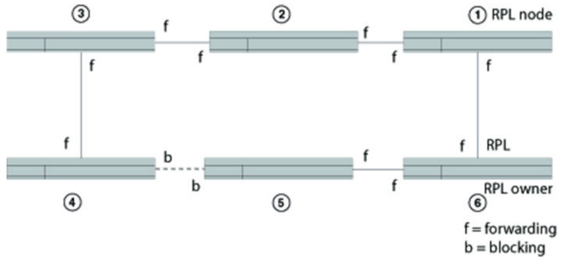
FIGURE 129 ERP topology in a Protected state
