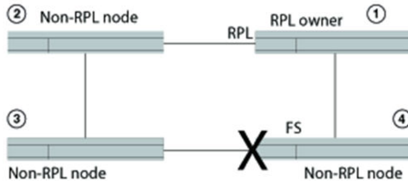
FIGURE 131 Single forced switch scenario
