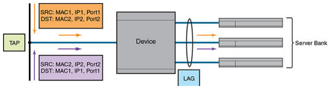
FIGURE 185 Symmetric load balancing for LAGs
