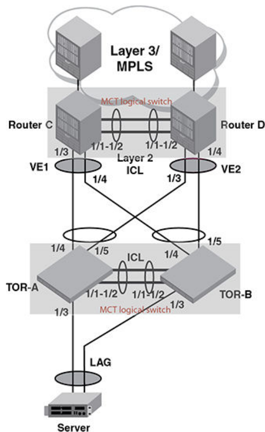
FIGURE 161 Two level MCT
