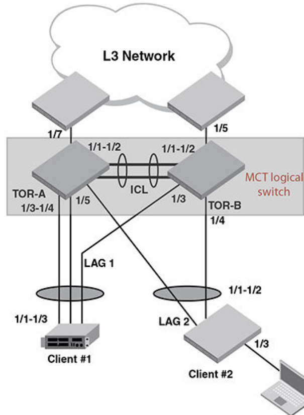
FIGURE 157 Single level MCT
