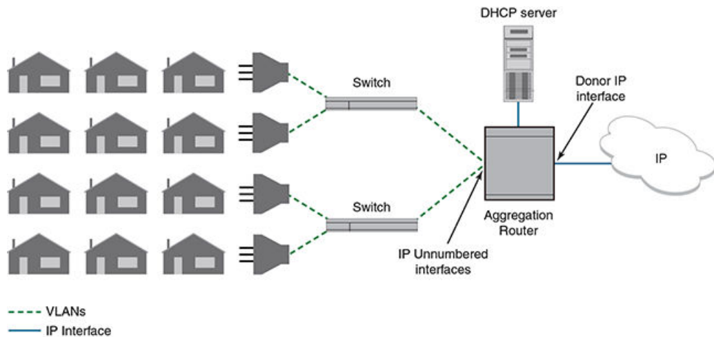
FIGURE 173 IP Unnumbered Interfaces feature
