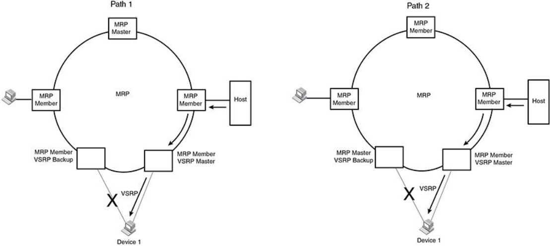
FIGURE 151 New path established
