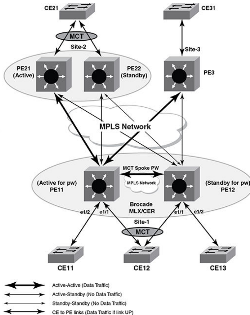
FIGURE 165 Sample topology with MCT end-points for VPLS
