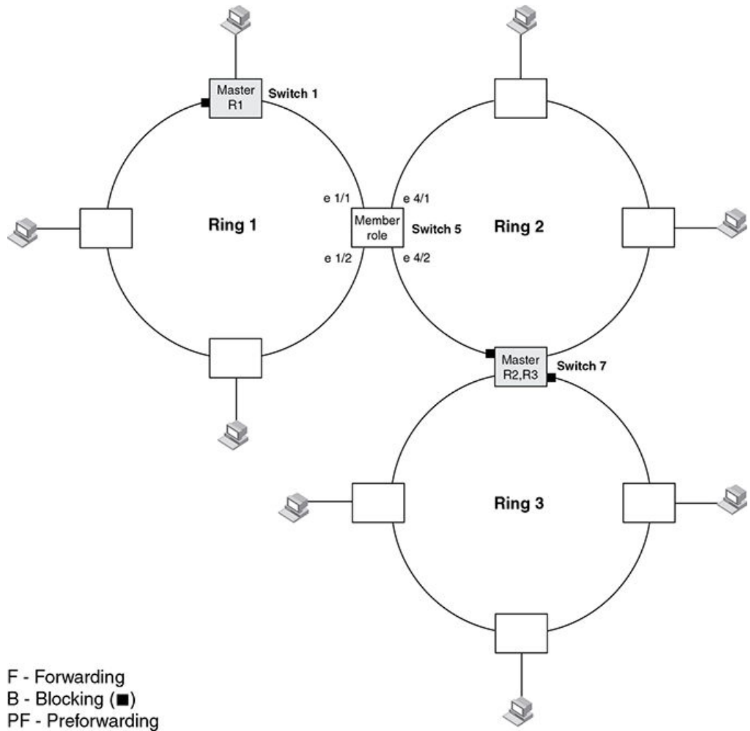
FIGURE 101 MRP - multiple rings, no shared interfaces
