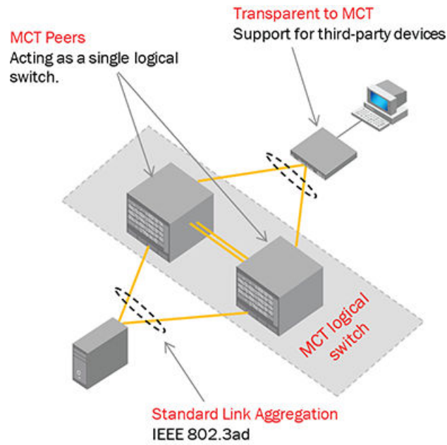
FIGURE 153 How MCT works
