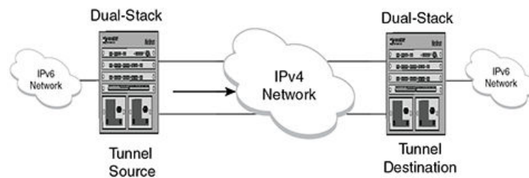
FIGURE 186 Manually configured tunnel
