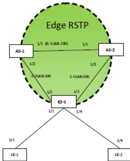
FIGURE 96 Edge RSTP topology 4
