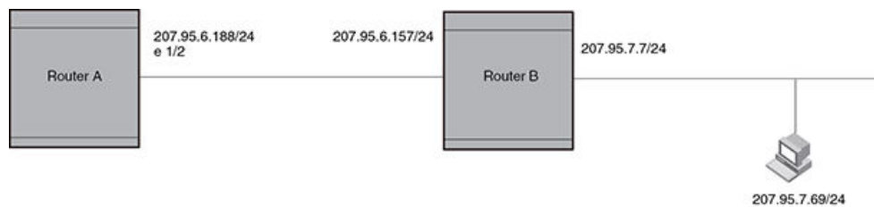
FIGURE 181 Example of a static route
