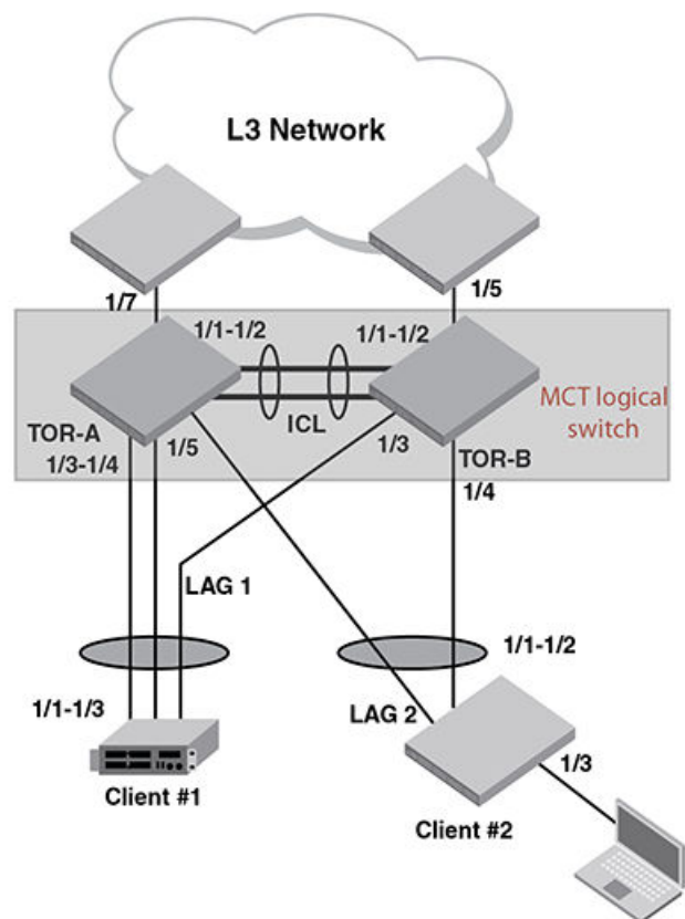
FIGURE 159 Single level MCT
