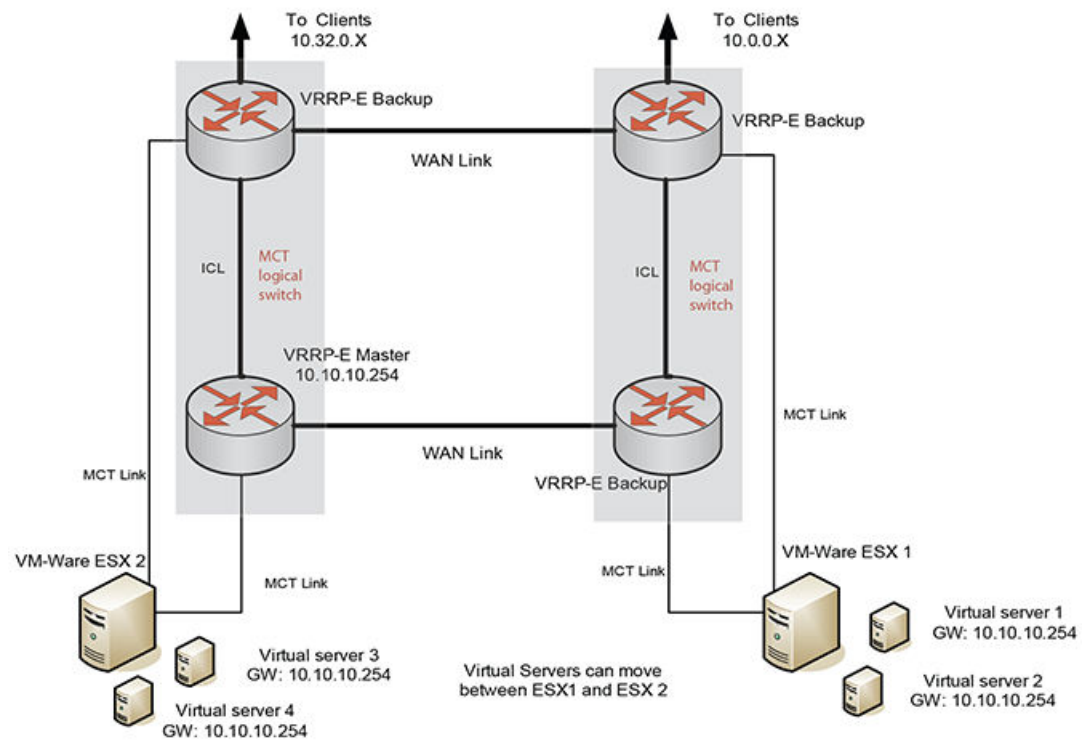
FIGURE 164 Example of MCTs that are deployed on two sites that are connected through two WAN links.
