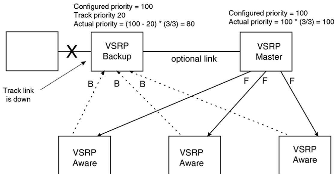
FIGURE 144 Track port priority subtracted during priority calculation
