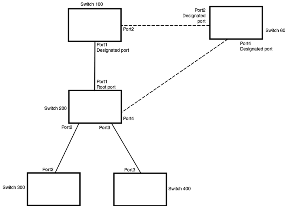
FIGURE 74 Addition of a new root bridge
