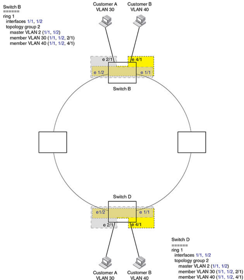
FIGURE 108 MRP ring - ring vlan and customer vlan
