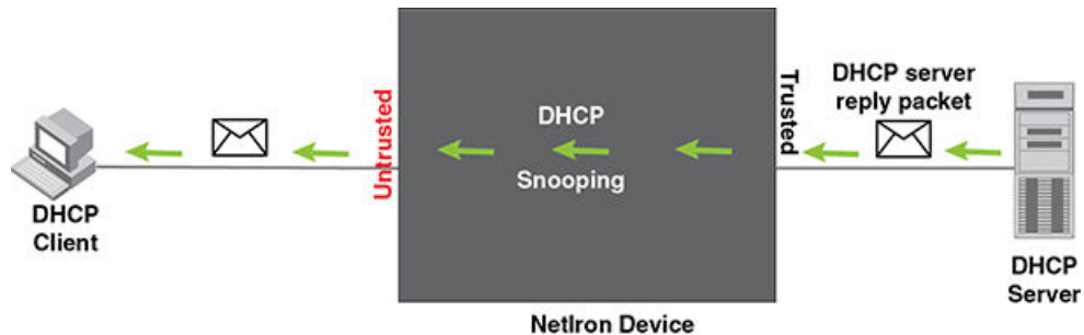
FIGURE 177 DHCP snooping at work - on trusted port
