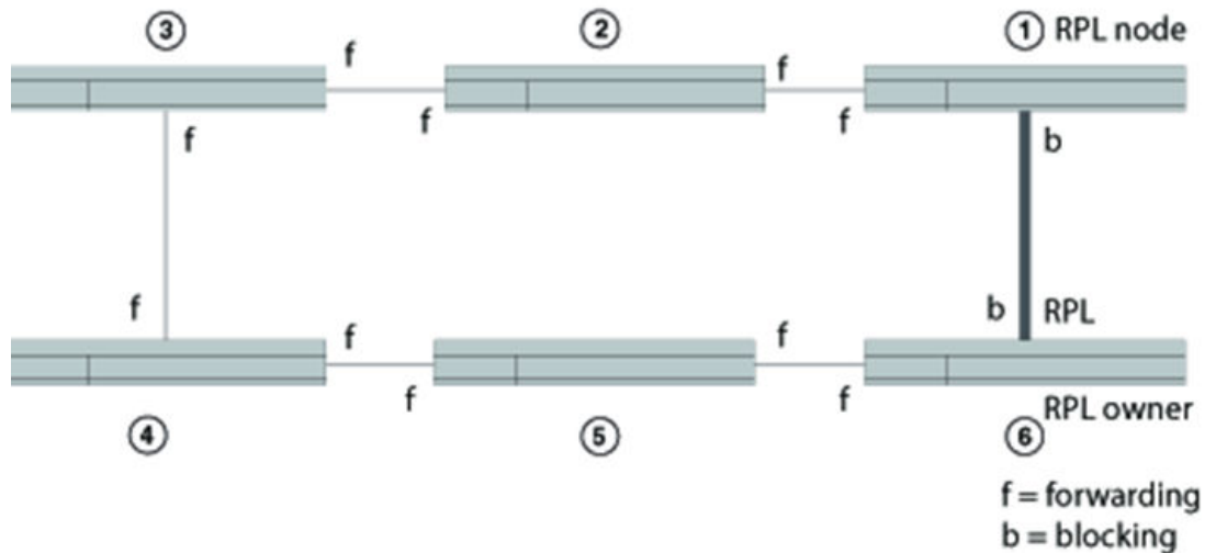
FIGURE 128 ERP topology
