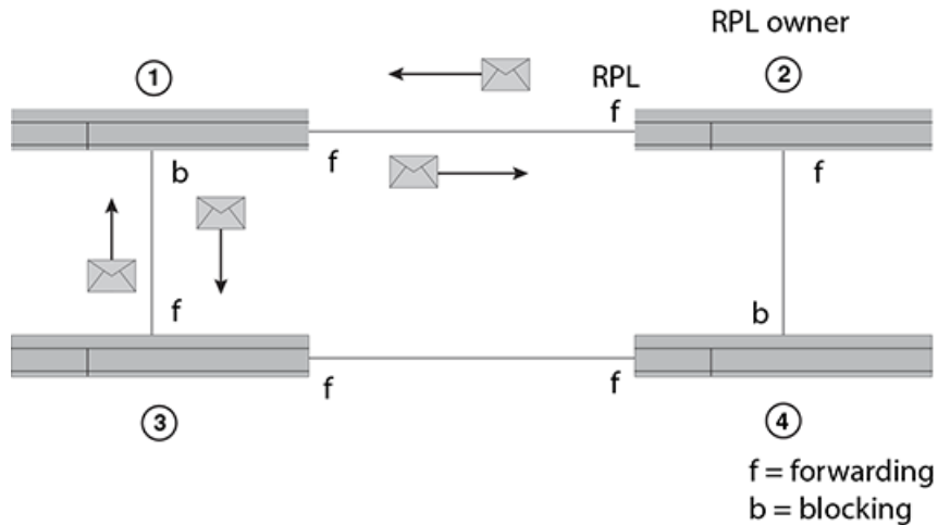
FIGURE 122 Initializing an ERP topology - II
