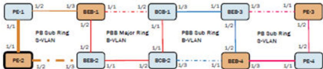
FIGURE 137 PB ring node sample configuration
