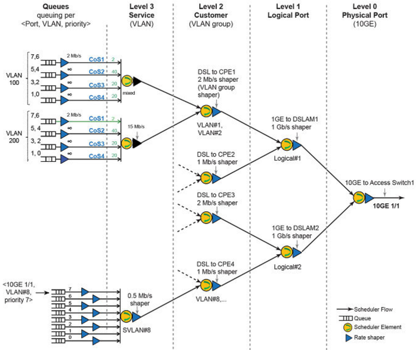
FIGURE 14 HQoS example
