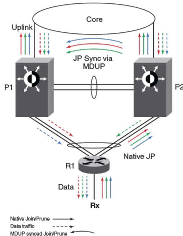
FIGURE 13 PIM over MCT reference topology
