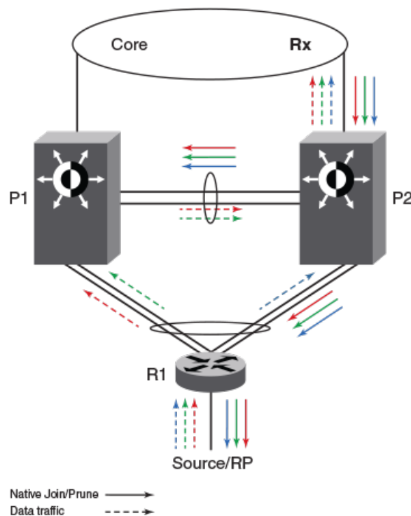
FIGURE 15 MCT peer as immediate downstream router
