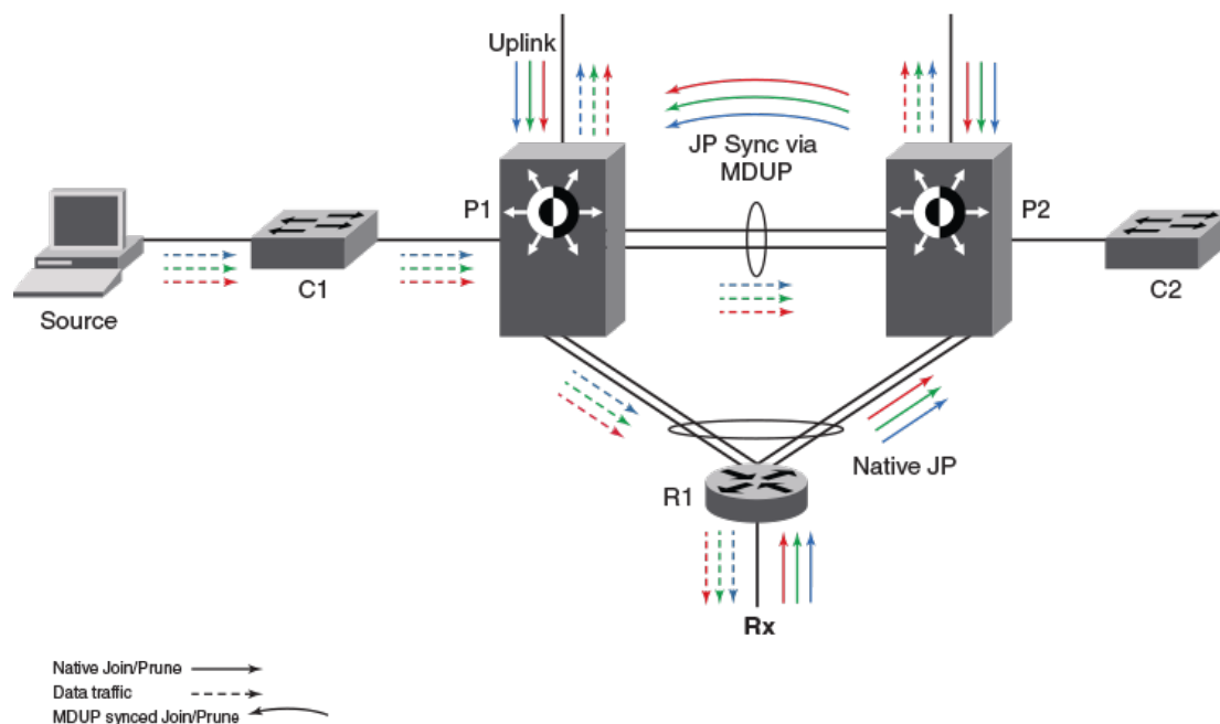
FIGURE 17 Source directly connected to CEP routers on MCT VLAN
