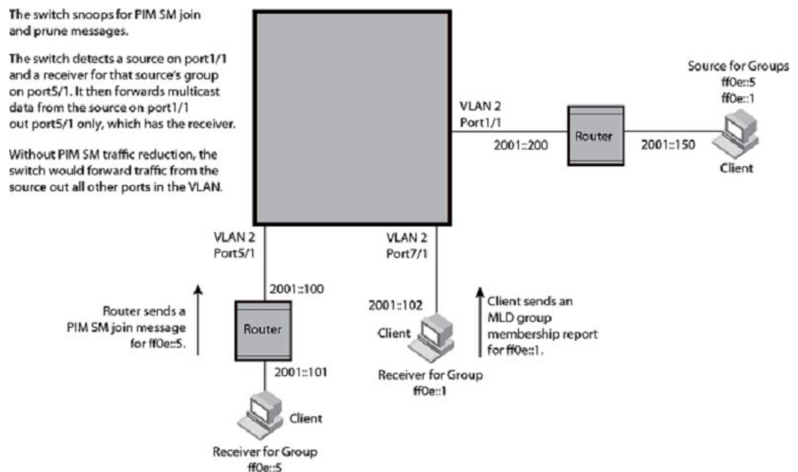
FIGURE 25 PIM-SM IPv6 traffic reduction in enterprise network
