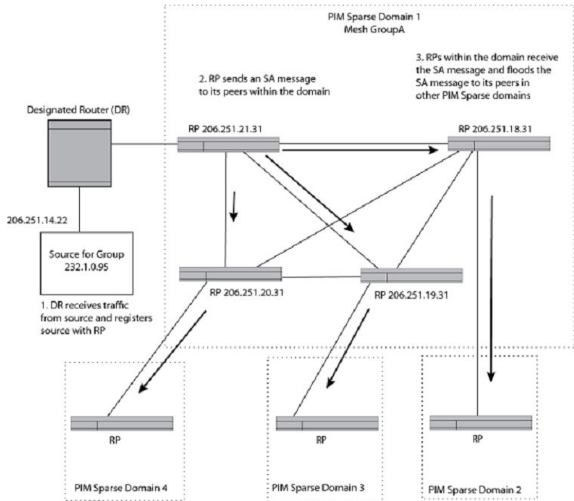
FIGURE 10 Example of MSDP mesh group
