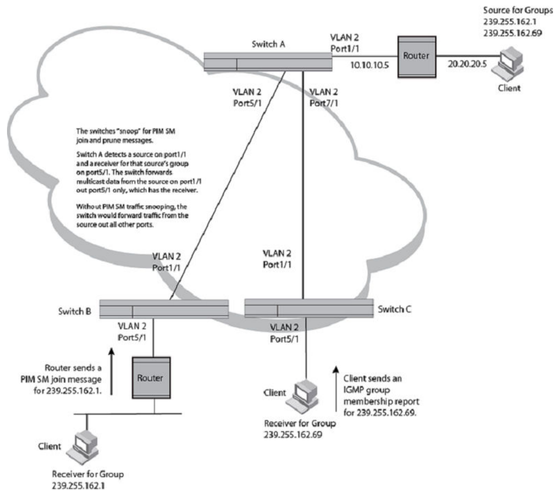
FIGURE 21 PIM SM traffic reduction in Global Ethernet environment
