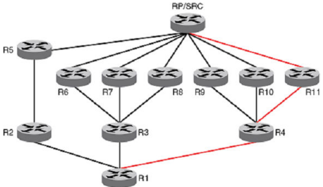
FIGURE 3 Path utilization without Multicast ECMP support
