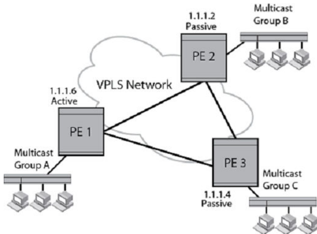
FIGURE 22 IP multicast traffic reduction in a VPLS network
