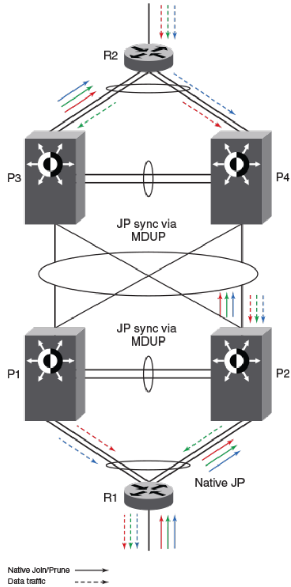
FIGURE 18 Multi tier MCT
