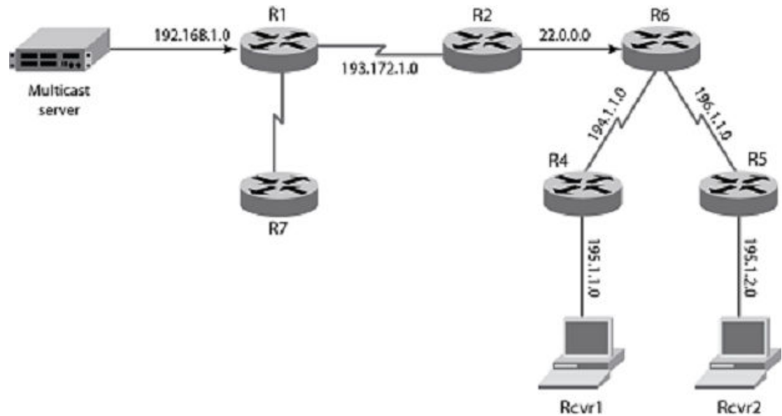
FIGURE 1 Network topology
