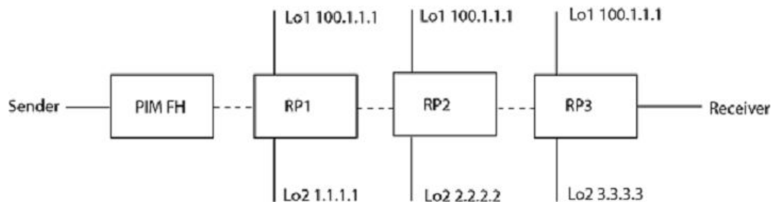
FIGURE 12 Example of a PIM Anycast RP network
