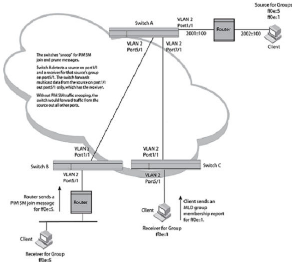
FIGURE 26 PIM-SM IPv6 traffic reduction in global Ethernet environment
