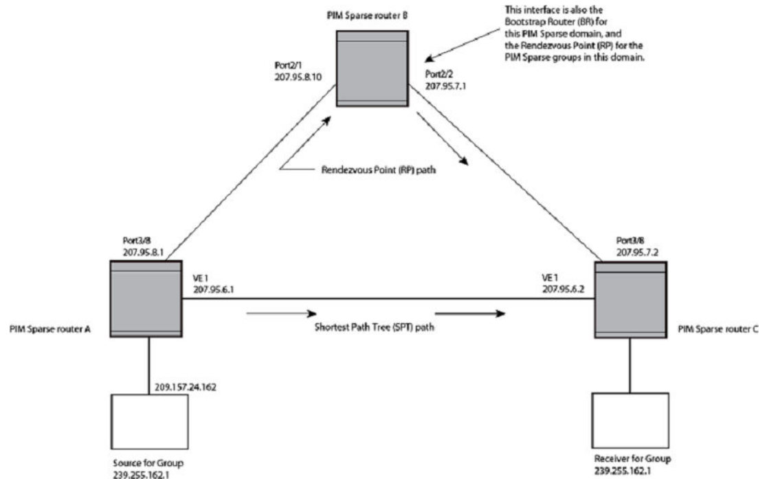
FIGURE 8 Example PIM Sparse domain
