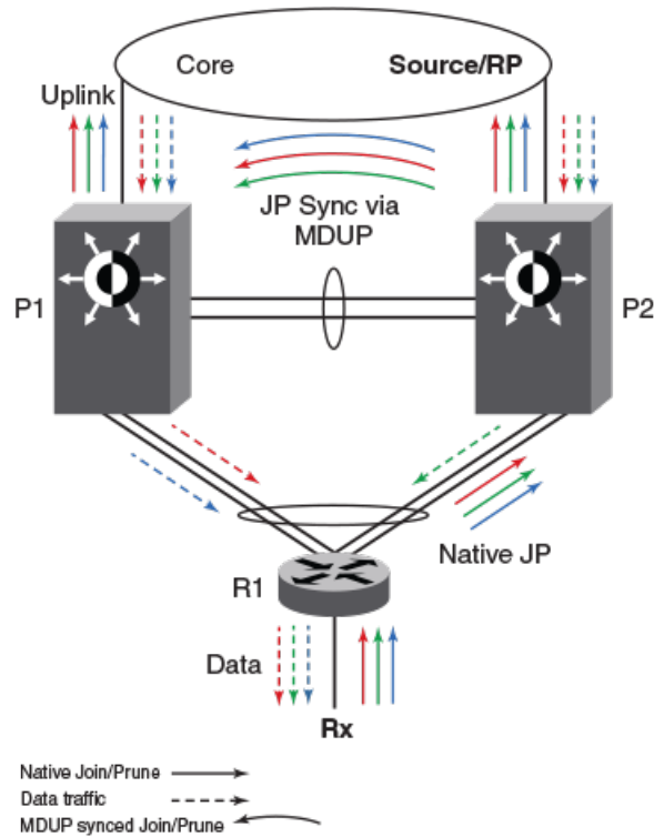
FIGURE 14 MCT peer as immediate Upstream router
