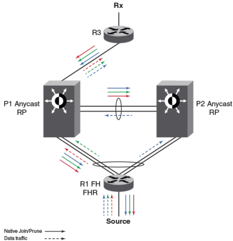
FIGURE 16 MCT peer as PIM Anycast RP
