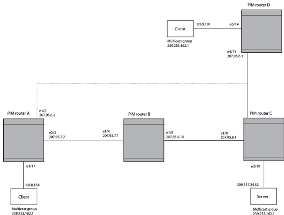
FIGURE 19 Example multicast static routes
