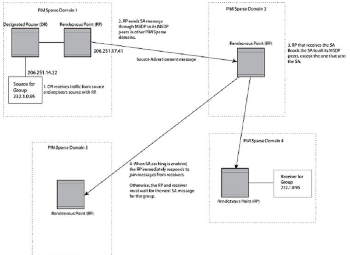
FIGURE 9 PIM Sparse domains joined by MSDP devices
