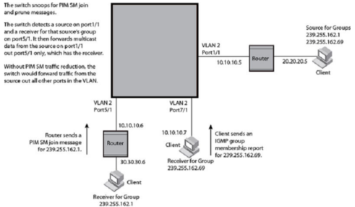
FIGURE 20 PIM SM traffic reduction in enterprise network
