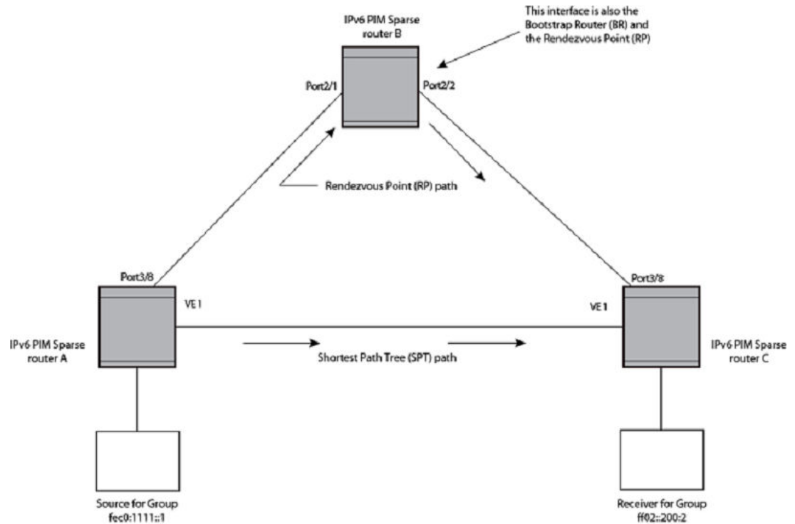
FIGURE 23 Example IPv6 PIM Sparse domain
