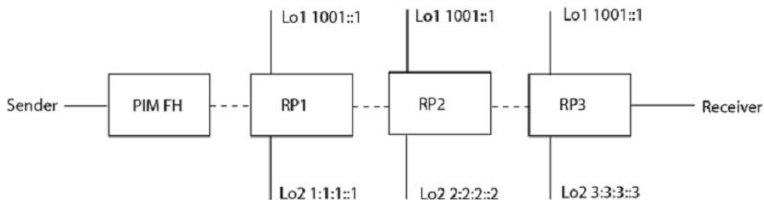
FIGURE 24 Example of a PIM Anycast RP network
