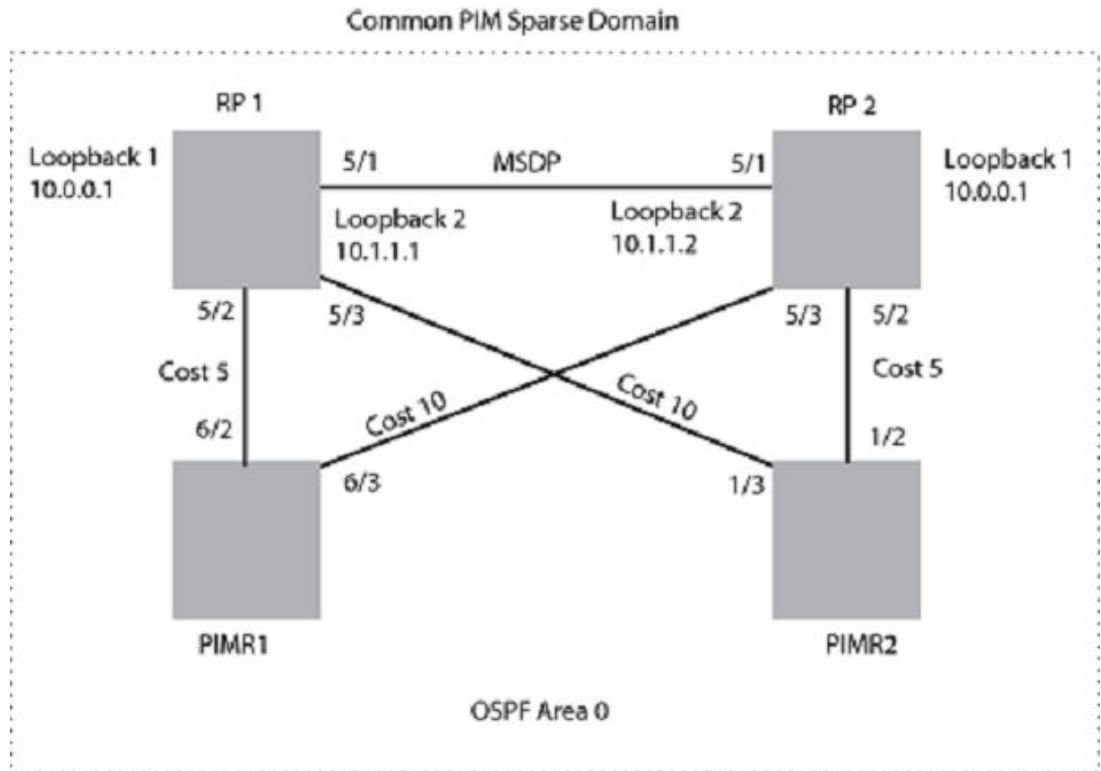
FIGURE 11 Example of a MSDP Anycast RP network
