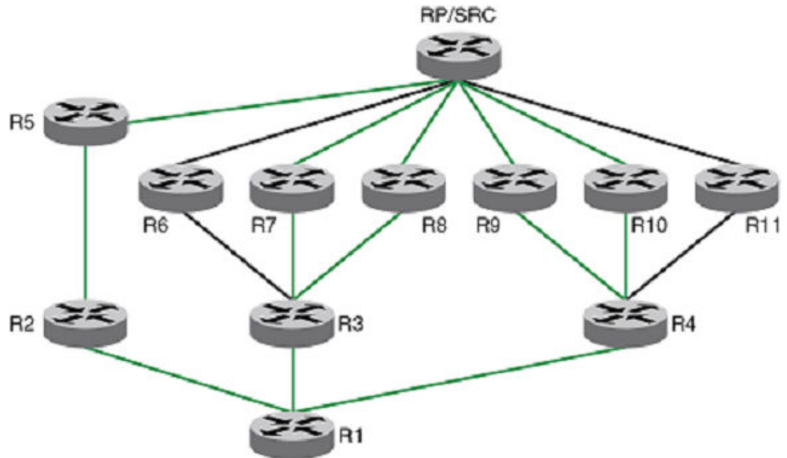
FIGURE 4 Path utilization with Multicast ECMP support
