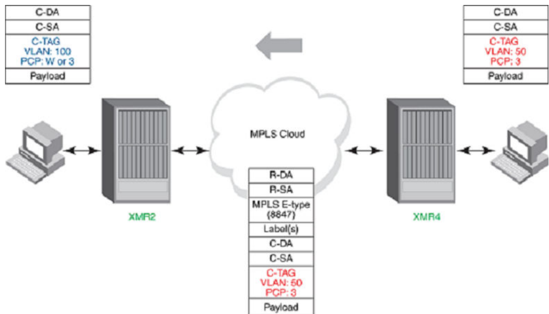
FIGURE 56 Sample configuration
