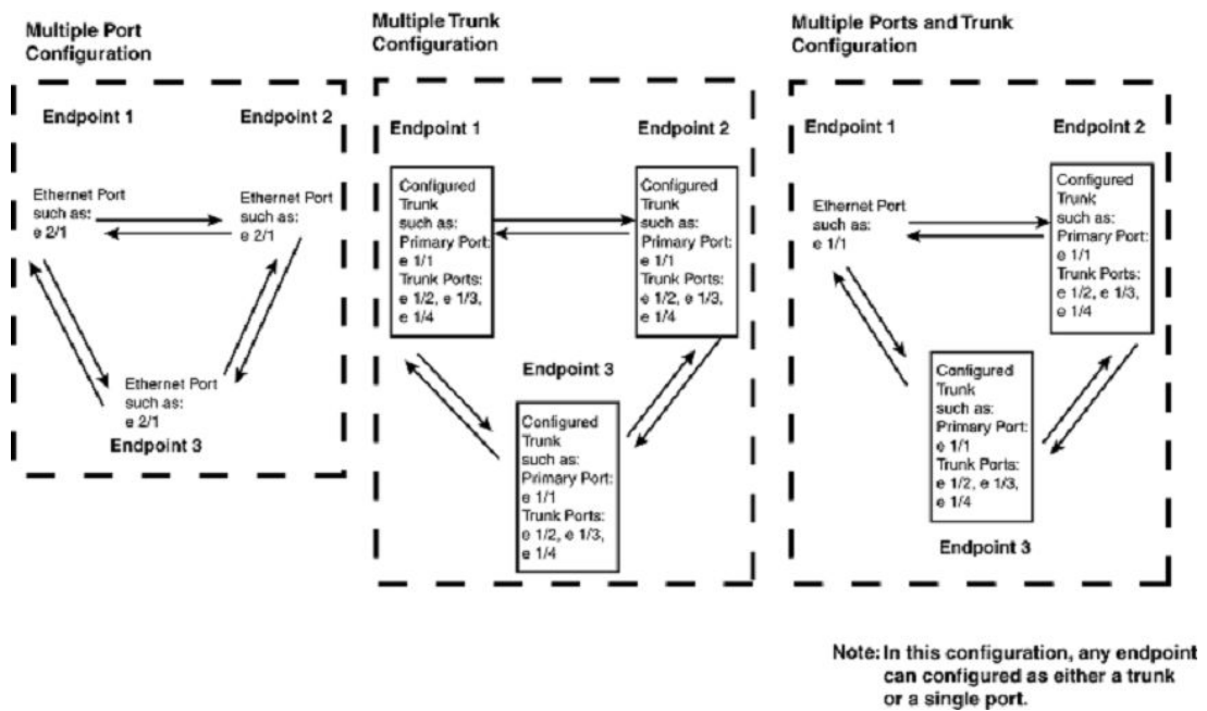
FIGURE 57 Local VPLS port and LAG configurations
