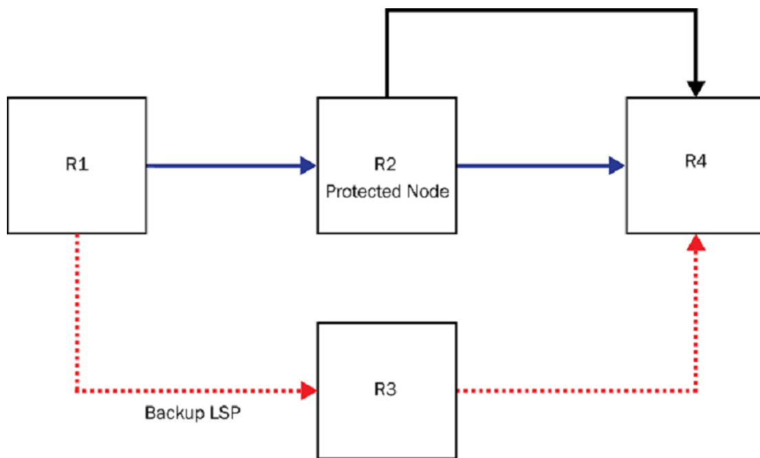
FIGURE 23 Node protection
