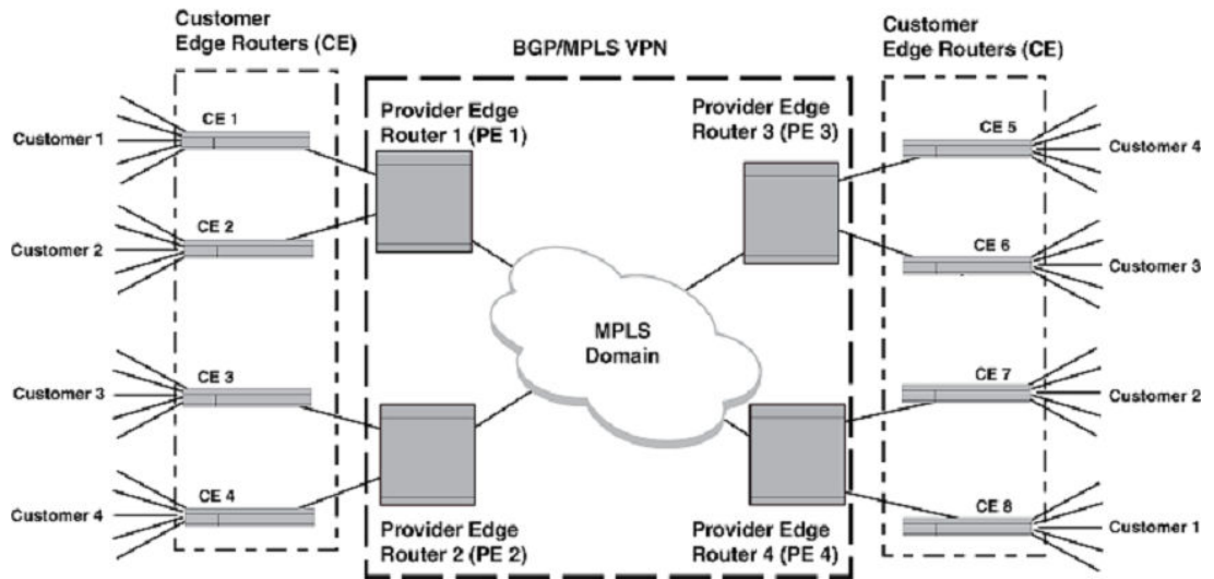
FIGURE 68 BGP or MPLS VPN network
