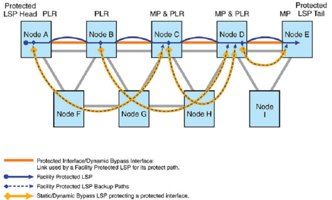
FIGURE 24 Protected dynamic bypass interface
