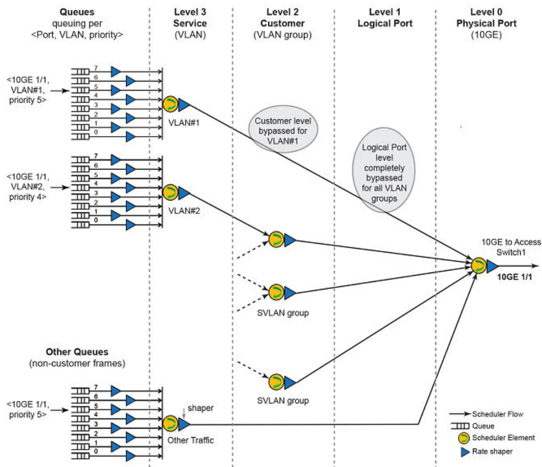
FIGURE 12 Bypassing hierarchy levels example
