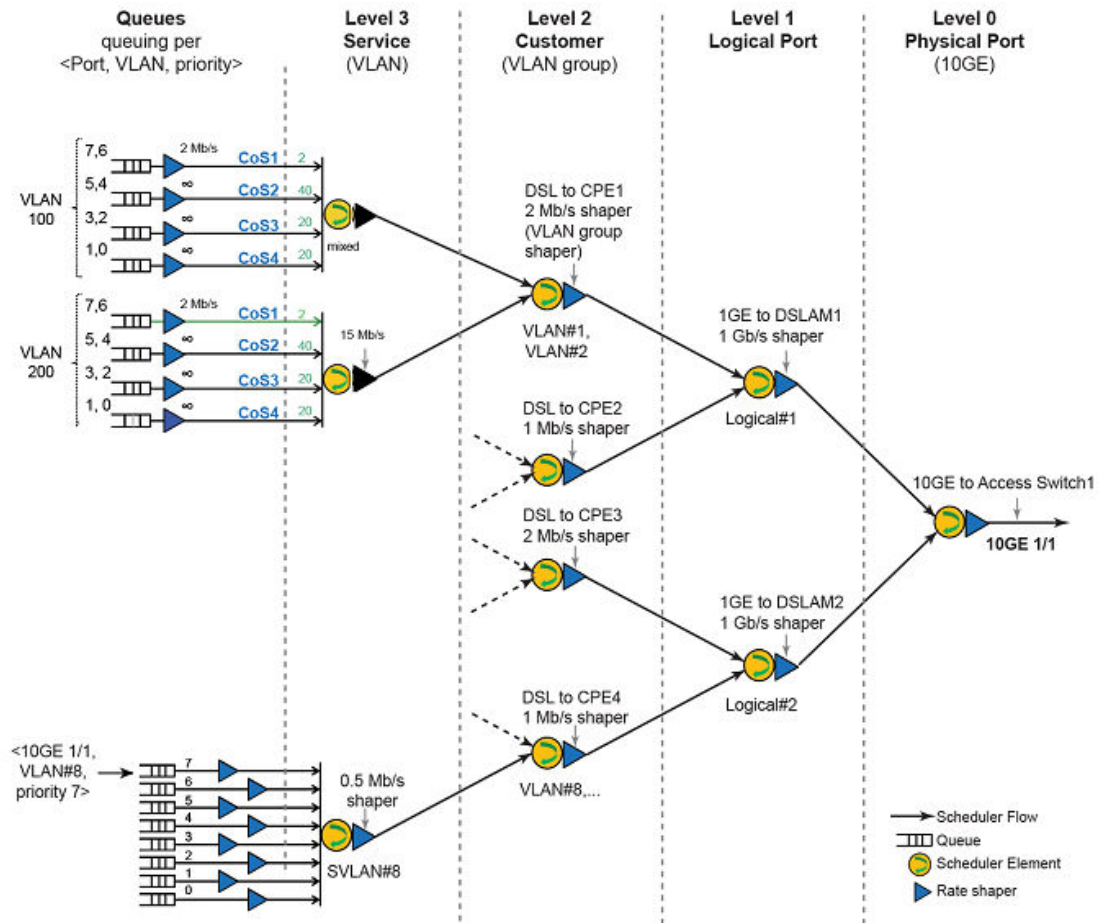
FIGURE 14 HQoS example
