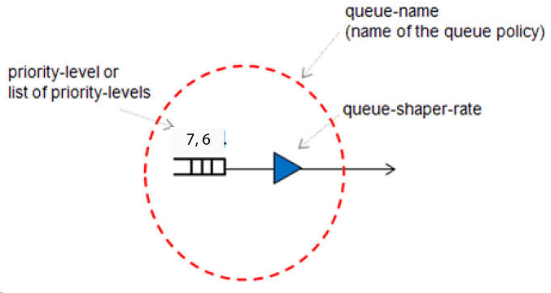
FIGURE 17 H-QoS Queue Policy
