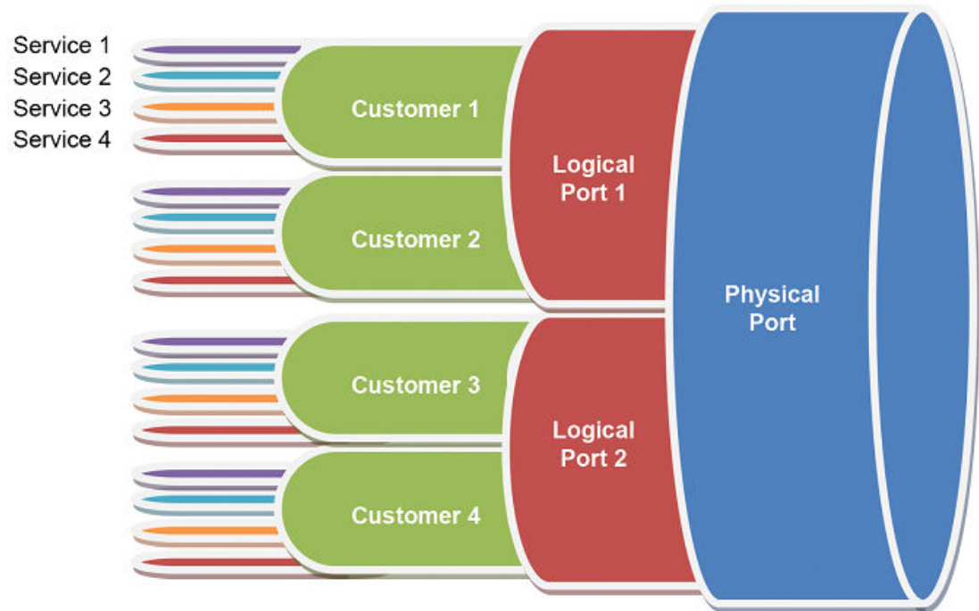
FIGURE 7 HQoS model
