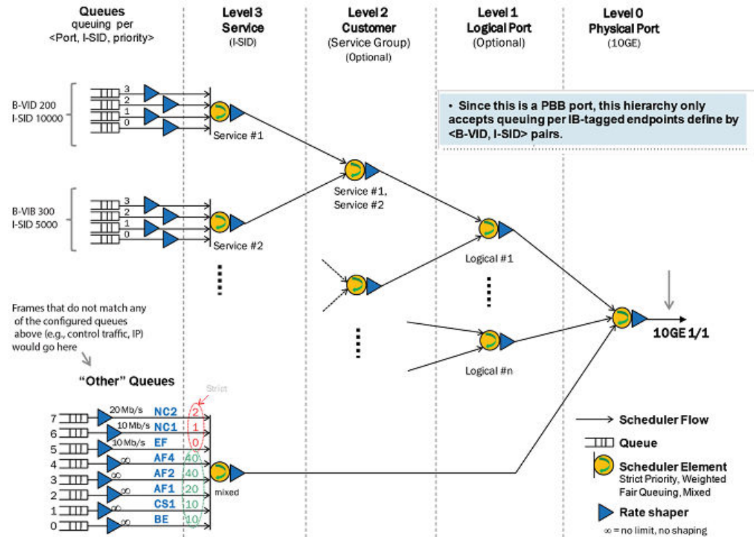
FIGURE 11 PBB HQoS example
