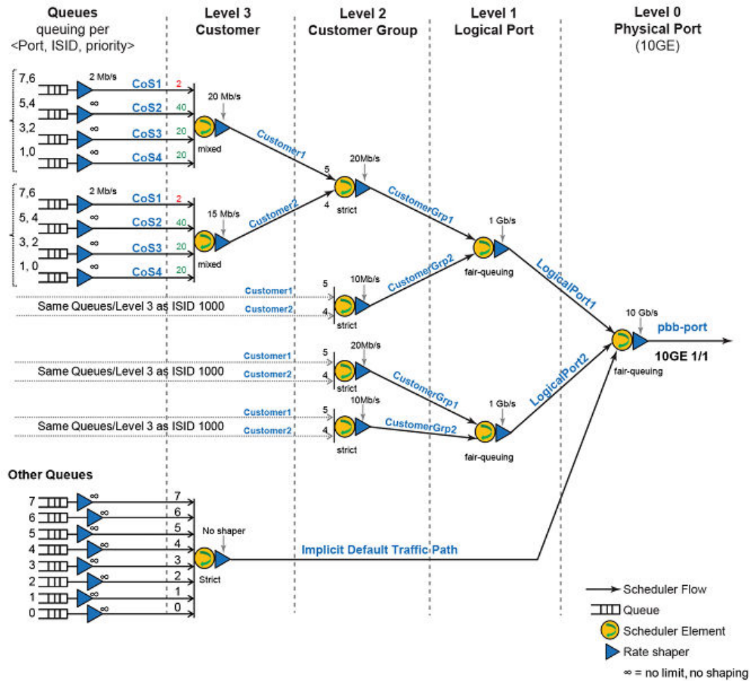
FIGURE 20 PBB HQoS deployment example
