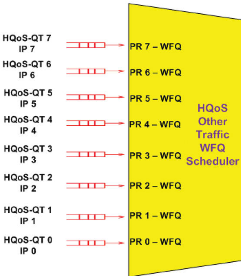
FIGURE 22 WFQ/FQ scheduling model for HQoS other traffic
