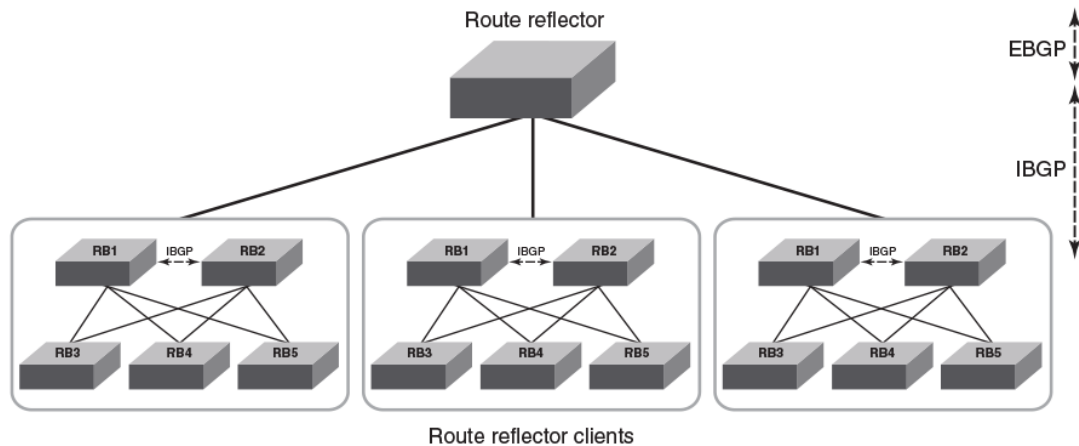
FIGURE 15 BGP route-reflector server and clients
