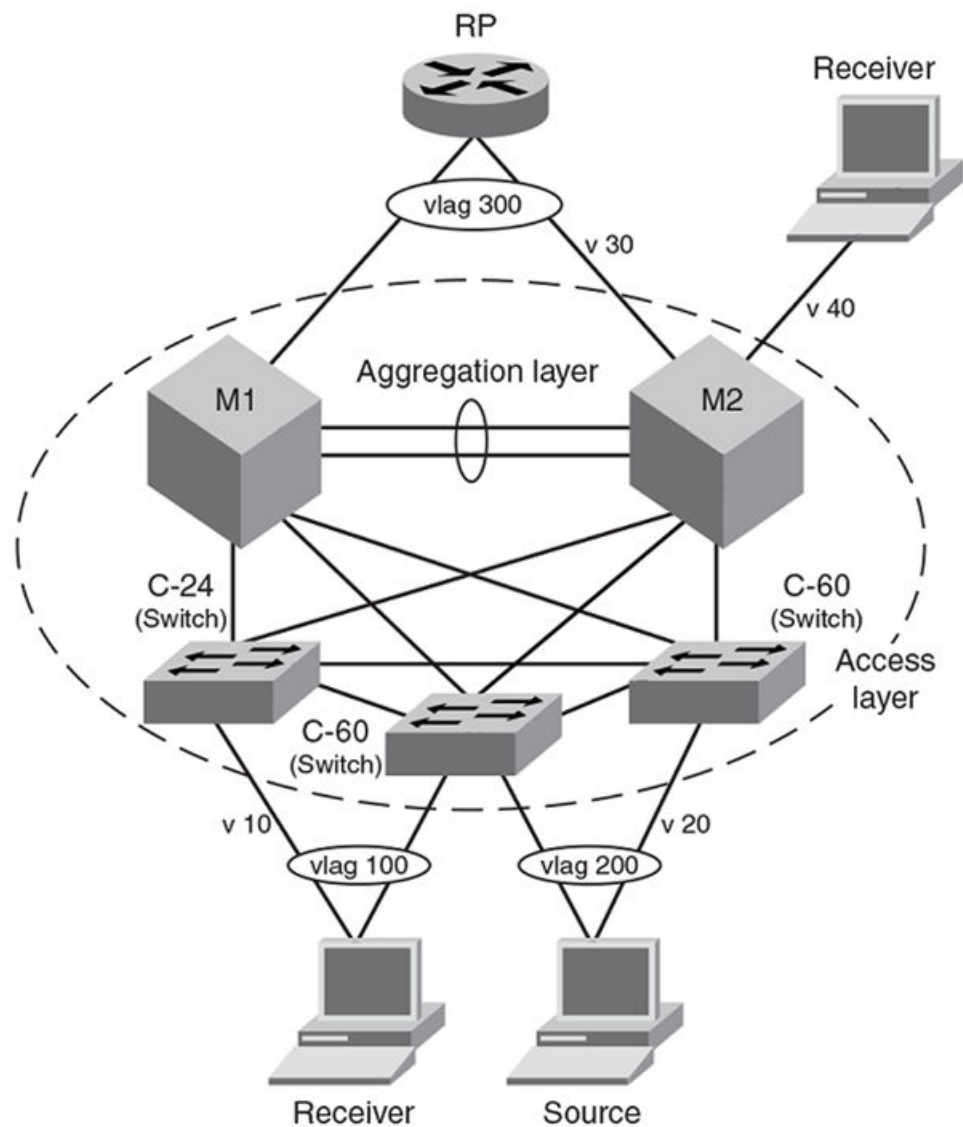
FIGURE 3 Example deployment using single VCS
