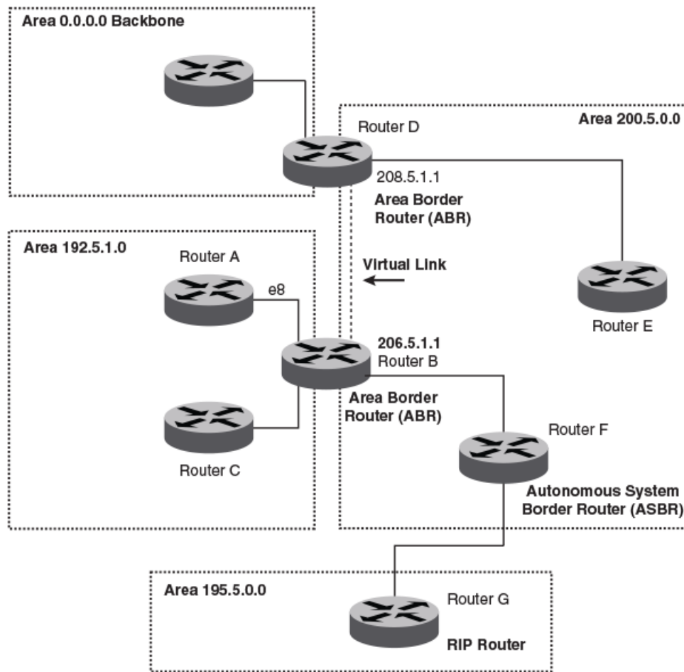
FIGURE 4 OSPF operating in a network
