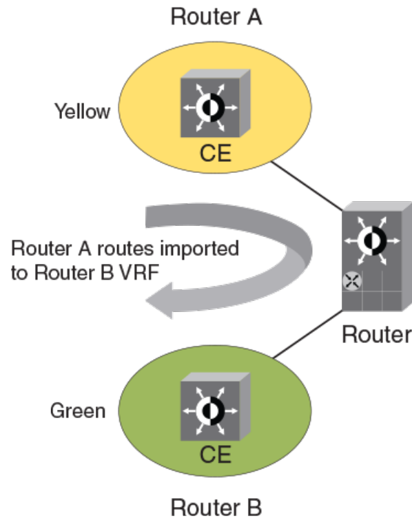
FIGURE 26 Dynamic Inter-VRF route leaking
