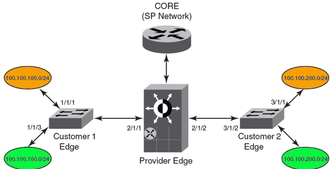
FIGURE 23 VRF topology
