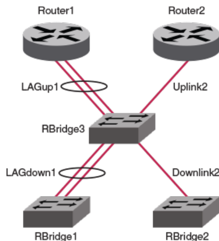
FIGURE 37 Multiple downlink/uplink topology
