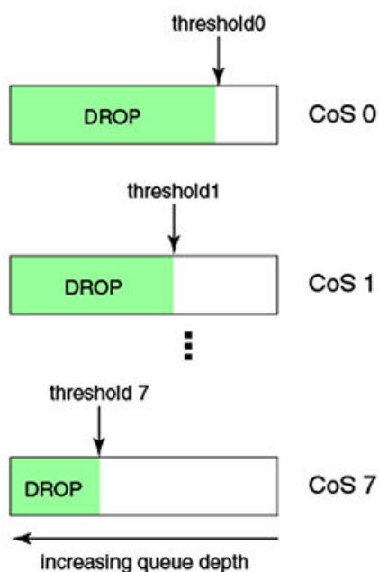
FIGURE 29 Queue depth
