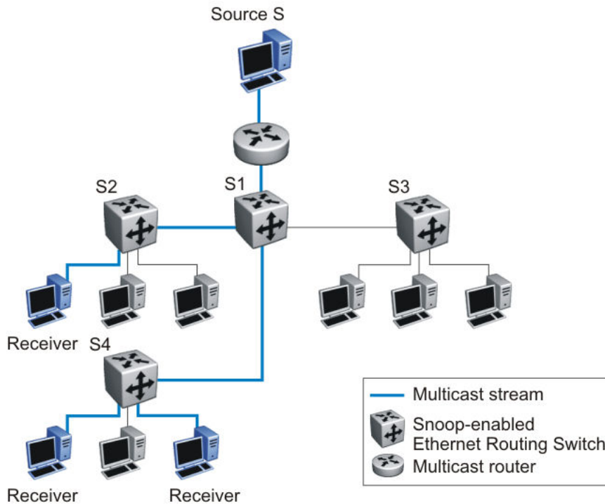
Figure 14: Ethernet Routing Switch running IGMP snooping
