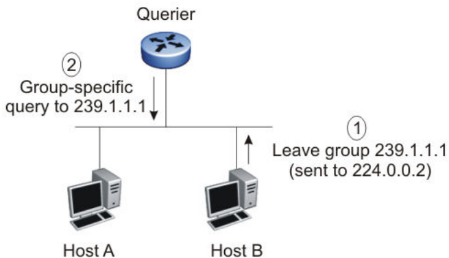
Figure 11: IGMPv2
