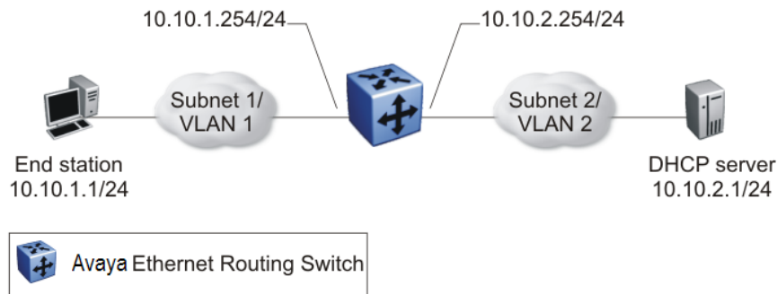
Figure 6: Forwarding DHCP packets
