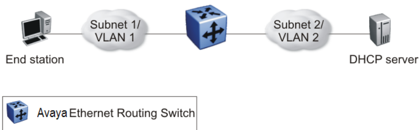
Figure 5: DHCP relay operation
