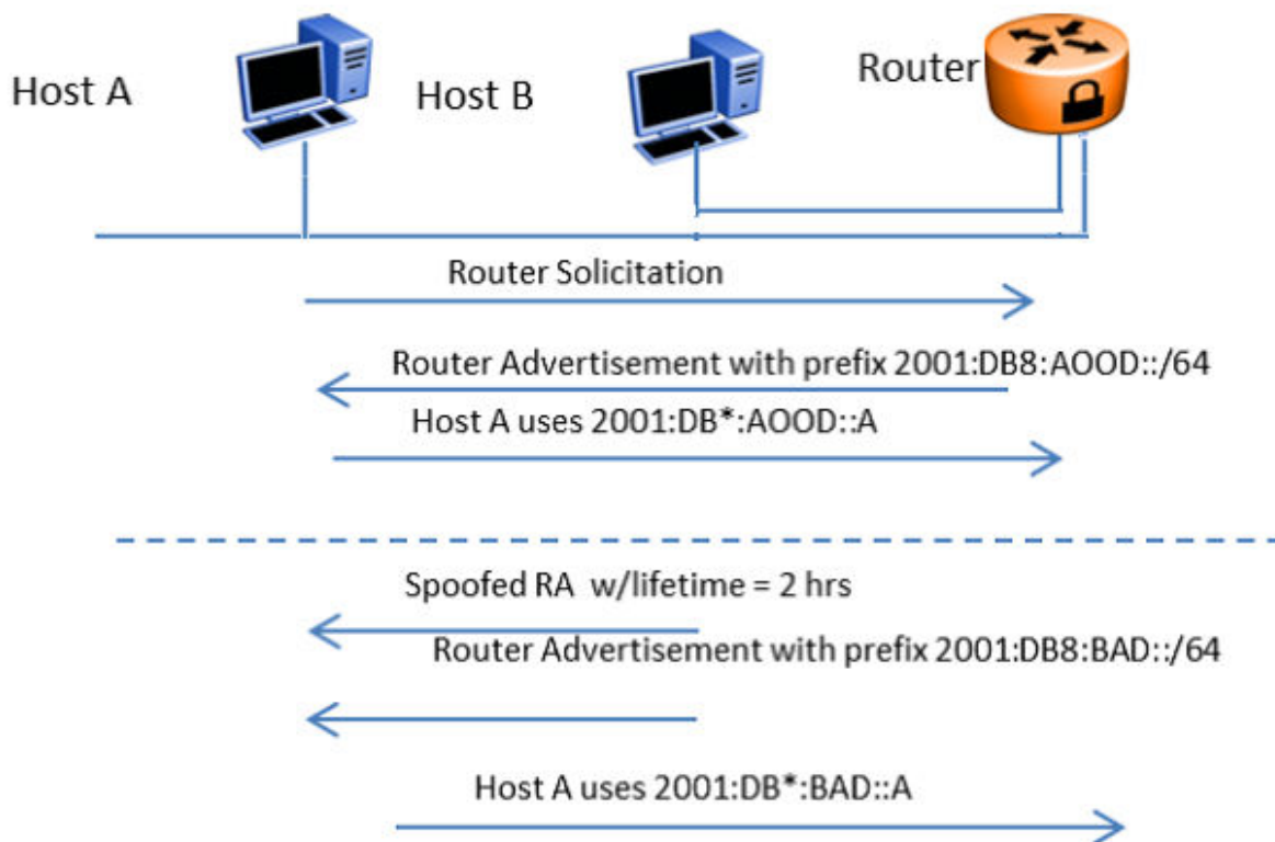
Figure 5: Stateless Address Autoconfiguration
