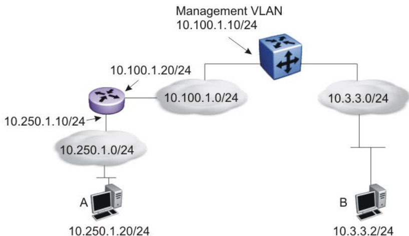
Figure 5: Management route
