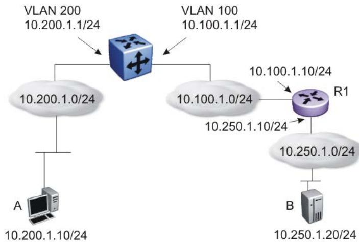
Figure 3: Static routes
