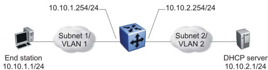
Figure 7: Forwarding DHCP packets
