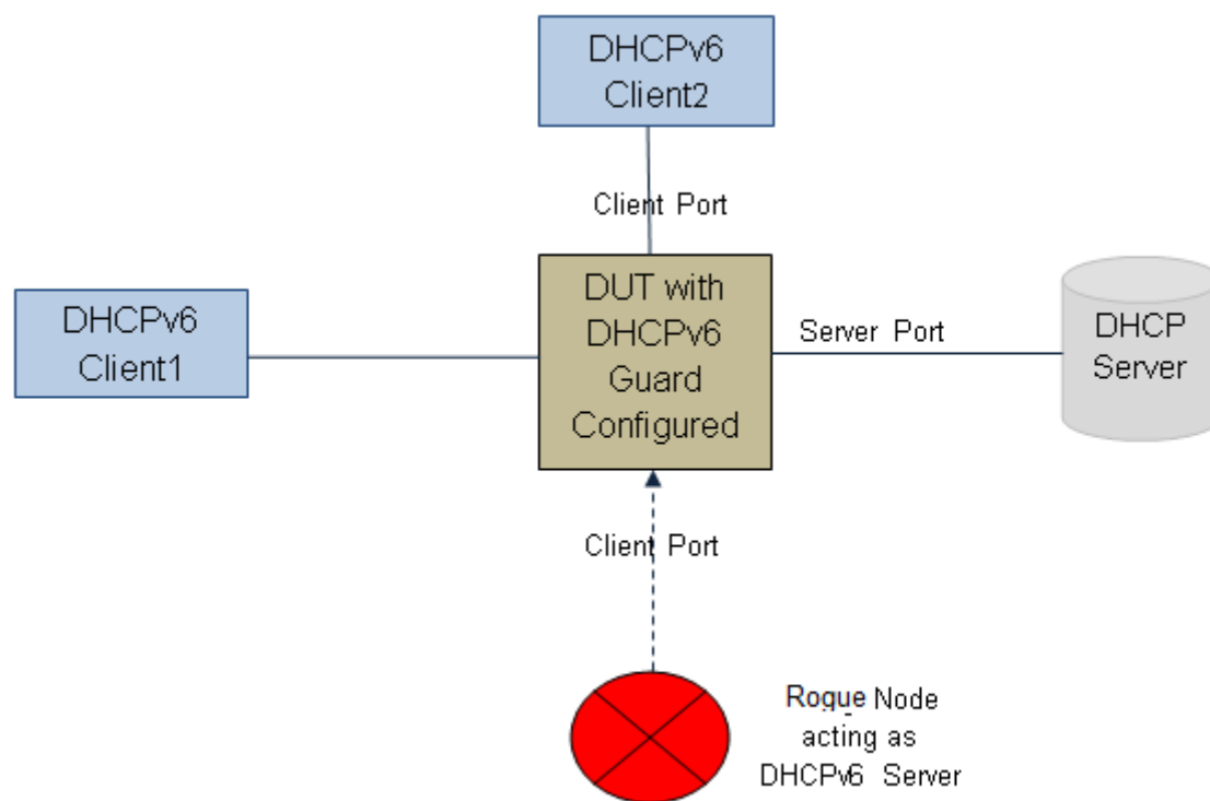
Figure 9: DHCPv6 Topology 1
