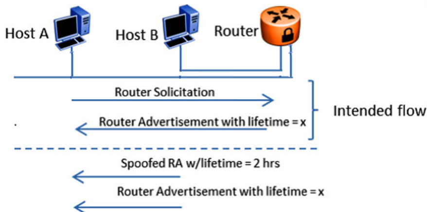
Figure 4: Message Flow IPv6 Router Discovery
