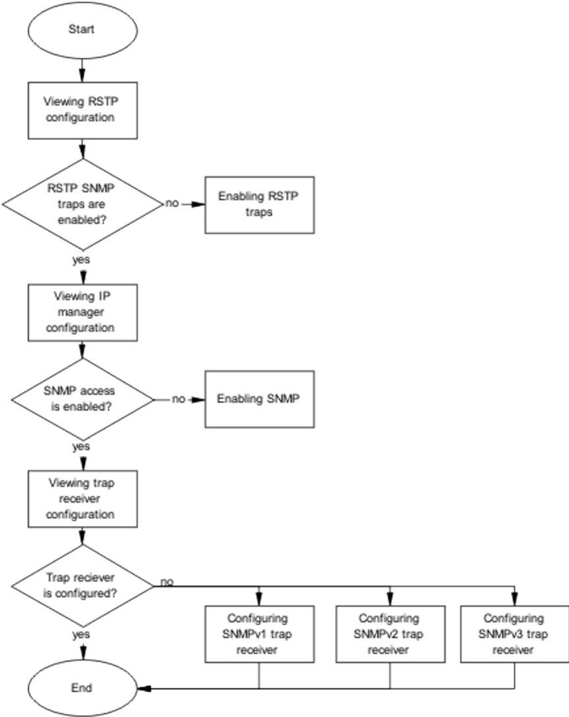
Figure 80: Task flow: No RSTP SNMP traps are received
