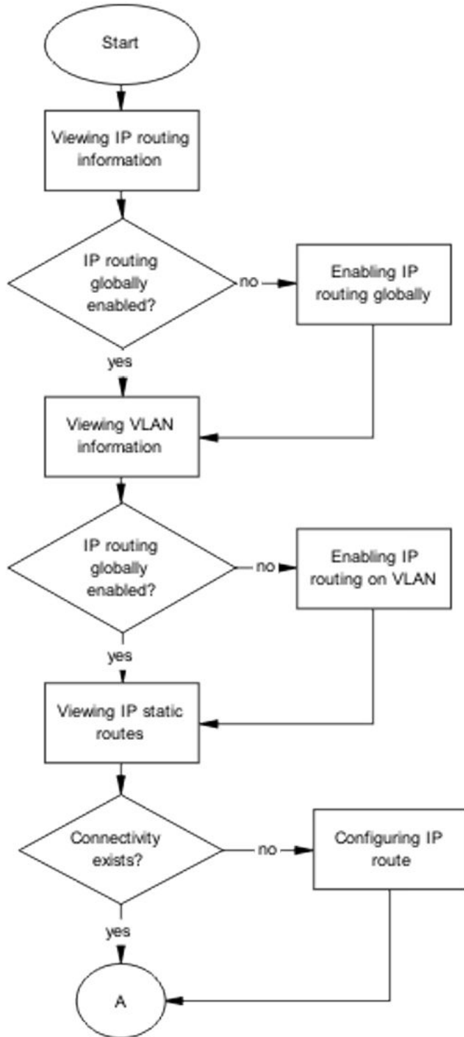
Figure 83: Task flow: Bootp/DHCP requests from clients do not reach Bootp/DHCP server part 1
