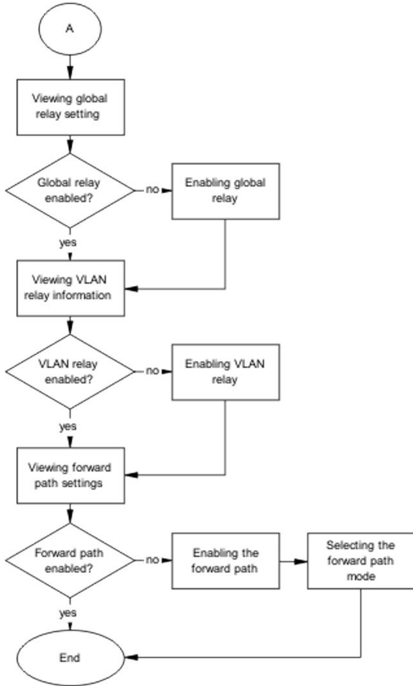
Figure 84: Task flow: Bootp/DHCP requests from clients do not reach Bootp/DHCP server part 2
