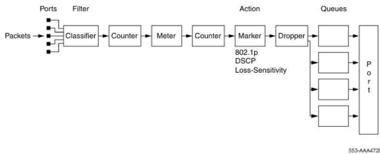
Figure 1: QoS Policy Schematic
