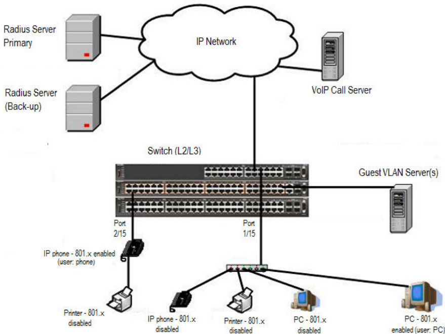
Figure 44: MHSA authentication mode (Guest VLAN option enabled) with or without RADIUS additional attributes with or without Multihost MultiVLAN
