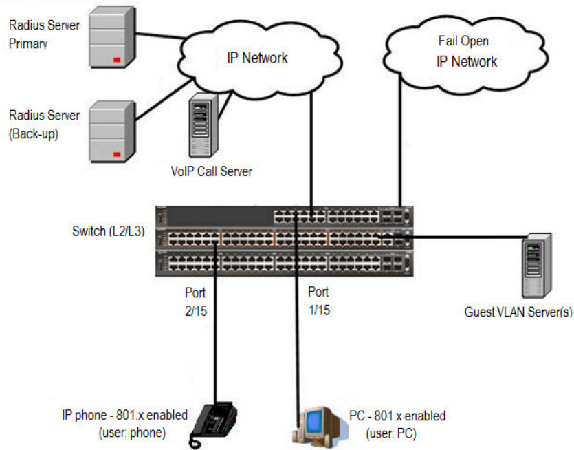
Figure 42: SSHA authentication mode (with Guest VLAN and Fail Open VLAN enabled) with or without RADIUS additional attributes with or without Multihost MultiVLAN
