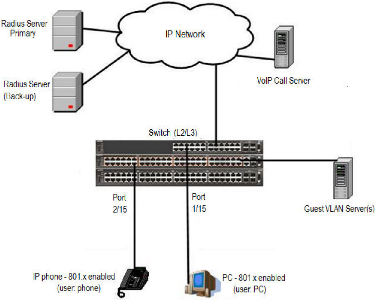
Figure 41: SHSA authentication mode (with Guest VLAN enabled) with or without RADIUS additional attributes, with or without Multihost MultiVLAN
