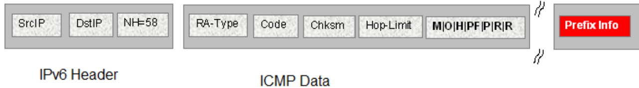
Figure 14: IPv6 ICMP RA data packet outline
