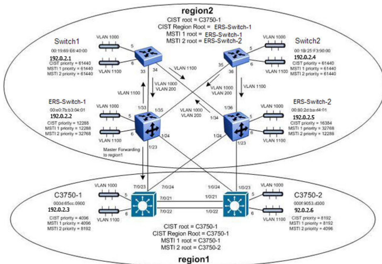
Figure 43: MSTP Example with Two Regions
