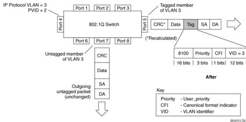
Figure 6: 802.1Q tagging (after policy-based VLAN assignment)
