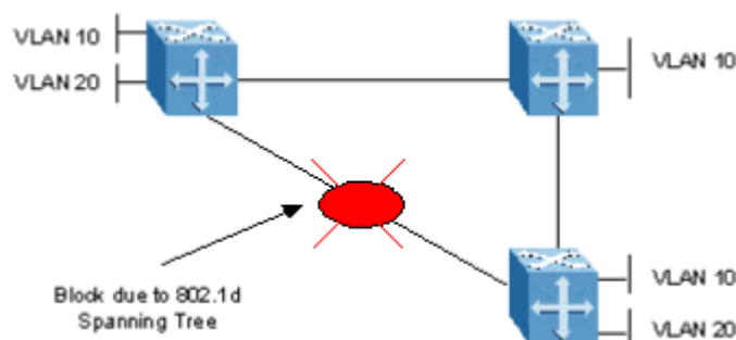
Figure 27: 802.1d spanning tree
