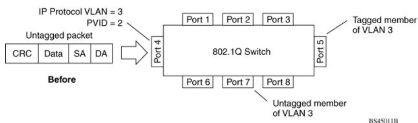
Figure 5: Policy-based VLAN assignment
