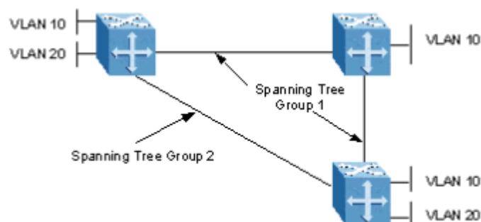
Figure 28: Multiple instances of spanning tree
