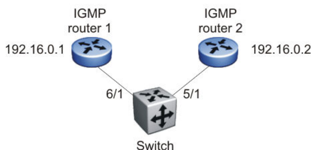
Figure 14: Static mrouter port and nonquerier
