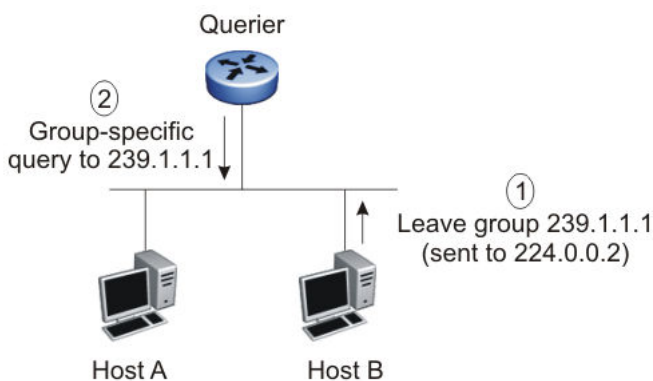
Figure 9: IGMPv2
