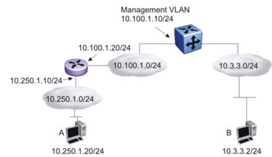
Figure 4: Management route
