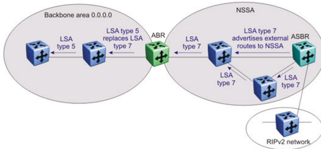
Figure 25: OSPF NSSA
