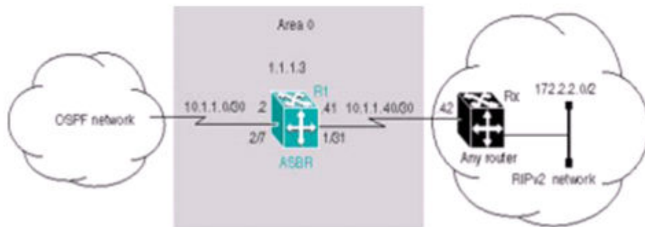
Figure 32: ASBR distribution example
