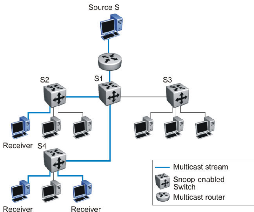
Figure 12: Switch running IGMP snooping
