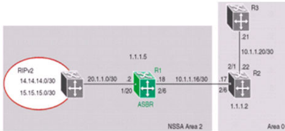
Figure 34: NSSA configuration example
