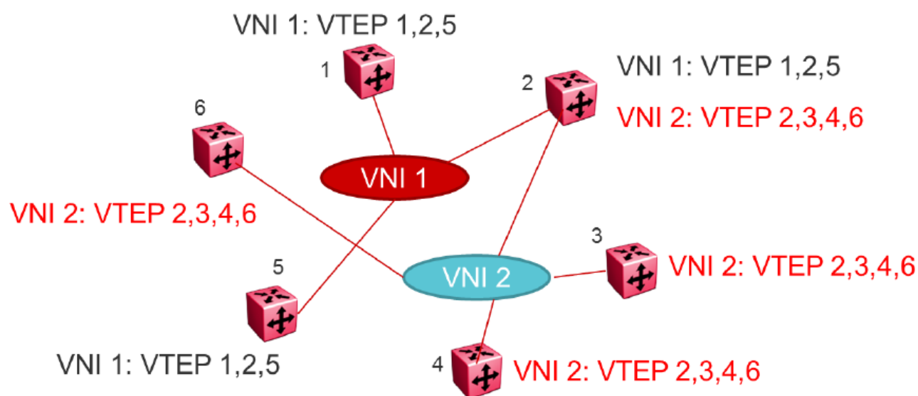
Figure 38: Example of the VXLAN Network topology
