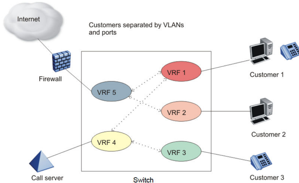
Figure 25: Inter-VRF forwarding
