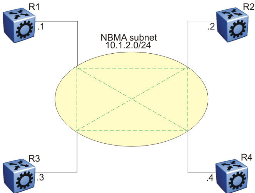
Figure 2: NBMA subnet
