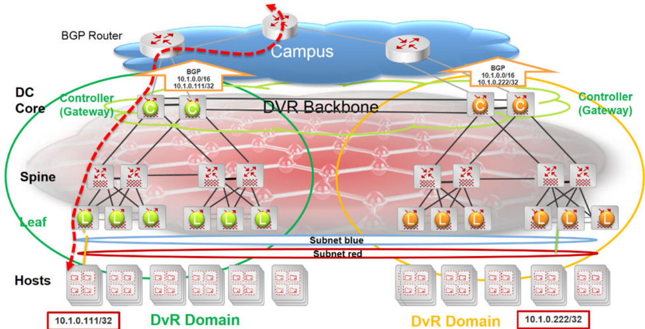
Figure 23: Traffic flow optimized with route redistribution
