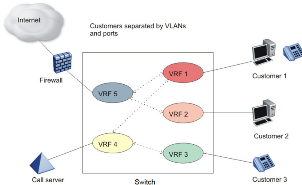
Figure 25: Inter-VRF forwarding
