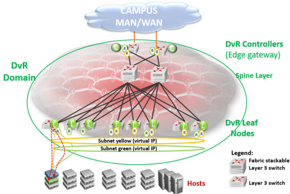
Figure 19: SPB Fabric network with central Layer 3 Controller and distributed Layer 3 datapath at the edges
