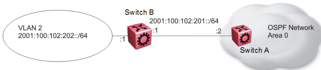
Figure 13: OSPFv3 configuration
