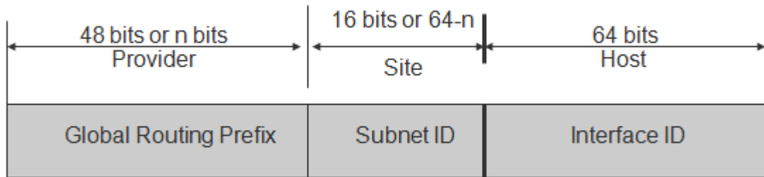
Figure 5: Unicast global address parts
