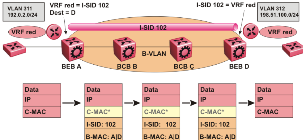
Figure 9: Packet forwarding in SPBM Layer 3 VSN
