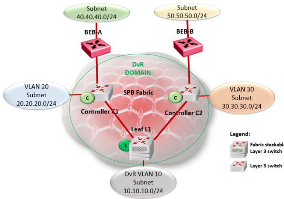
Figure 7: Redistribution of IPv4 local and static routes
