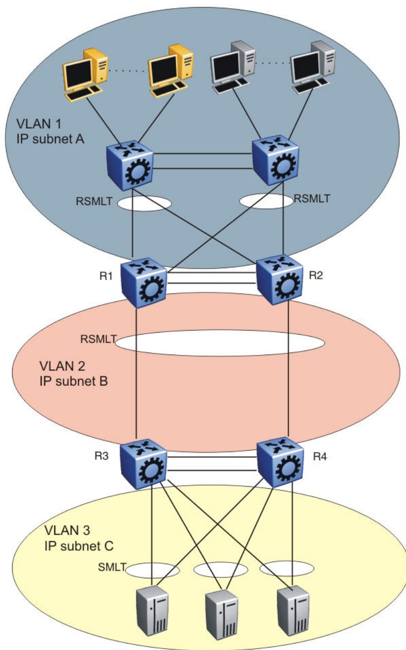
Figure 18: SMLT and RSMLT in Layer 3 environments
