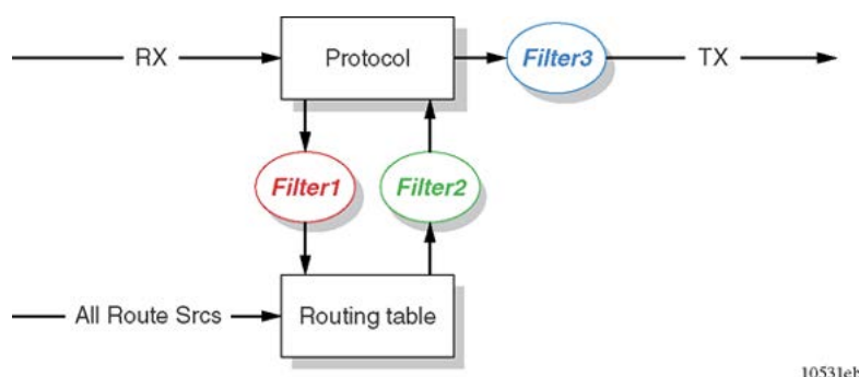
Figure 16: Route filtering stages
