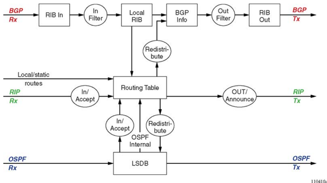
Figure 14: Route filtering for BGP, RIP, and OSPF routing protocols
