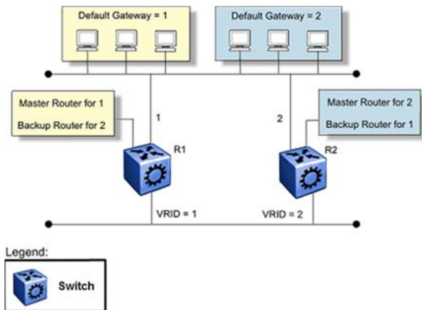
Figure 19: Virtual Router Redundancy Protocol configuration
