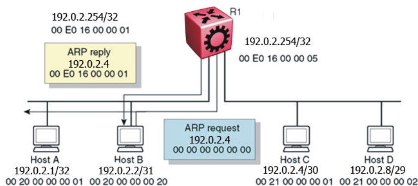
Figure 11: Proxy ARP operation
