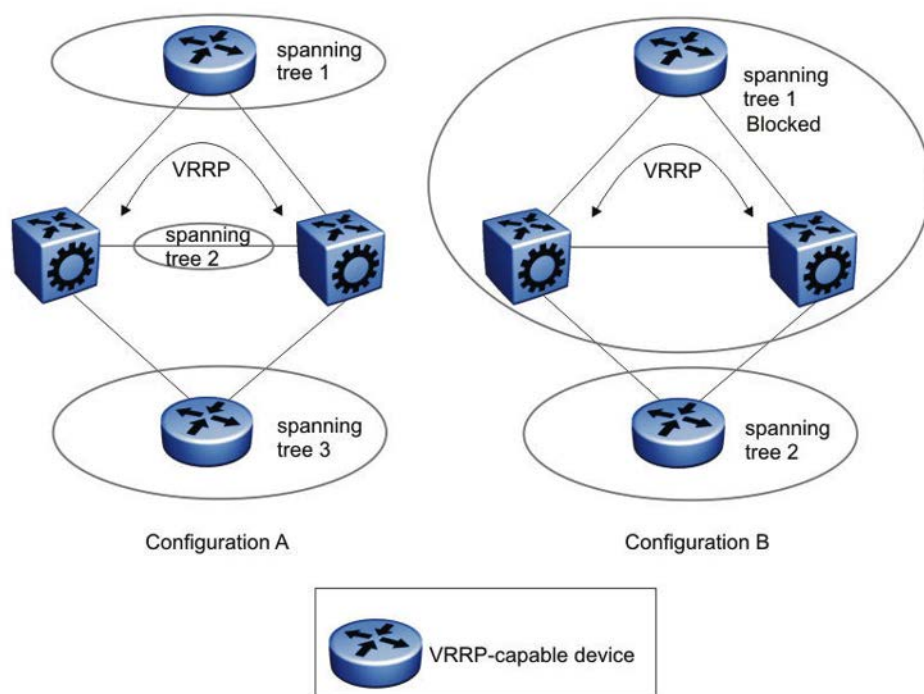
Figure 22: VRRP and STG configurations
