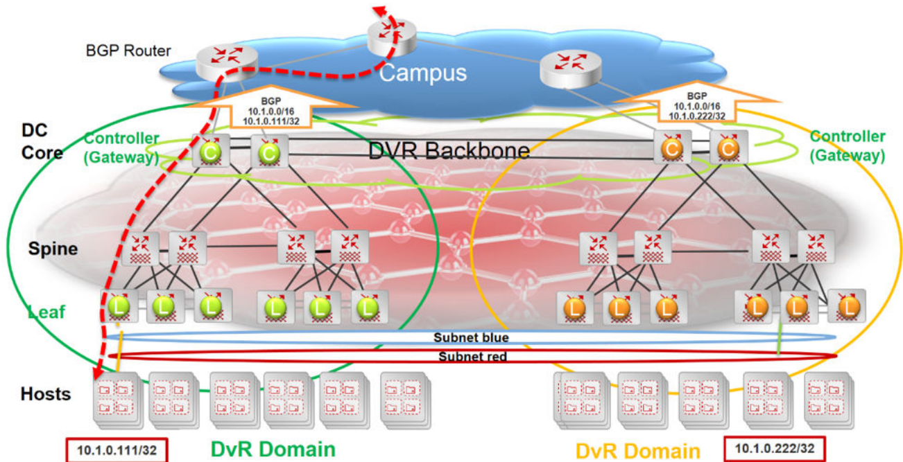
Figure 9: Traffic flow optimized with route redistribution
