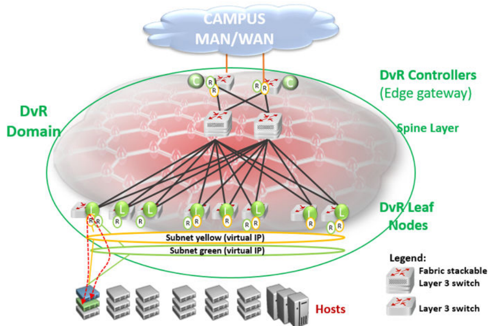
Figure 5: SPB Fabric network with central Layer 3 Controller and distributed Layer 3 datapath at the edges
