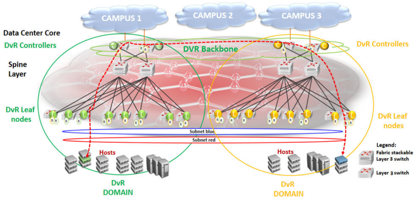
Figure 6: Shortest path routing between servers in different data centers
