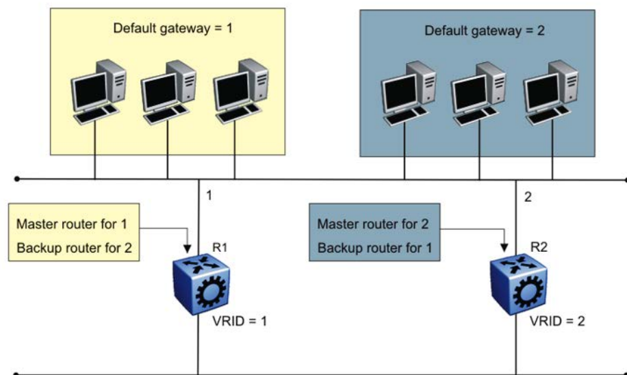
Figure 21: VRRP network configuration
