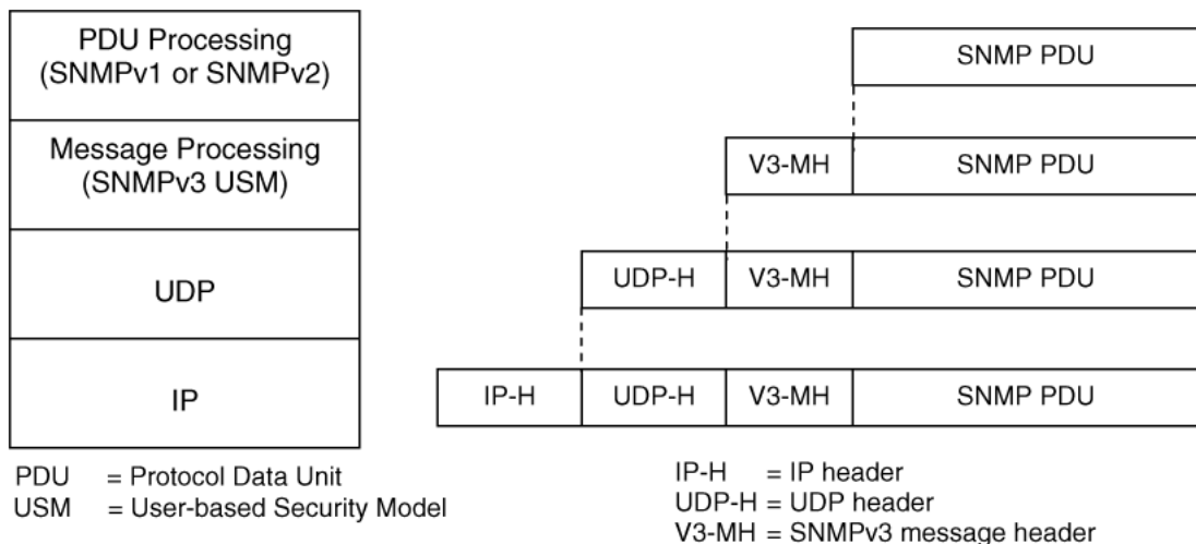
Figure 26: SNMPv3 USM
