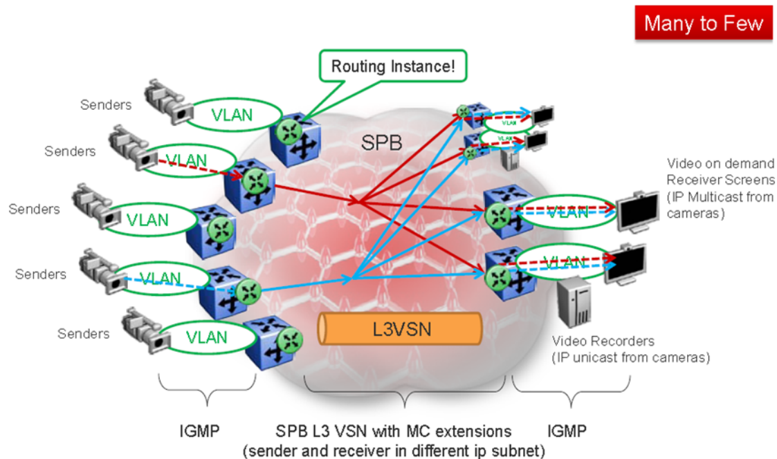
Figure 26: Deployment scenario — Routed video surveillance and IP camera deployment for transportation, airports, and government
