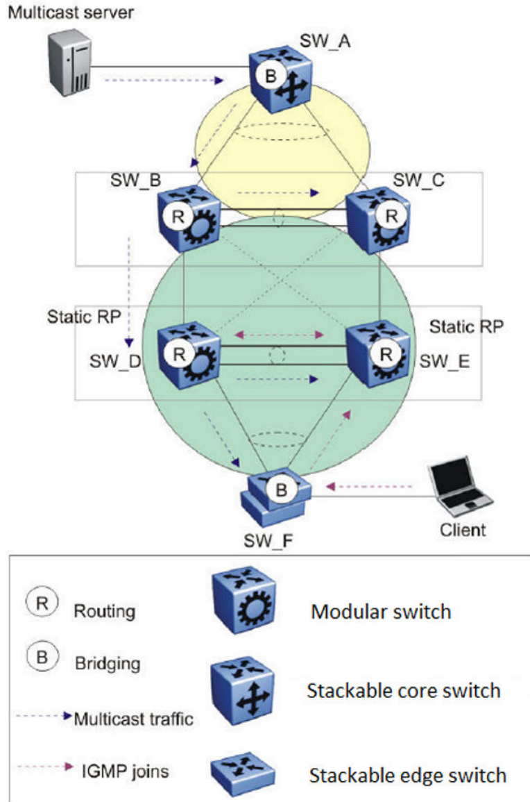
Figure 19: Multicast behavior in SMLT environment
