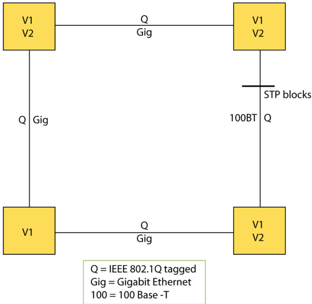
Figure 7: VLAN isolation
