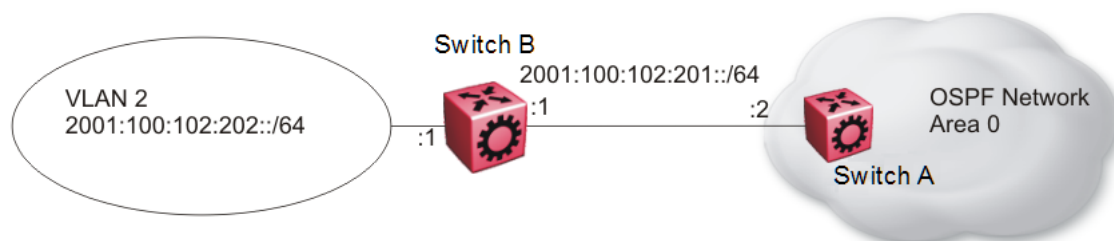
Figure 13: OSPFv3 configuration
