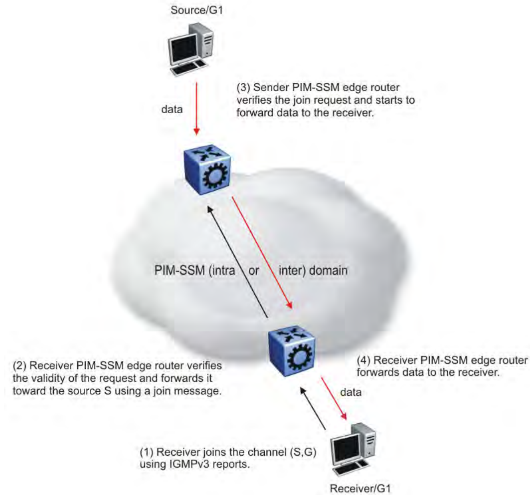
Figure 8: PIM-SSM architecture
