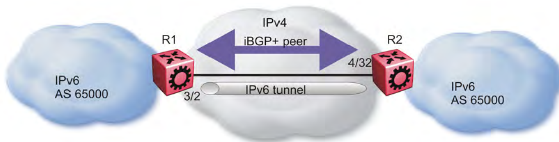
Figure 22: iBGP+ peers on CLIP interfaces with IPv6 tunneling
