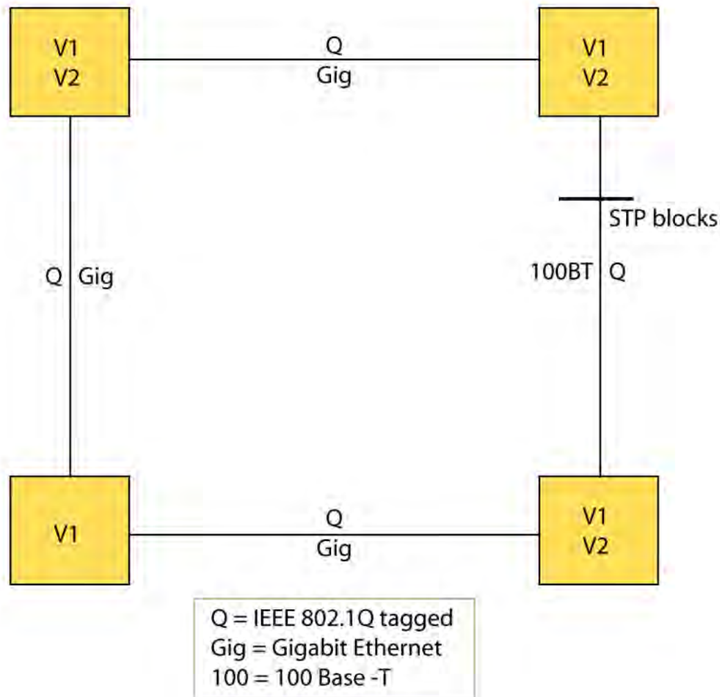
Figure 7: VLAN isolation
