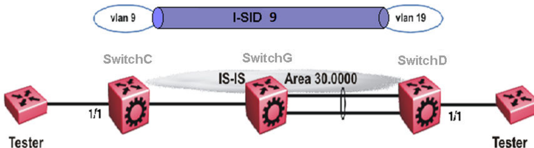
Figure 44: Layer 2 VSN with different VLAN IDs
