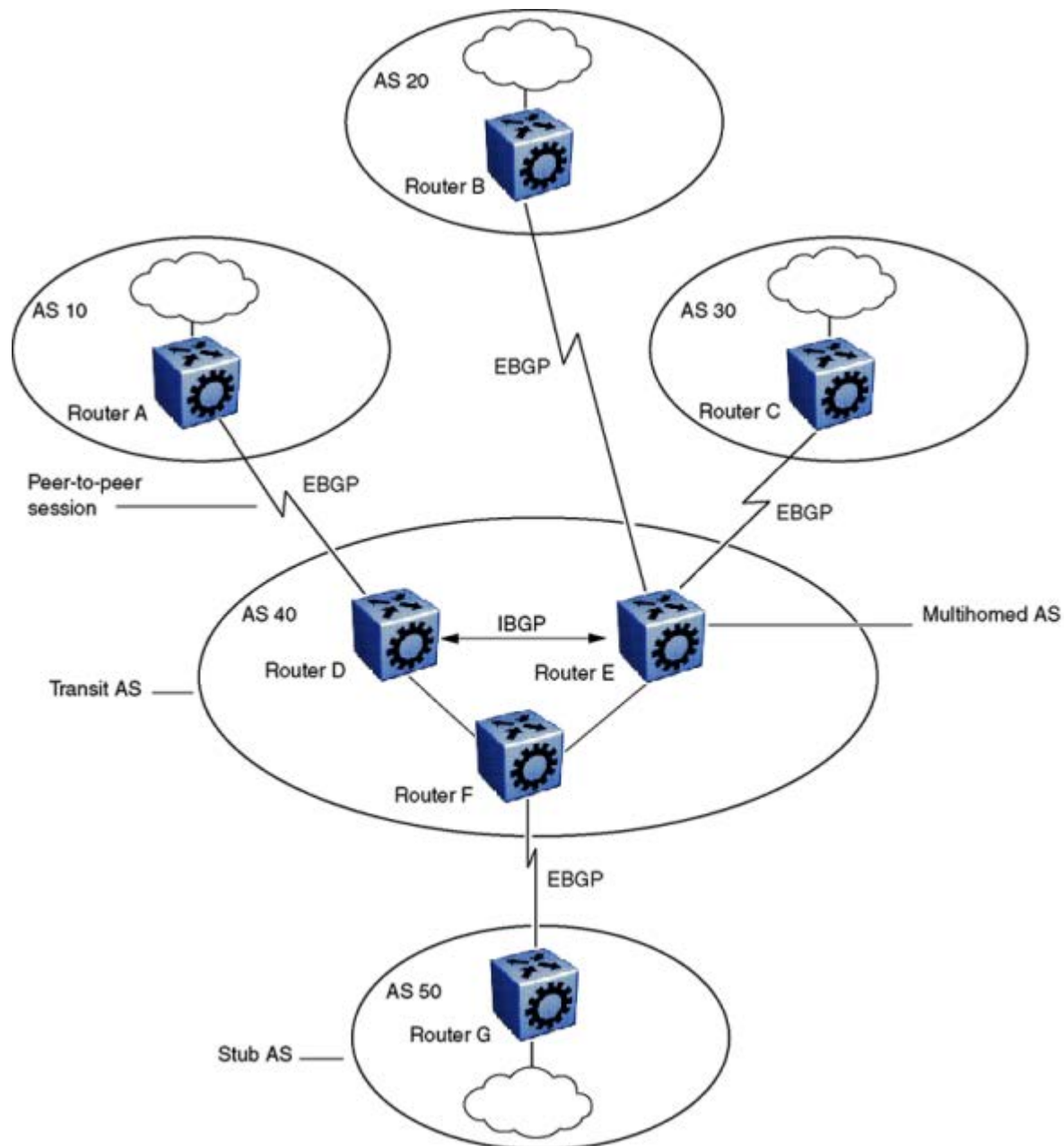
Figure 2: BGP networks
