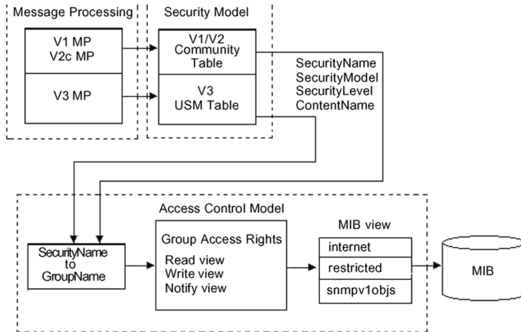
Figure 30: USM association with VACM
