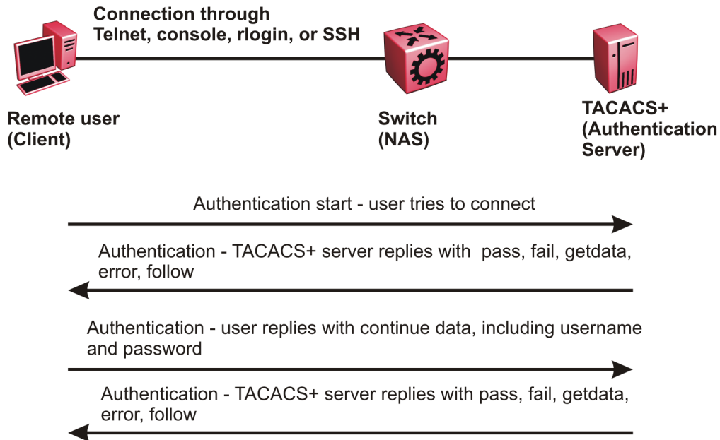
Figure 34: Authentication process
