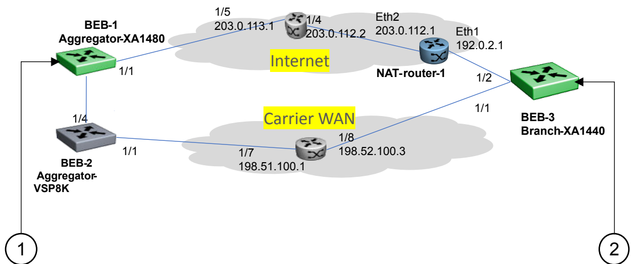
Figure 23: IPsec NAT-T with NAT router on one side
