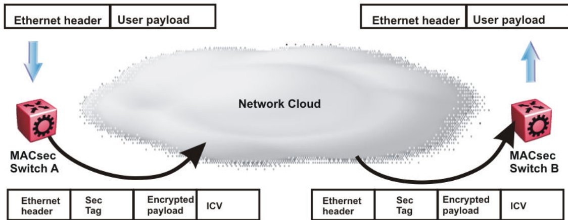
Figure 28: MACsec operation
