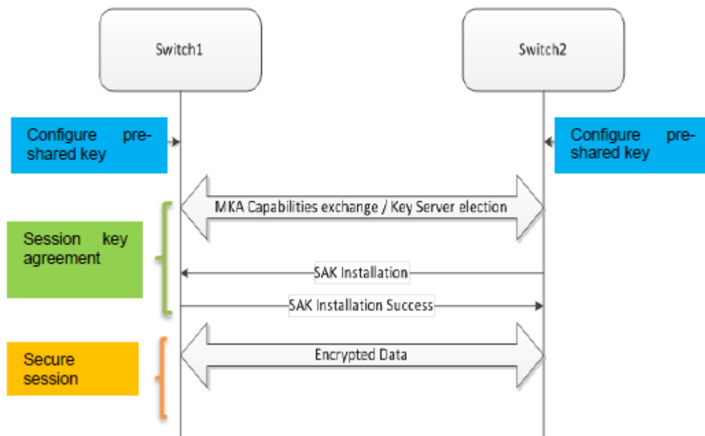
Figure 27: Switch to switch MACsec deployment scenario
