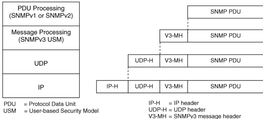
Figure 29: SNMPv3 USM
