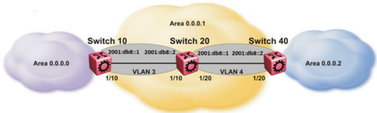
Figure 25: OSPFv3 virtual link with IPsec configuration
