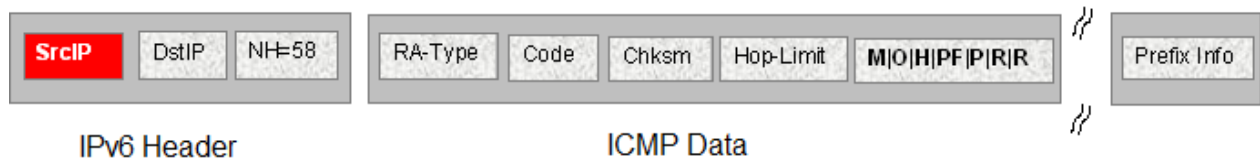
Figure 5: IPv6 ICMP RA Data Packet Online
