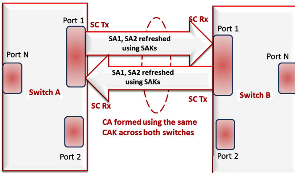
Figure 26: MACsec relationship
