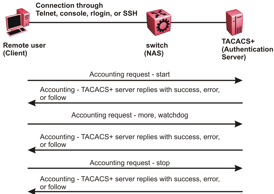
Figure 36: Accounting process
