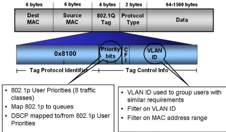
Figure 4: VLAN tag insertion
