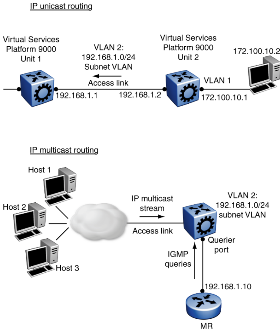
Figure 3: Incorrect use of an IP subnet-based VLAN
