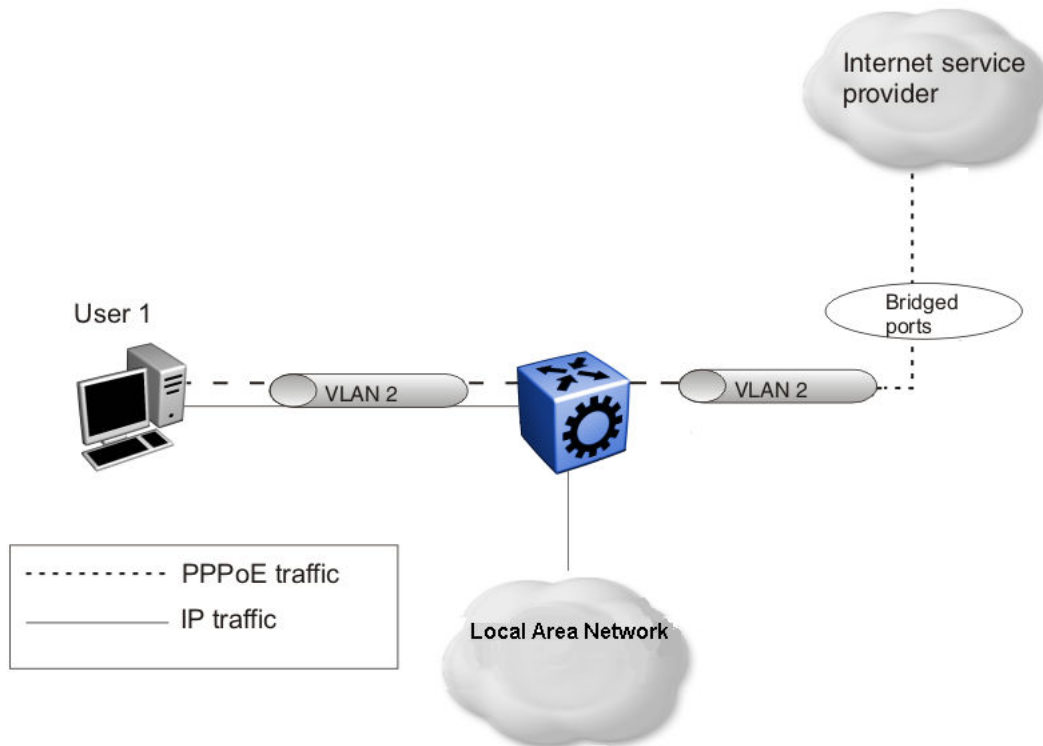
Figure 2: PPPoE and IP configuration
