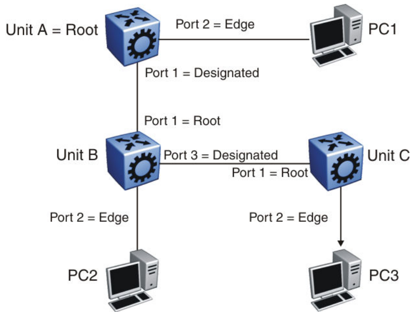
Figure 6: RSTP negotiation process
