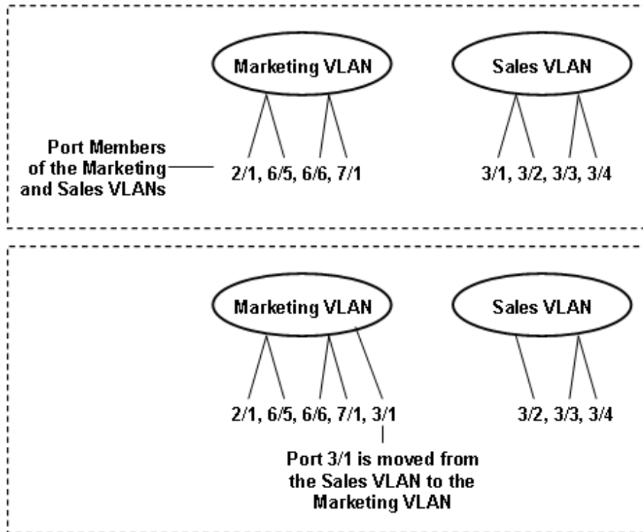
Figure 1: Port-based VLAN
