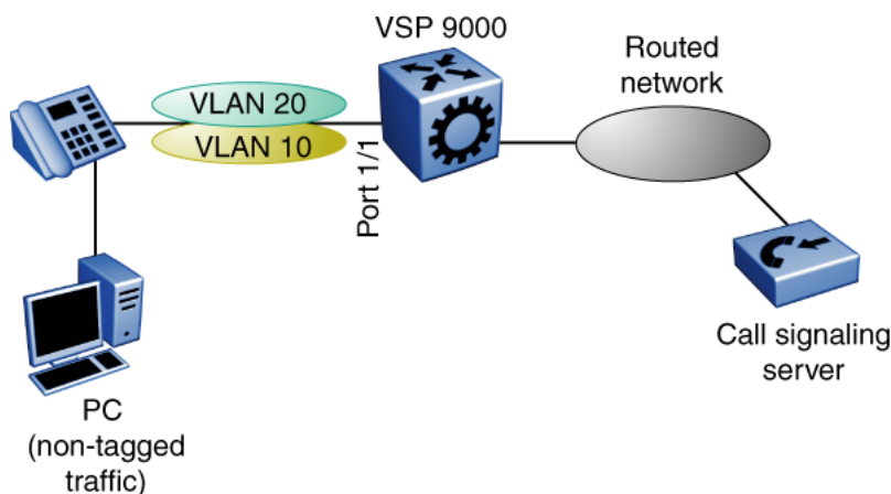
Figure 5: Network with IP phone and PC
