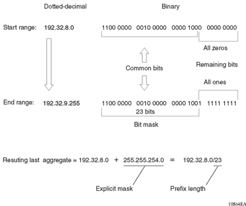
Figure 6: Last aggregate and prefix length
