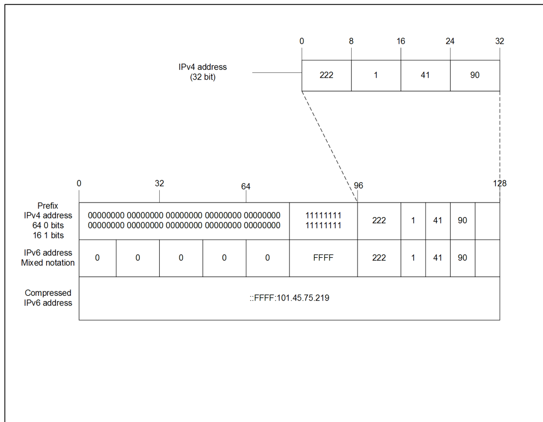
Figure 17: IPv4-mapped IPv6 address components
