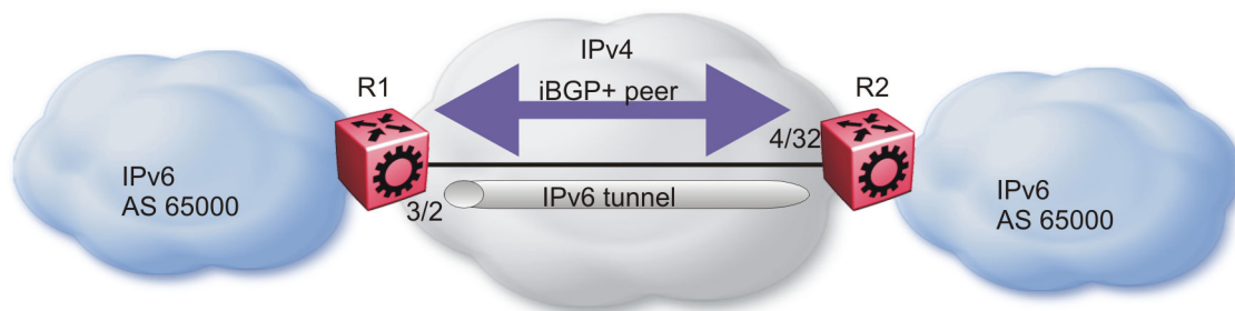
Figure 19: iBGP+ peers on CLIP interfaces with IPv6 tunneling
