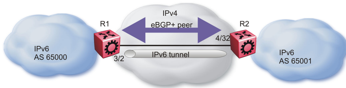
Figure 18: eBGP+ peers with IPv6 tunneling
