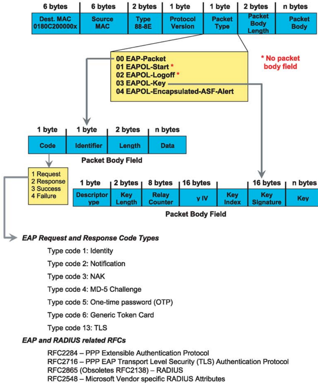
Figure 3: 802.1x Ethernet frame
