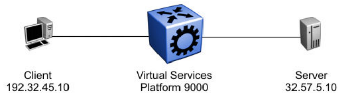
Figure 1: Reverse path checking network configuration
