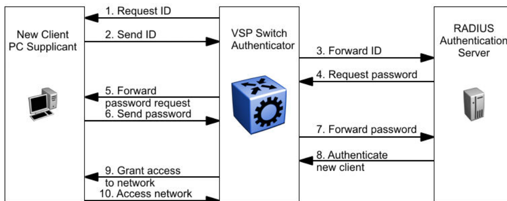
Figure 2: EAPoL configuration example
