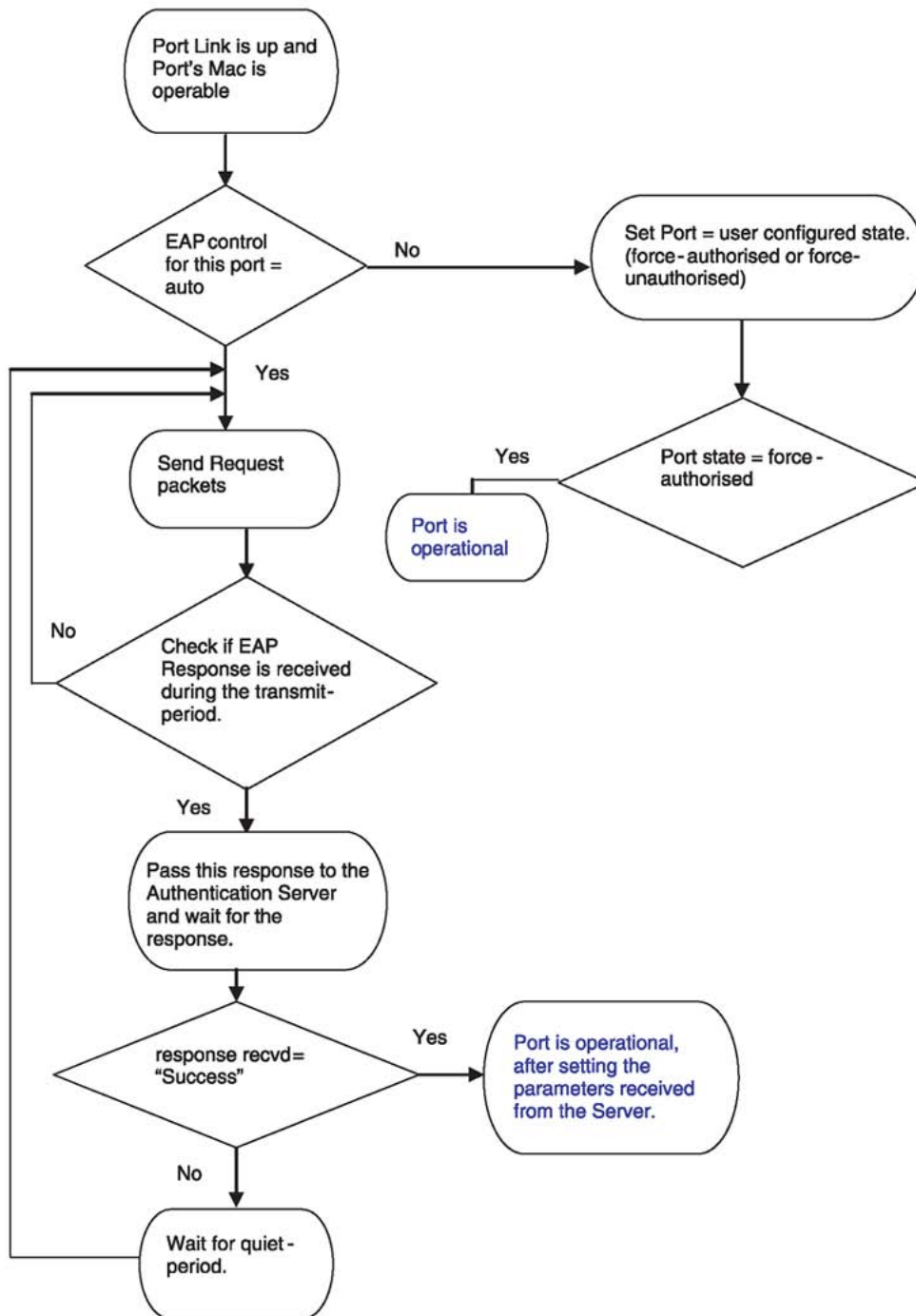
Figure 4: Virtual Services Platform 9000 EAPoL flow diagram
