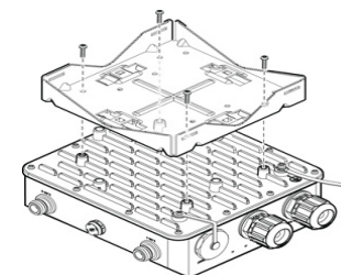
Figure 5 Attaching a Pole Bracket to the AP
