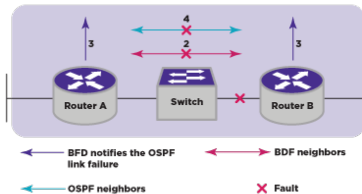
Figure 251: OSPFv3 Neighbor Relationship Eliminated by BFD Fault Detection
