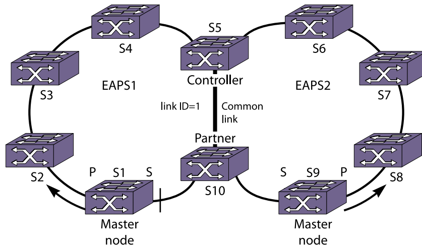
Figure 136: Multiple Rings Sharing a Common Link
