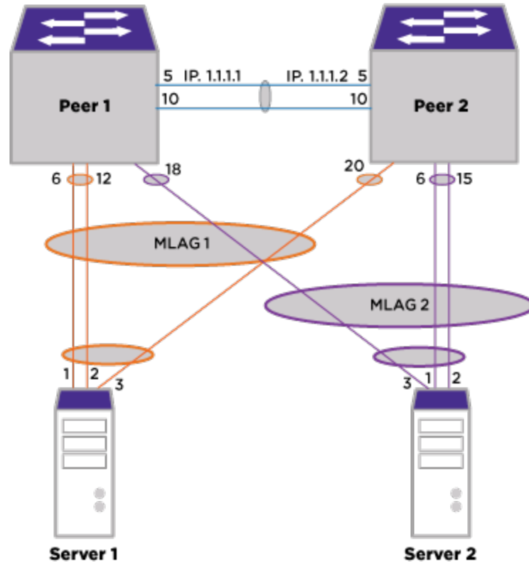
Figure 27: LACP Ports in MLAG Configuration
