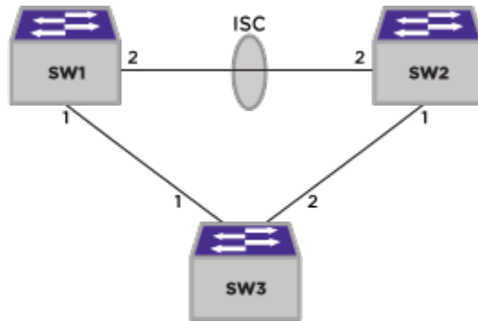
Figure 285: ELRP Egress Port Disable (2)
