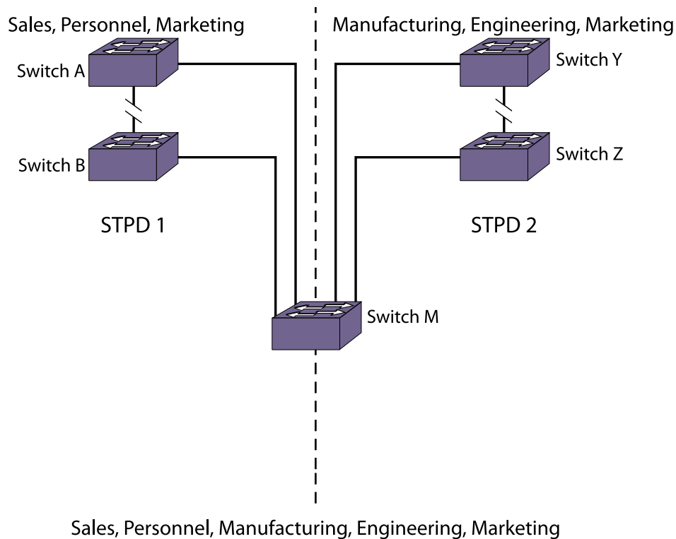
Figure 165: Multiple STPDs
