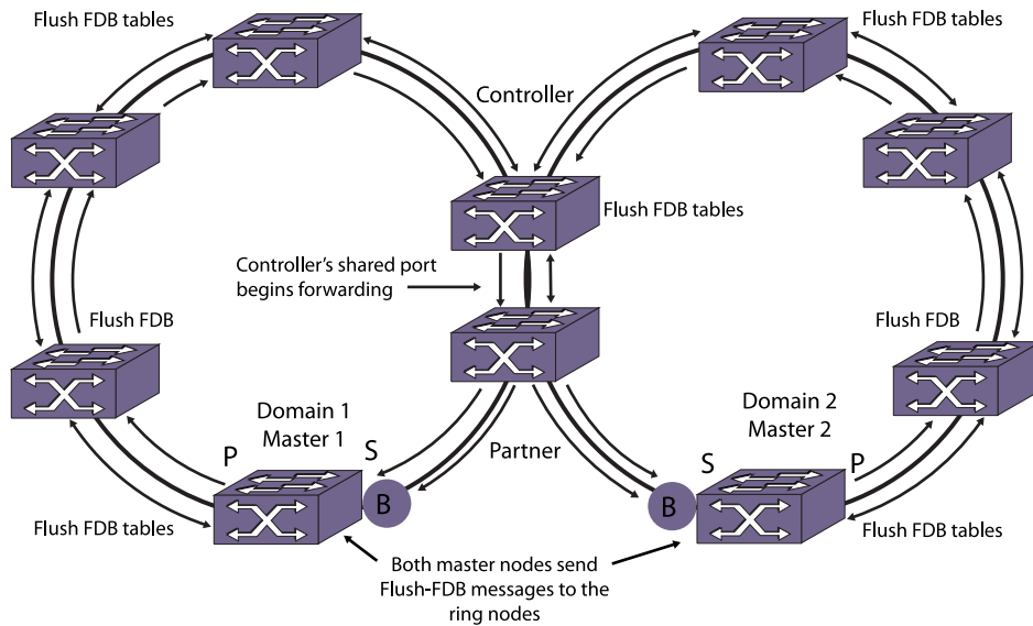
Figure 141: Common-Link Restored
