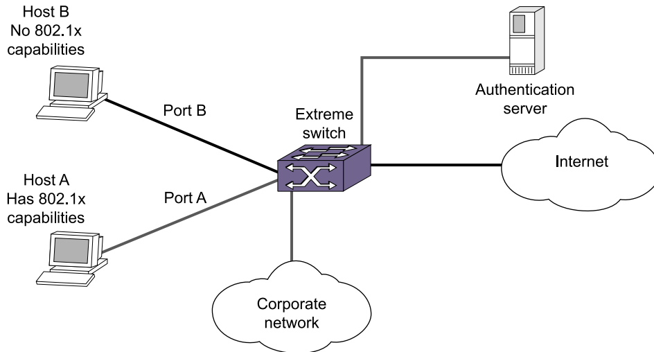
Figure 105: Guest VLAN for Network Login
