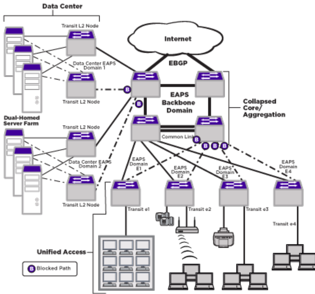
Figure 149: Extreme Networks EAPS Everywhere
