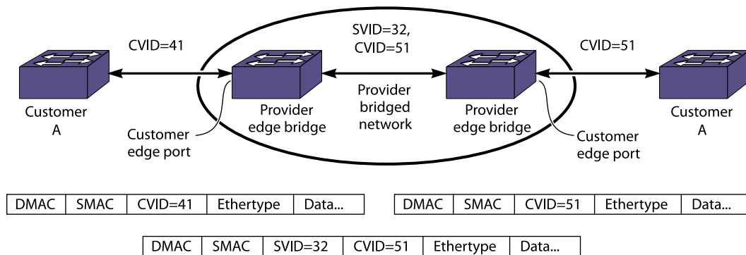
Figure 83: CVID Translation
