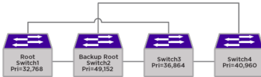
Figure 159: STP Root Bridge Loss Example
