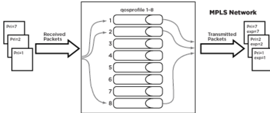
Figure 222: Mapping Dot1p to EXP Bits
