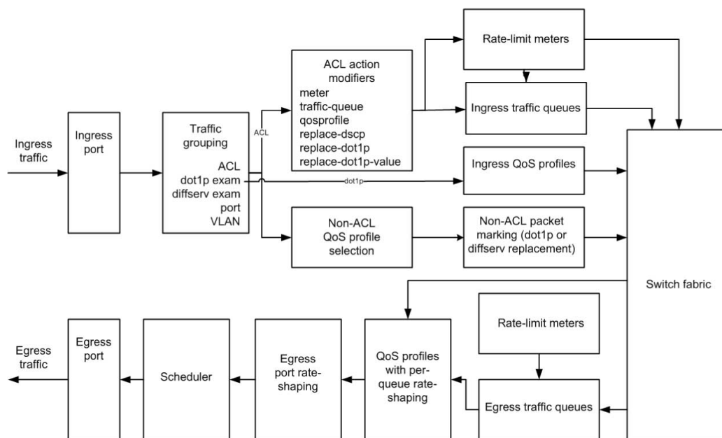
Figure 100: QoS on Extreme Networks Switches
