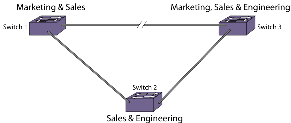
Figure 166: Incorrect Tag-Based STPD Configuration
