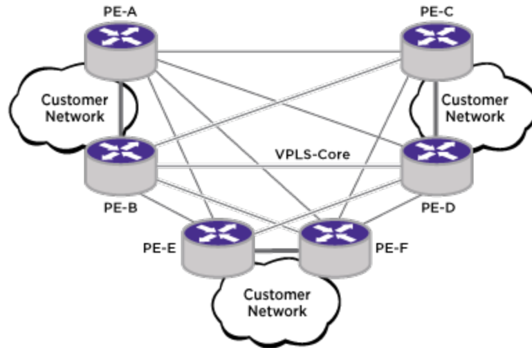
Figure 213: Example Protected Access VPLS Network
