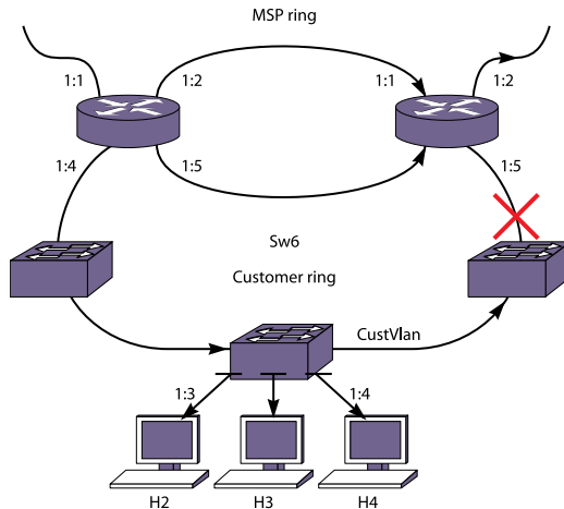
Figure 280: Inter-Multicast VLAN Forwarding
