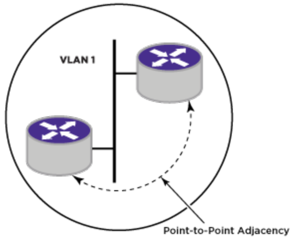
Figure 255: Point-to-Point Adjacency
