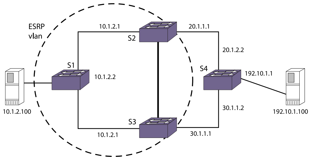
Figure 122: MAC Address Limits and VLANs Participating in ESRP
