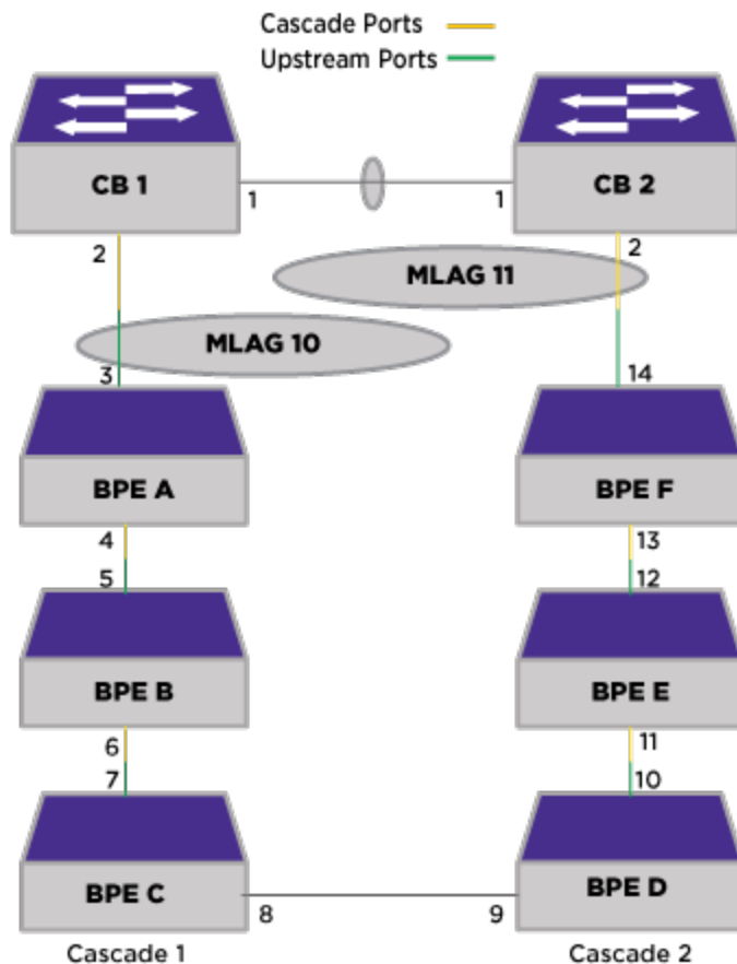
Figure 39: One-Arm MLAG
