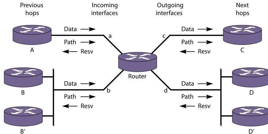
Figure 219: RSVP Messages
