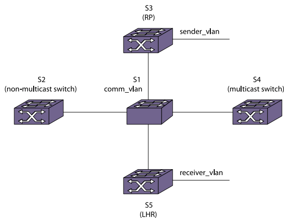
Figure 276: PIM Snooping Configuration Example
