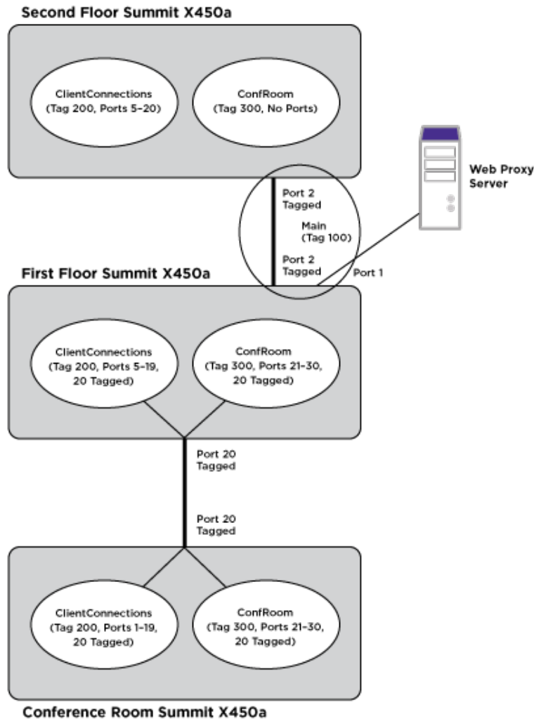
Figure 75: PVLAN Configuration Example 2
