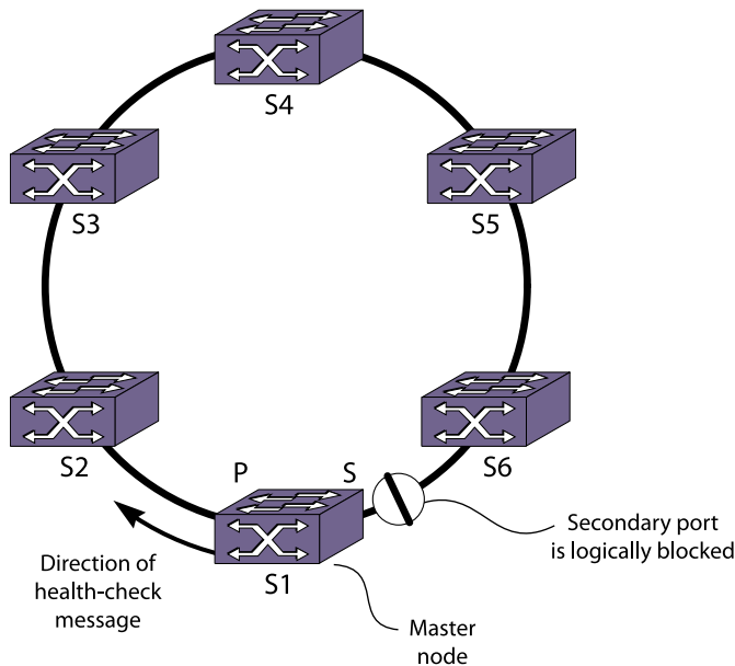
Figure 134: EAPS Operation
