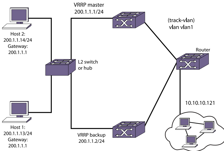
Figure 203: VRRP Tracking
