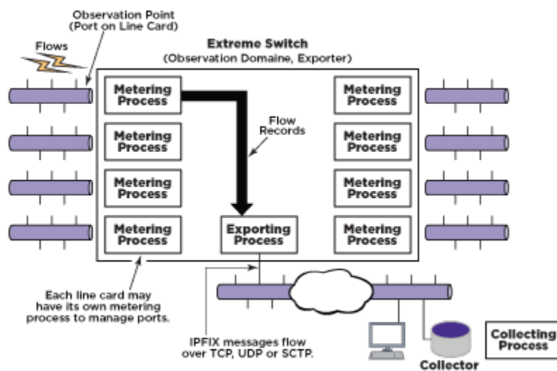
Figure 11: IPFIX Processes
