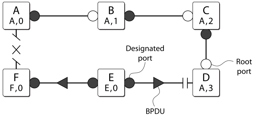
Figure 174: New Root Bridge Selected
