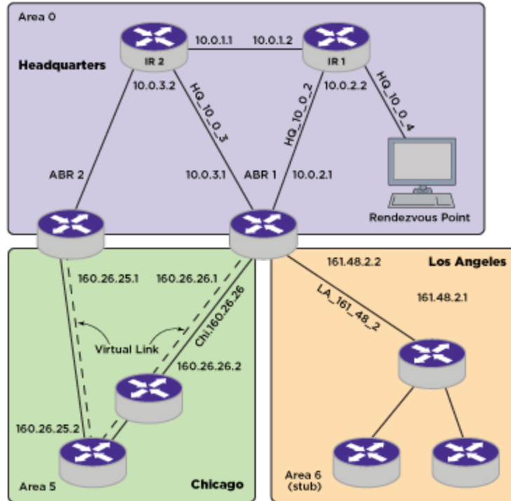
Figure 275: IP Multicast Routing Using PIM-SM Configuration Example
