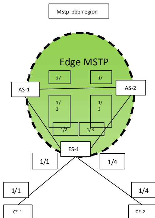
FIGURE 70 Edge MSTP in a PB network
