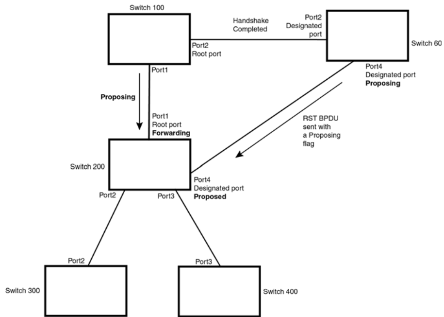
FIGURE 80 New root bridge sending a proposal flag
