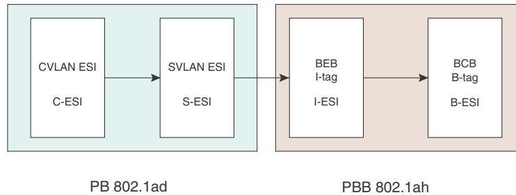
FIGURE 38 Association of ESI and VLAN for different stages
