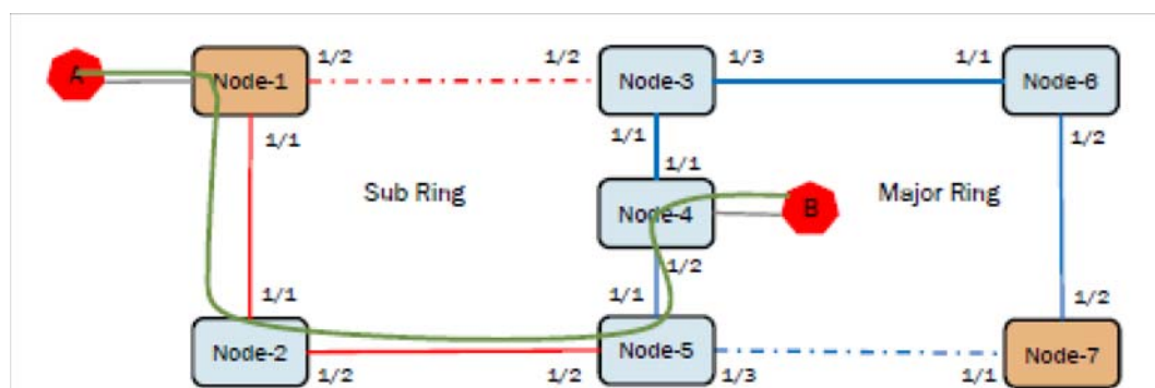
FIGURE 157 RAPS-propagate-tc topology change
