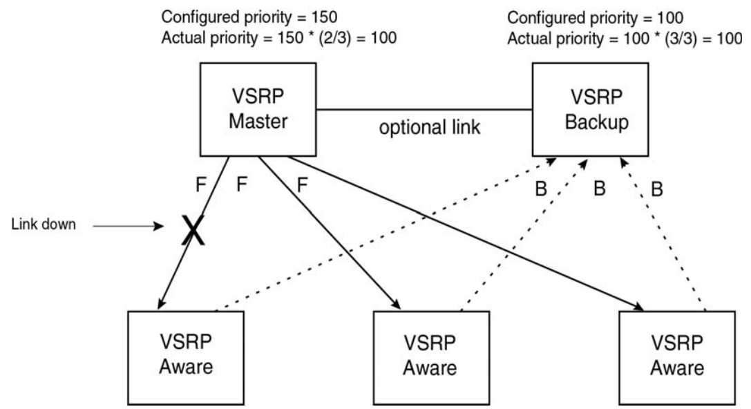
FIGURE 161 VSRP priority bias
