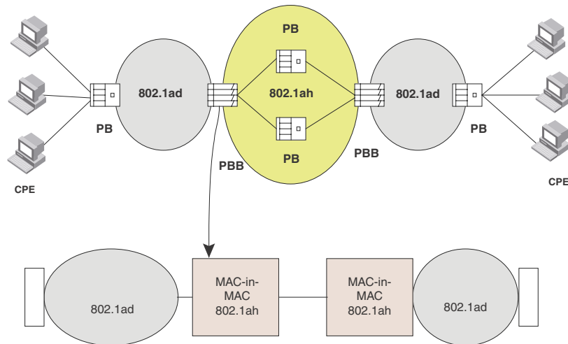
FIGURE 34 IEEE 802.1ah PBB configuration
