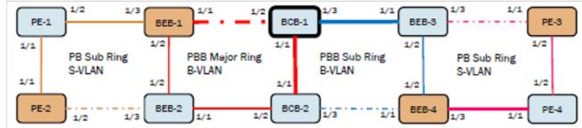
FIGURE 153 PBB Interconnection node (BCB)
