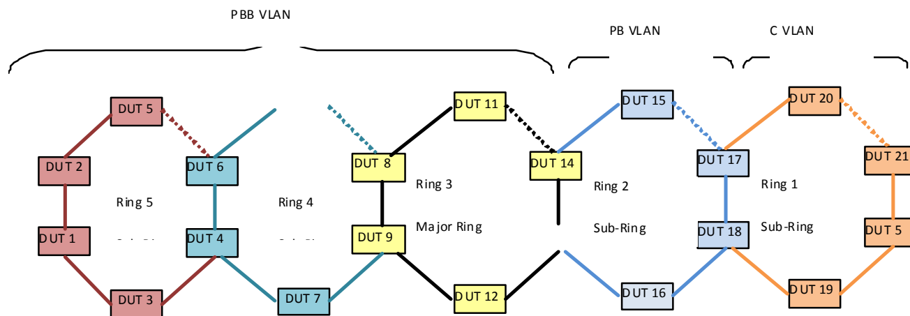
FIGURE 146 ERP configuration over ESI network
