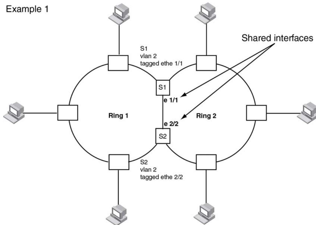
FIGURE 115 Example 1 multiple rings sharing interfaces - phase 2
