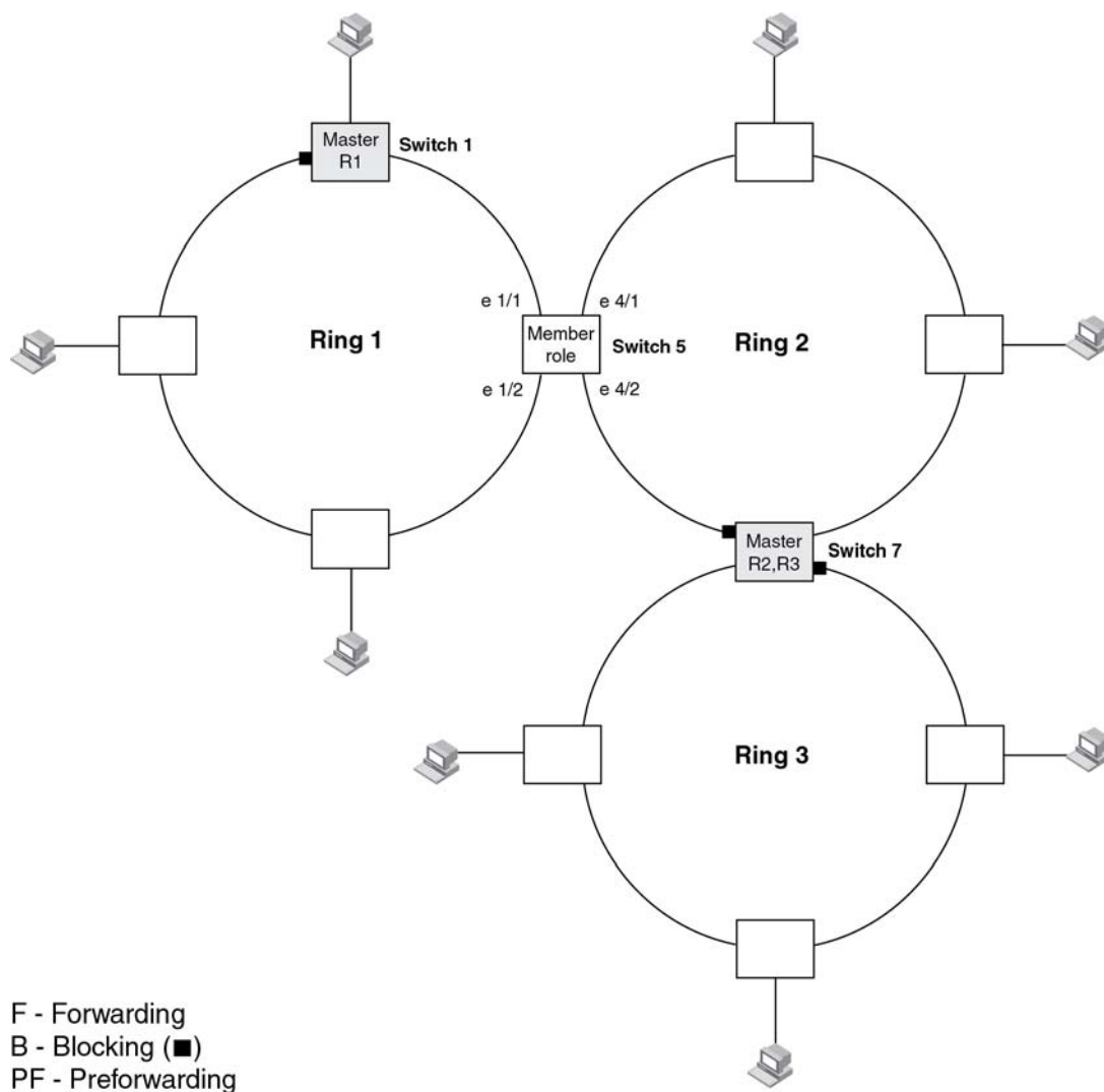
FIGURE 106 MRP – multiple rings, no shared interfaces
