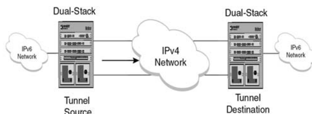
FIGURE 204 Manually configured tunnel
