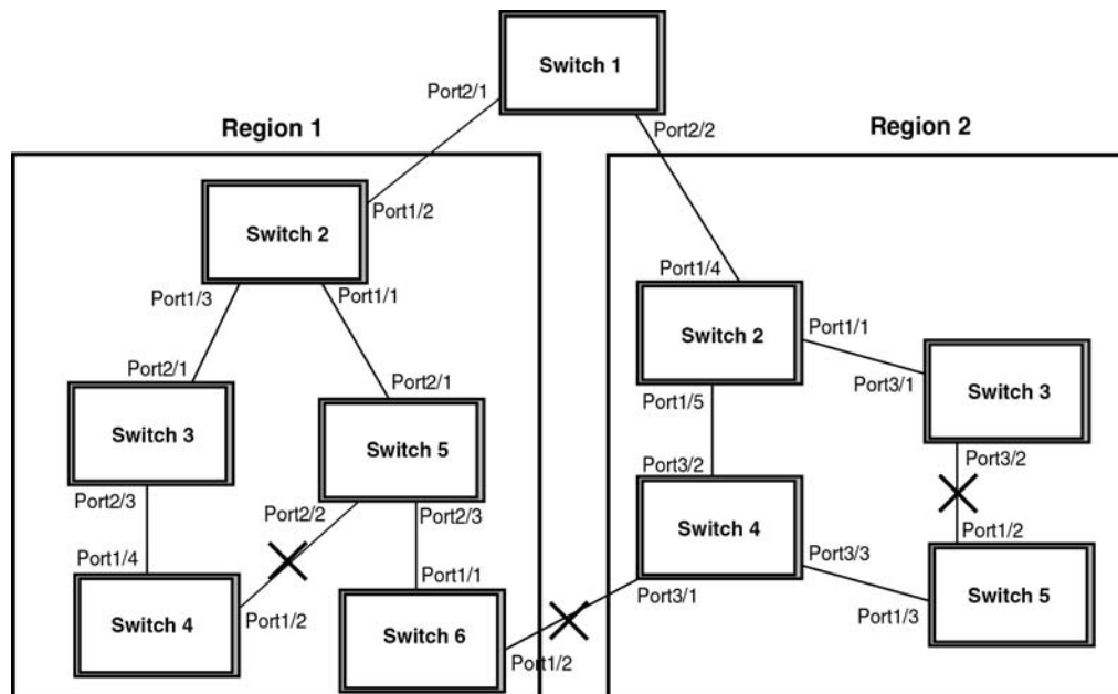
FIGURE 66 MSTP configured network
