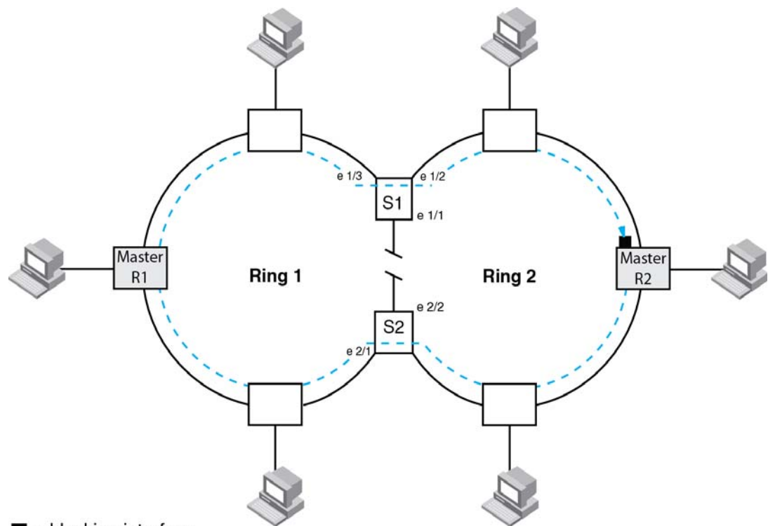
FIGURE 123 Flow of RHP packets when a link for shared interfaces breaks
