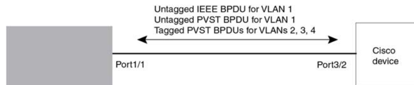
FIGURE 64 Default VLAN 1 for untagged BPDUs
